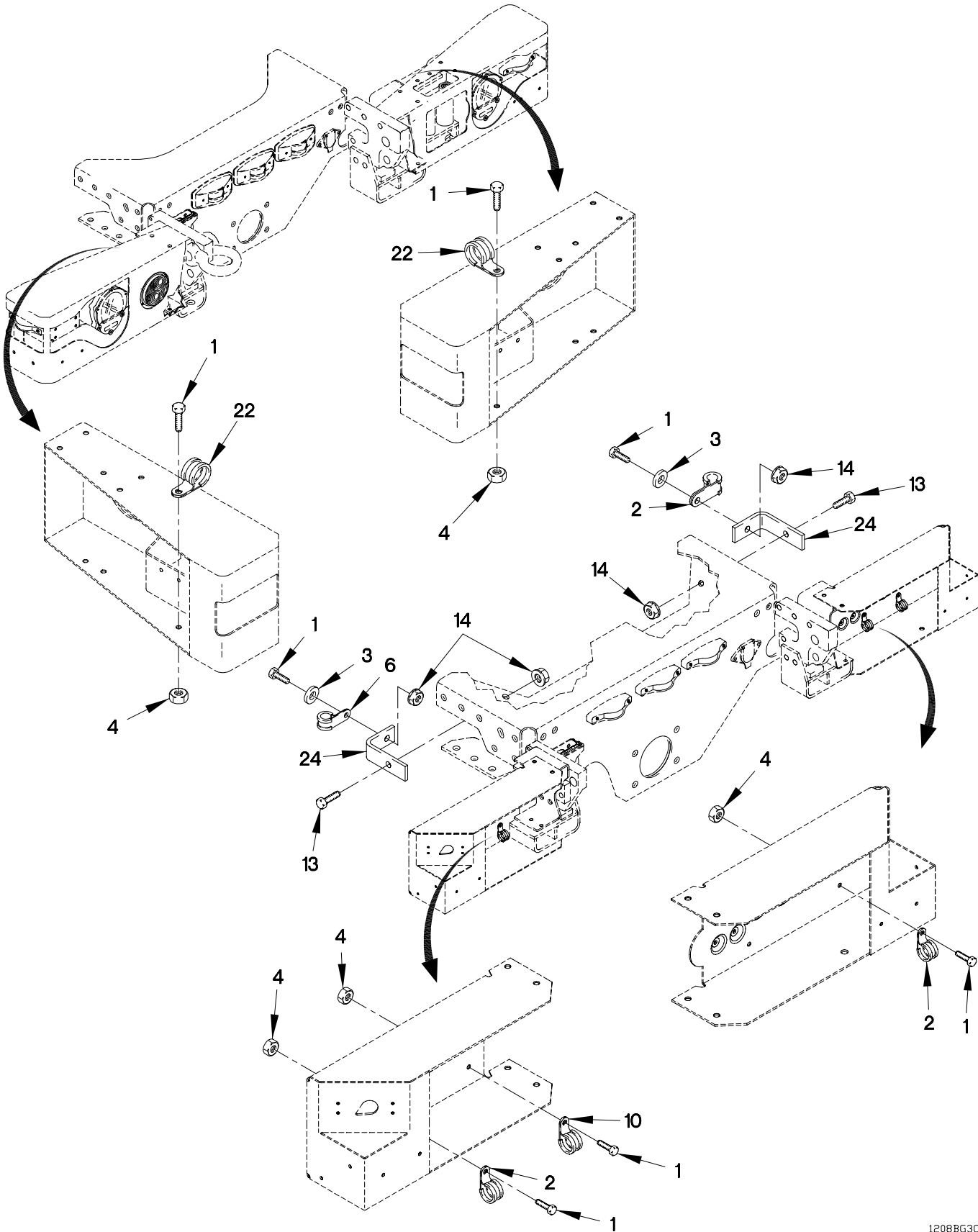
FIGURE 199. M1094 PNEUMATIC HOSE ROUTING LOOP CLAMPS AND BRACKETS (SHEET 3 OF 3)
