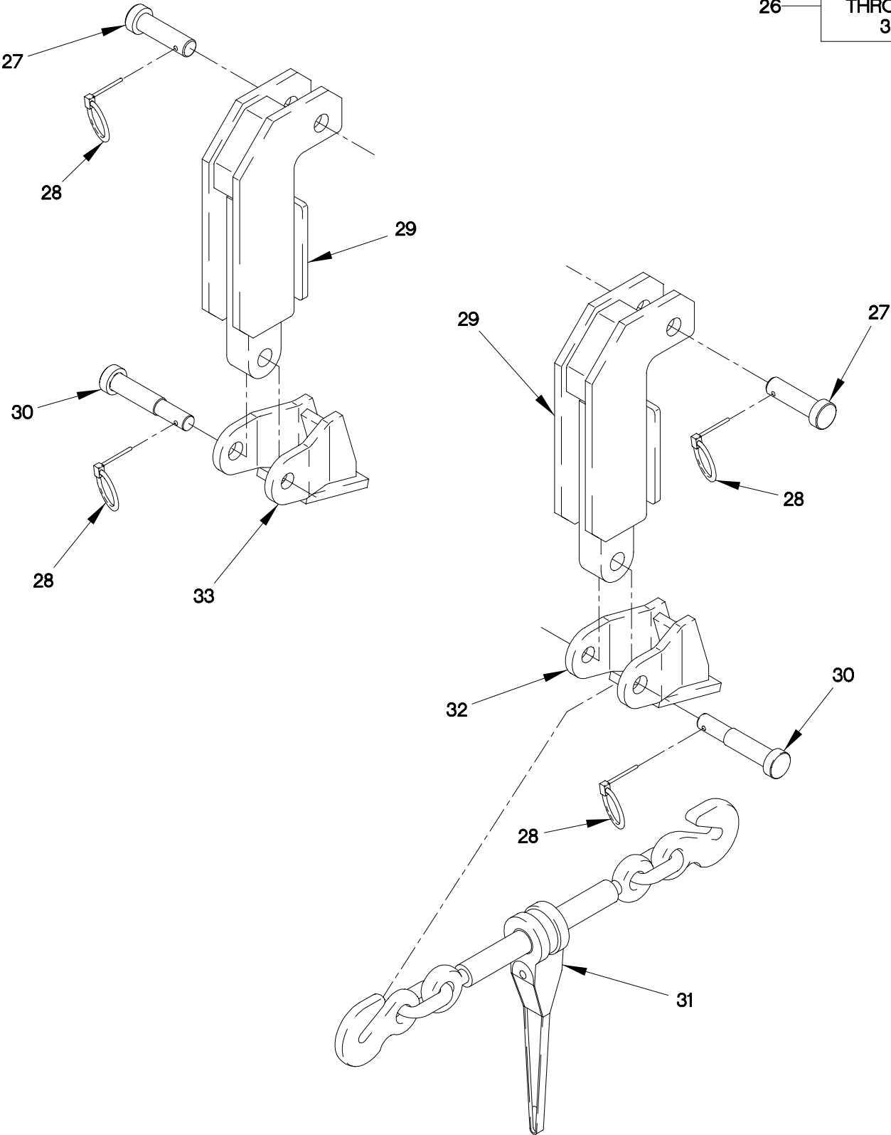
FIGURE 302 M1089 UNDERLIFT CROSSBAR ASSEMBLY AND FRONT TOWING ADAPTER (SHEET 2 OF 2)
