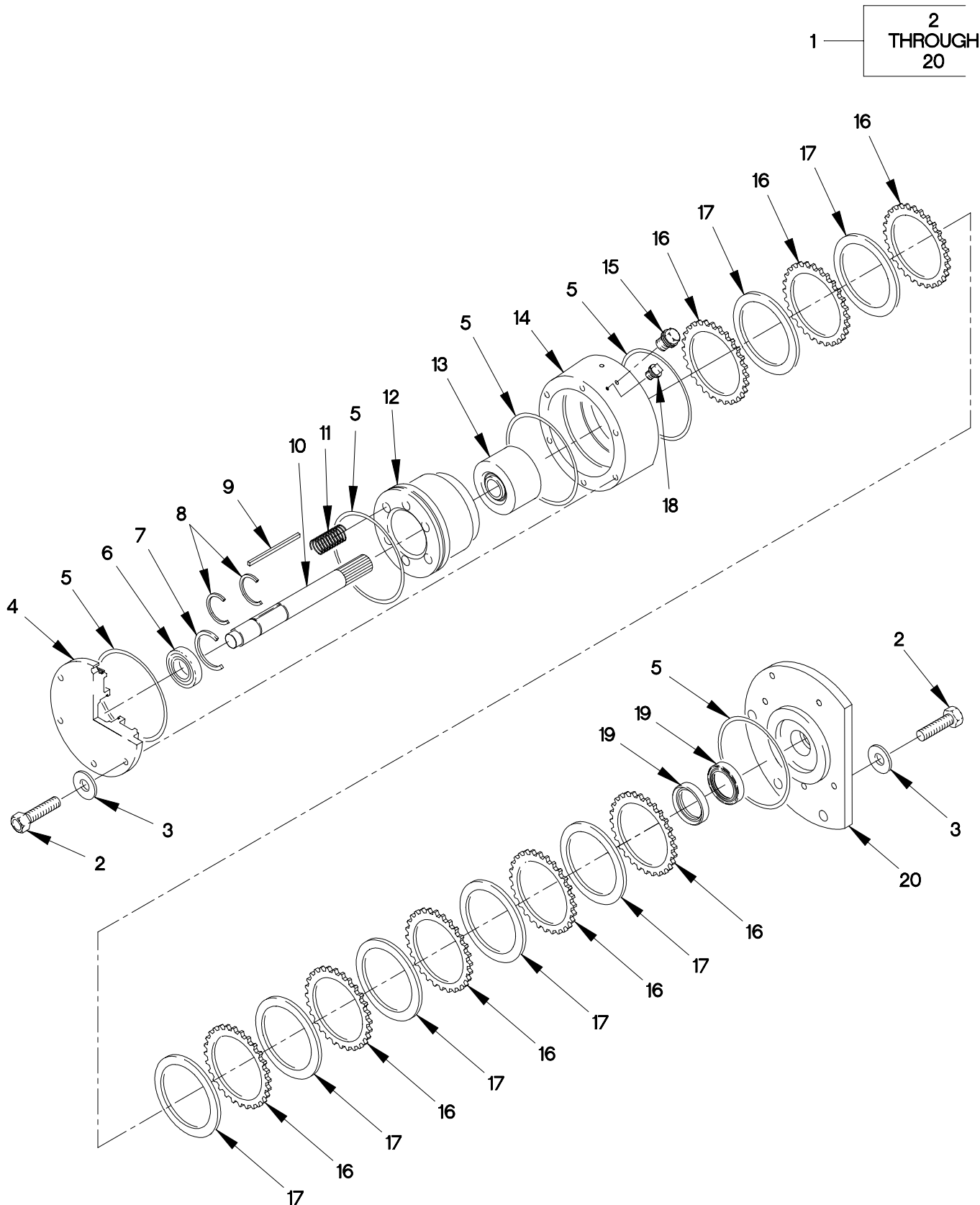
FIGURE 382. M1084 AND M1086 OIL FILLED DISC BRAKE
