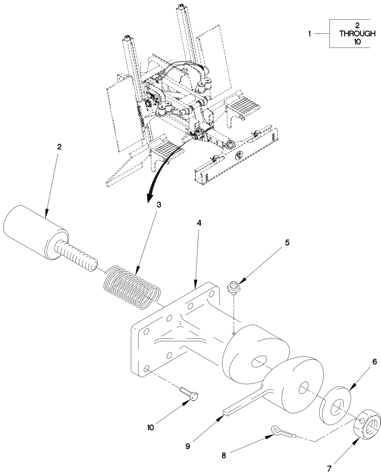
FIGURE 312. M1089 UNDERLIFT CAMLOCK ASSEMBLY
