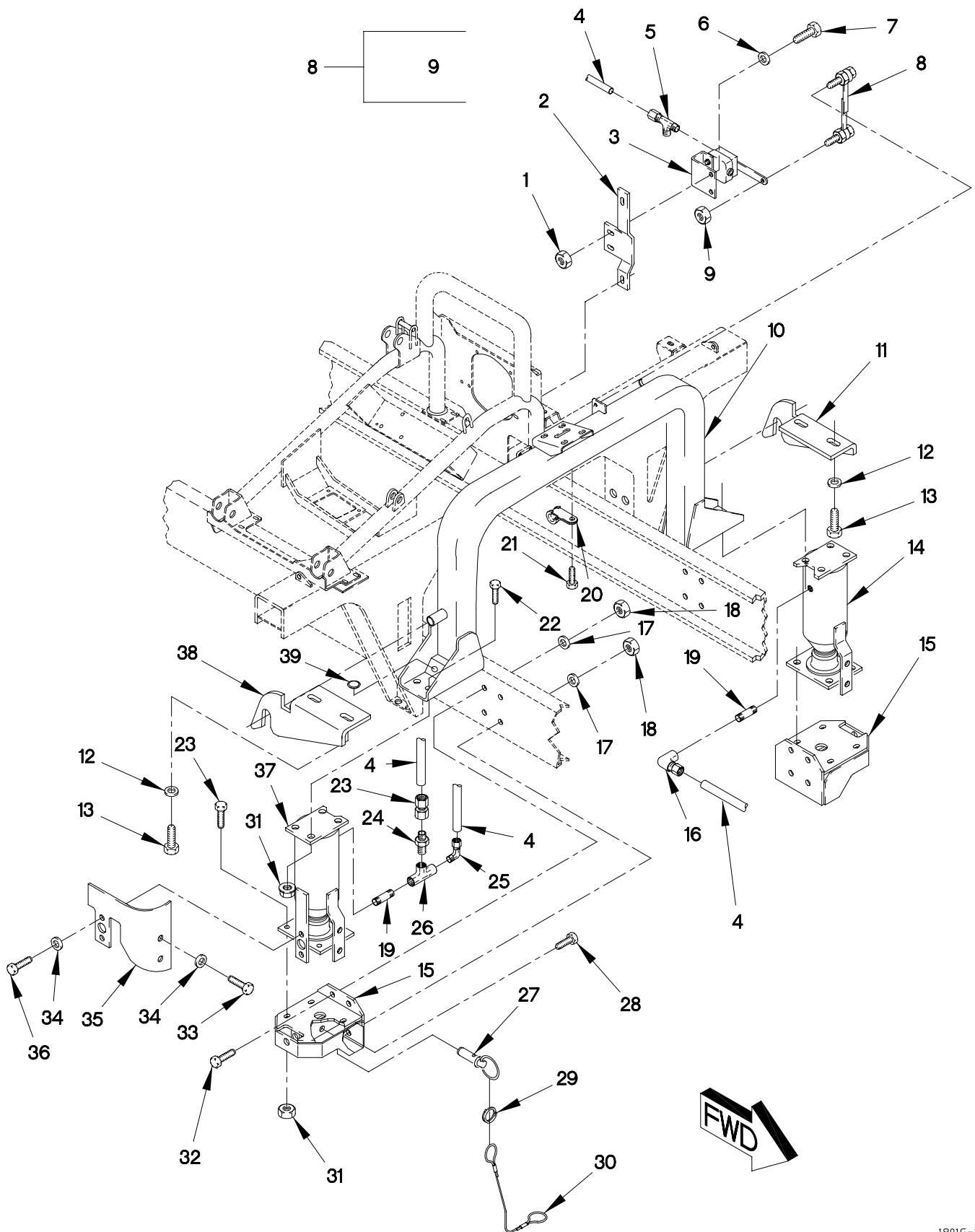
FIGURE 254. REAR CAB SUPPORT, LEVELING VALVE, LATCH, AIR SPRING, HOSES AND FITTINGS (SHEET 1 OF 2)
