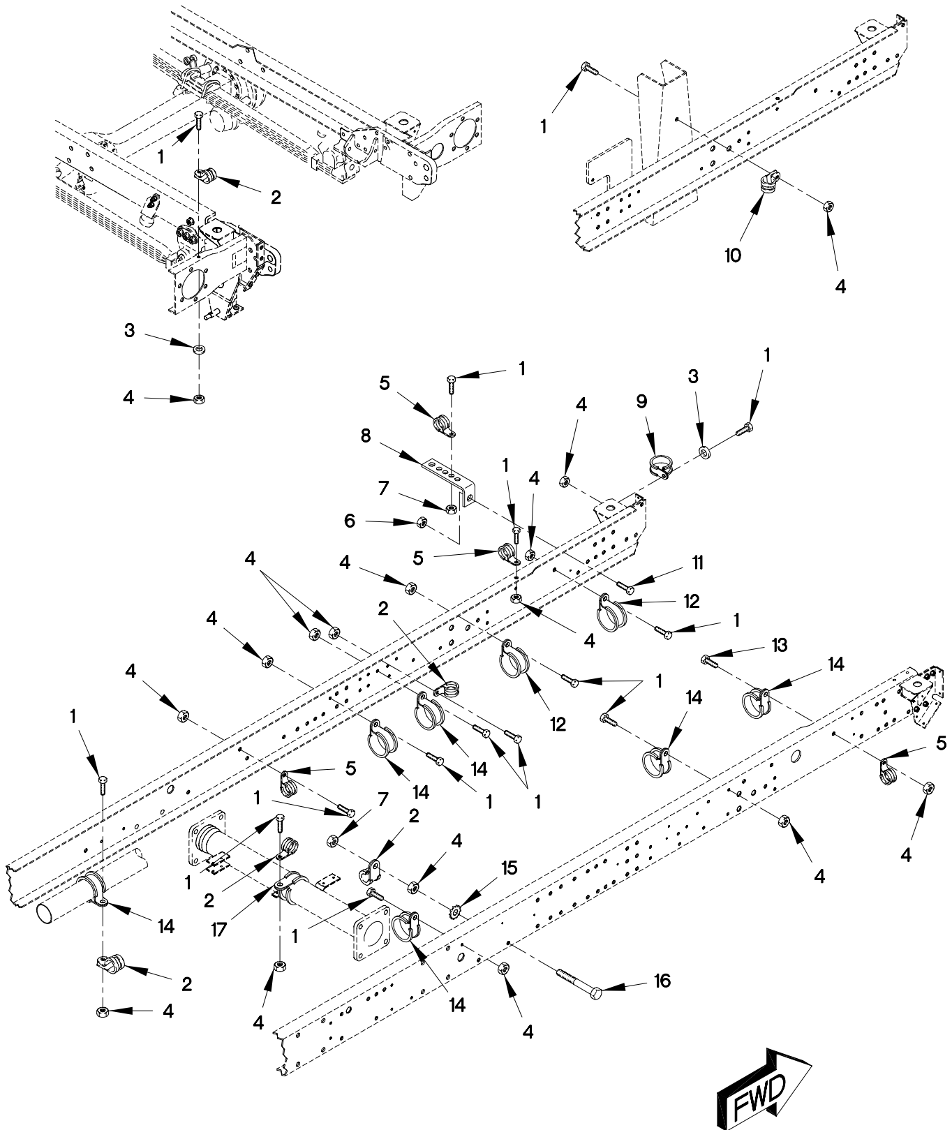
FIGURE 193. M1085 AND M1096 PNEUMATIC HOSE ROUTING LOOP CLAMPS AND BRACKETS (SHEET 1 OF 3)
