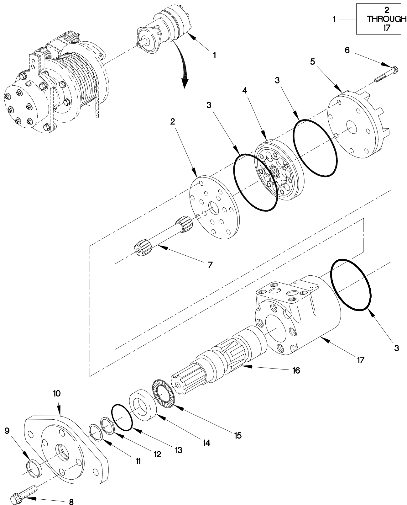
FIGURE 326. M1089 HOIST HYDRAULIC MOTOR
