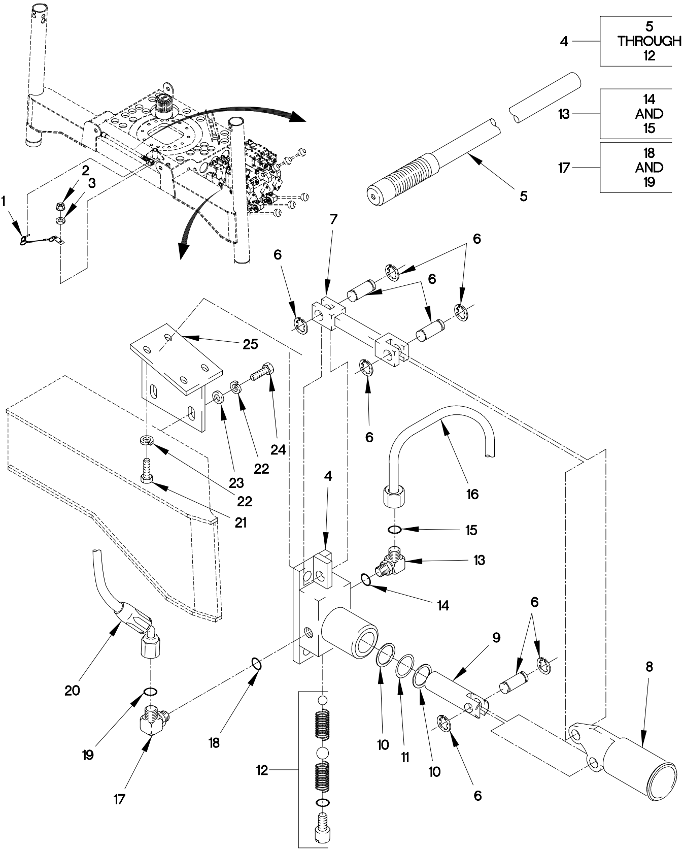
FIGURE 401. M1084 AND M1086 HAND PUMP ASSEMBLY
