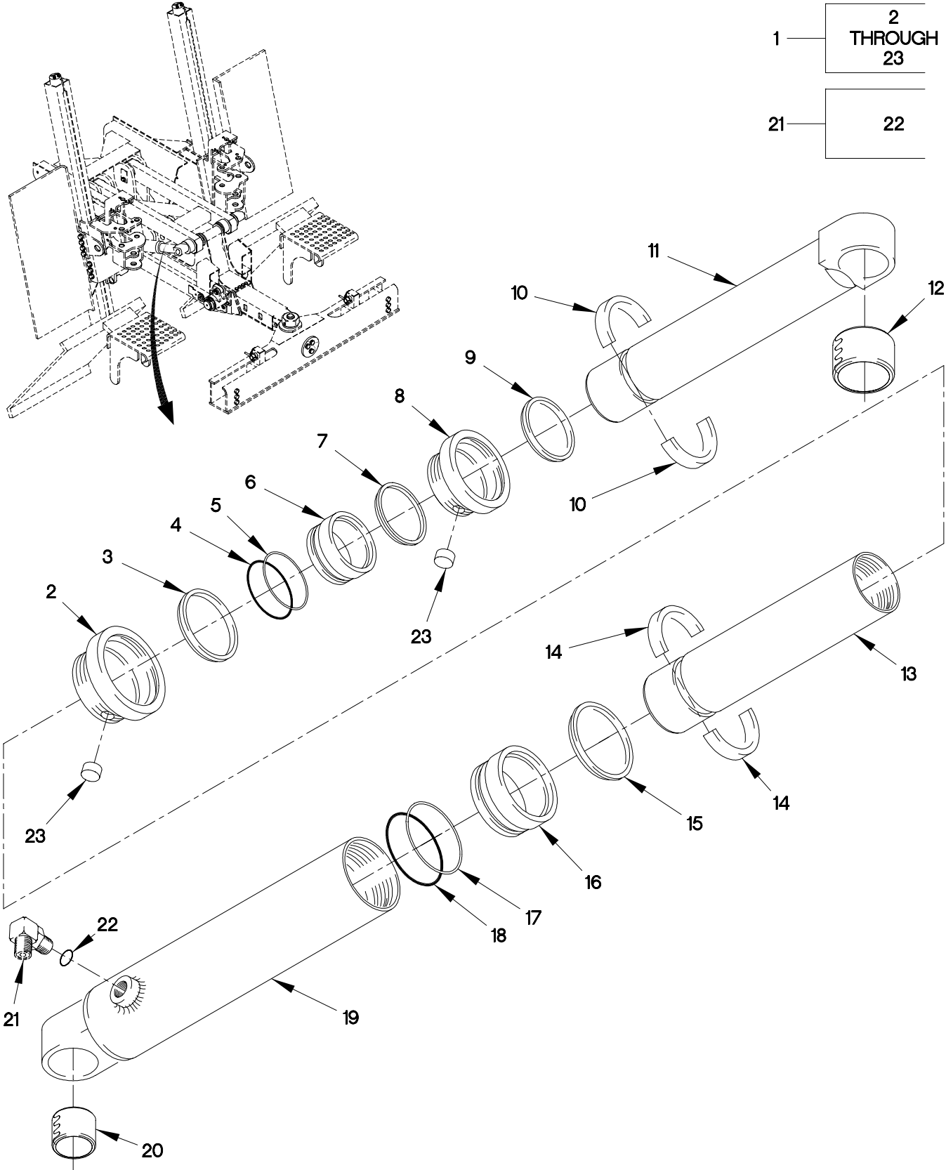
FIGURE 311. M1089 UNDERLIFT TELESCOPE LIFT CYLINDER ASSEMBLY
