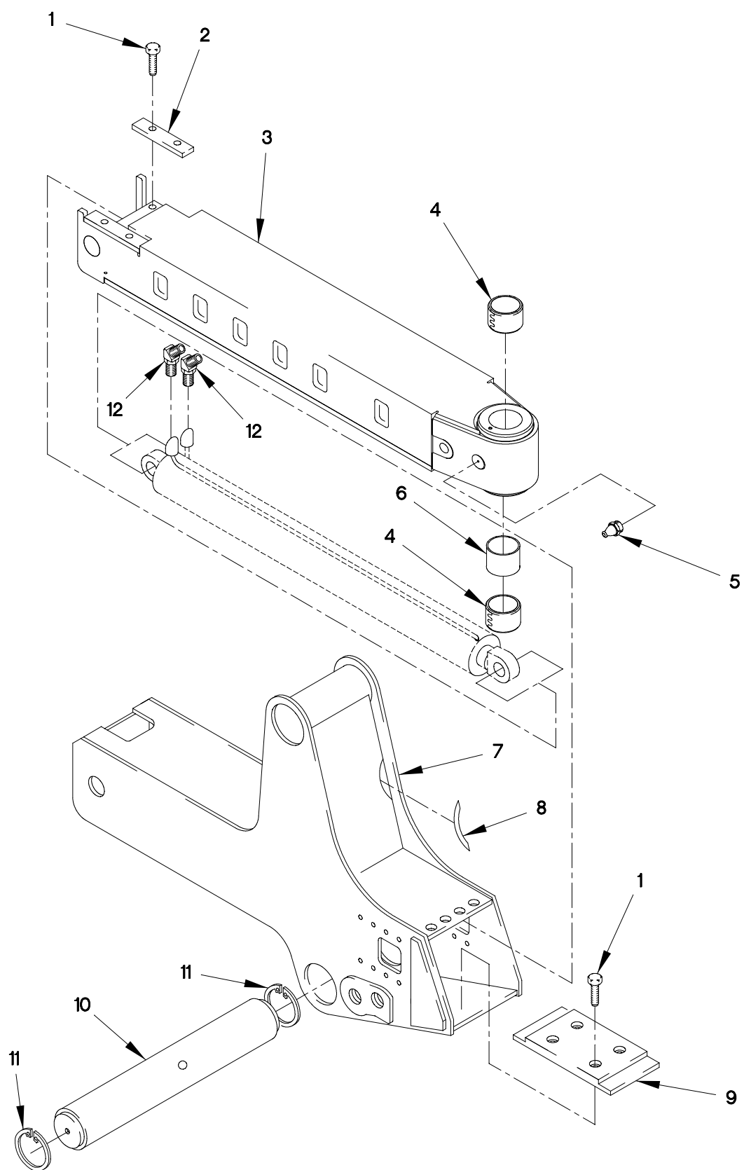
FIGURE 308. M1089 UNDERLIFT FOLDING BOOM FRAME
