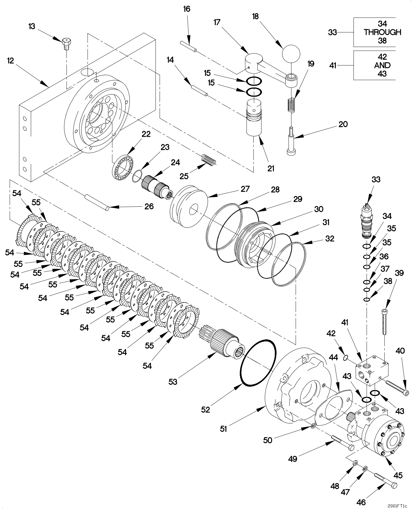
FIGURE 299. 15K SELF RECOVERY WINCH ASSEMBLY (SHEET 2 OF 4)
