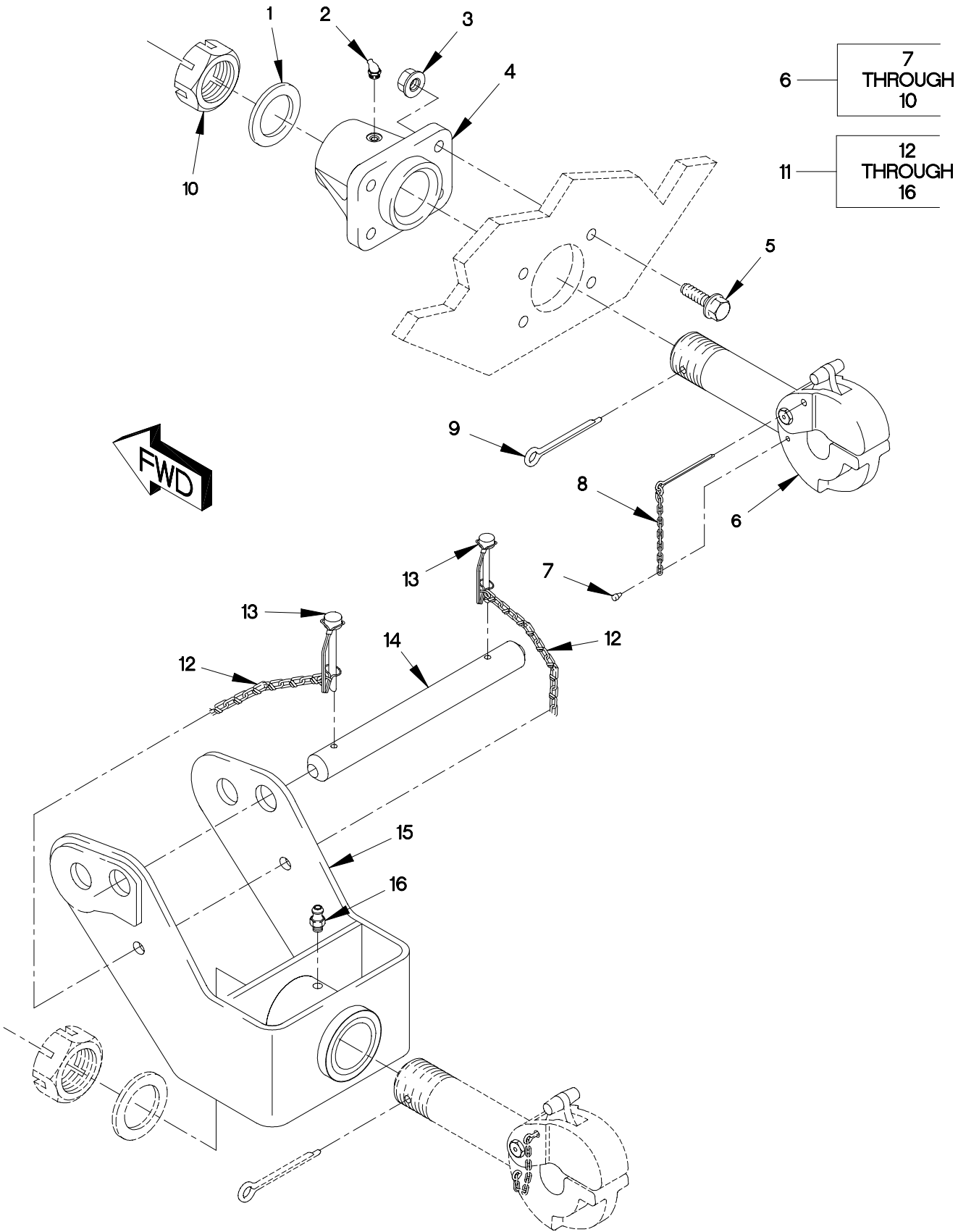
FIGURE 235. PINTLE HOOK
