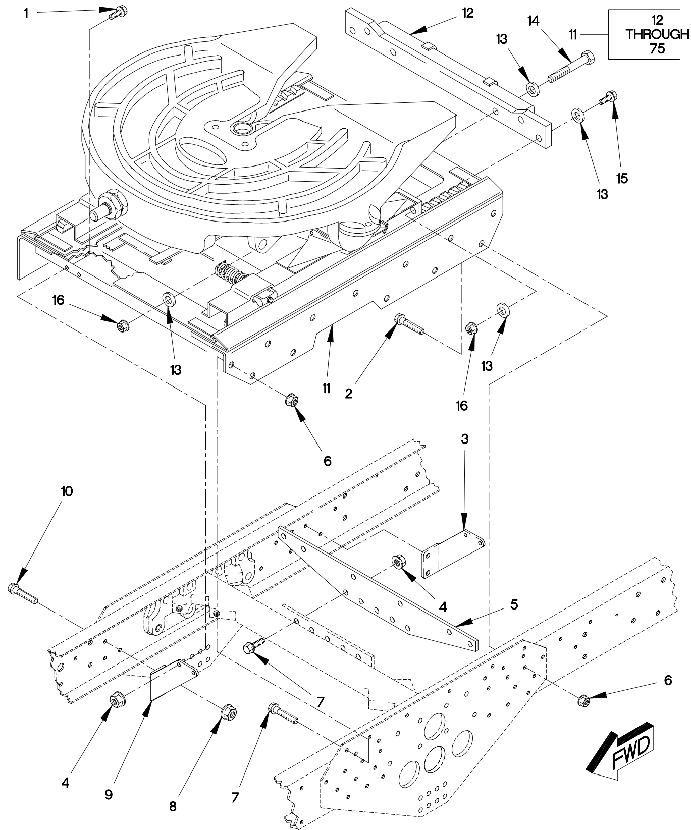
FIGURE 237. M1088 FIFTH WHEEL ASSEMBLY (SHEET 1 OF 4)
