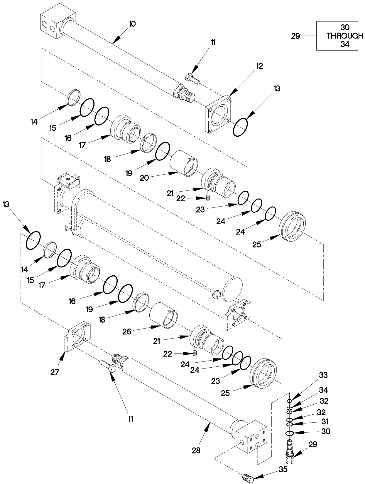
FIGURE 331. M1089 BOOM TELESCOPIC CYLINDER ASSEMBLY (SHEET 2 OF 2)
