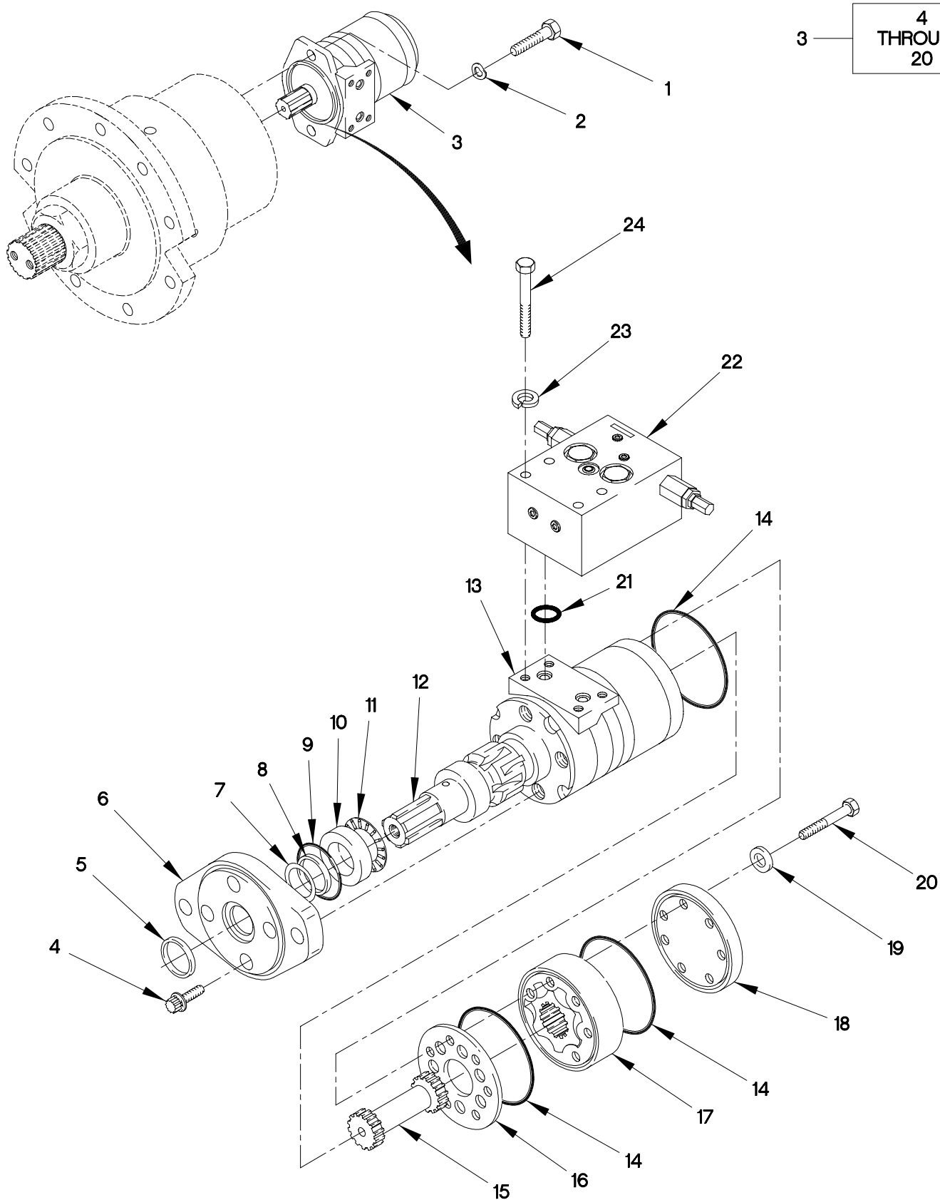
FIGURE 334. M1089 SWING DRIVE HYDRAULIC MOTOR AND CROSS RELIEF VALVE
