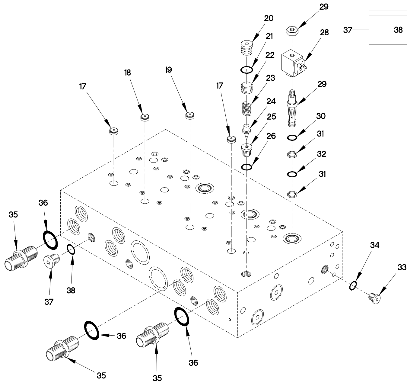
FIGURE 356. M1089 EIGHT BANK SWING CONTROL VALVE MANIFOLD ASSEMBLY AND FITTINGS (SHEET 2 OF 2)
