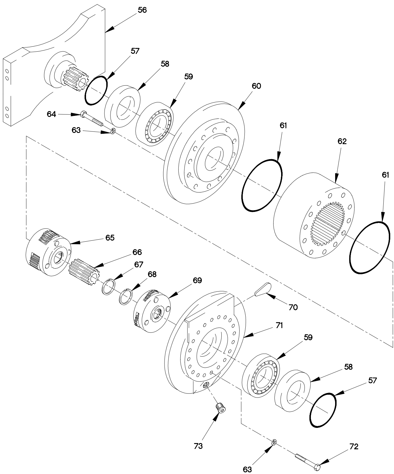
FIGURE 299. 15K SELF RECOVERY WINCH ASSEMBLY (SHEET 3 OF 4)
