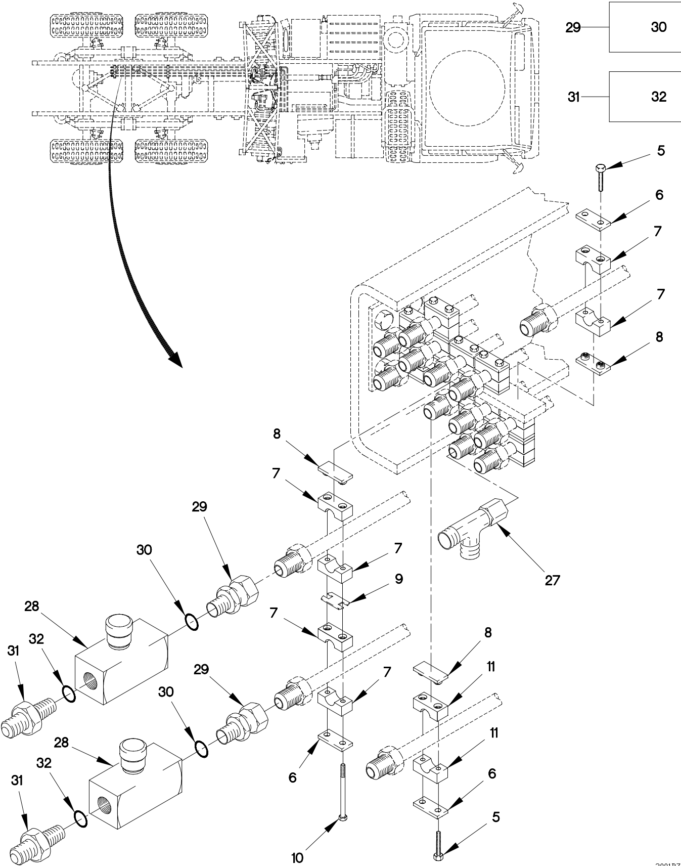
FIGURE 357. M1089 HYDRAULIC HOSES, TUBES AND FITTINGS (SHEET 4 OF 5)
