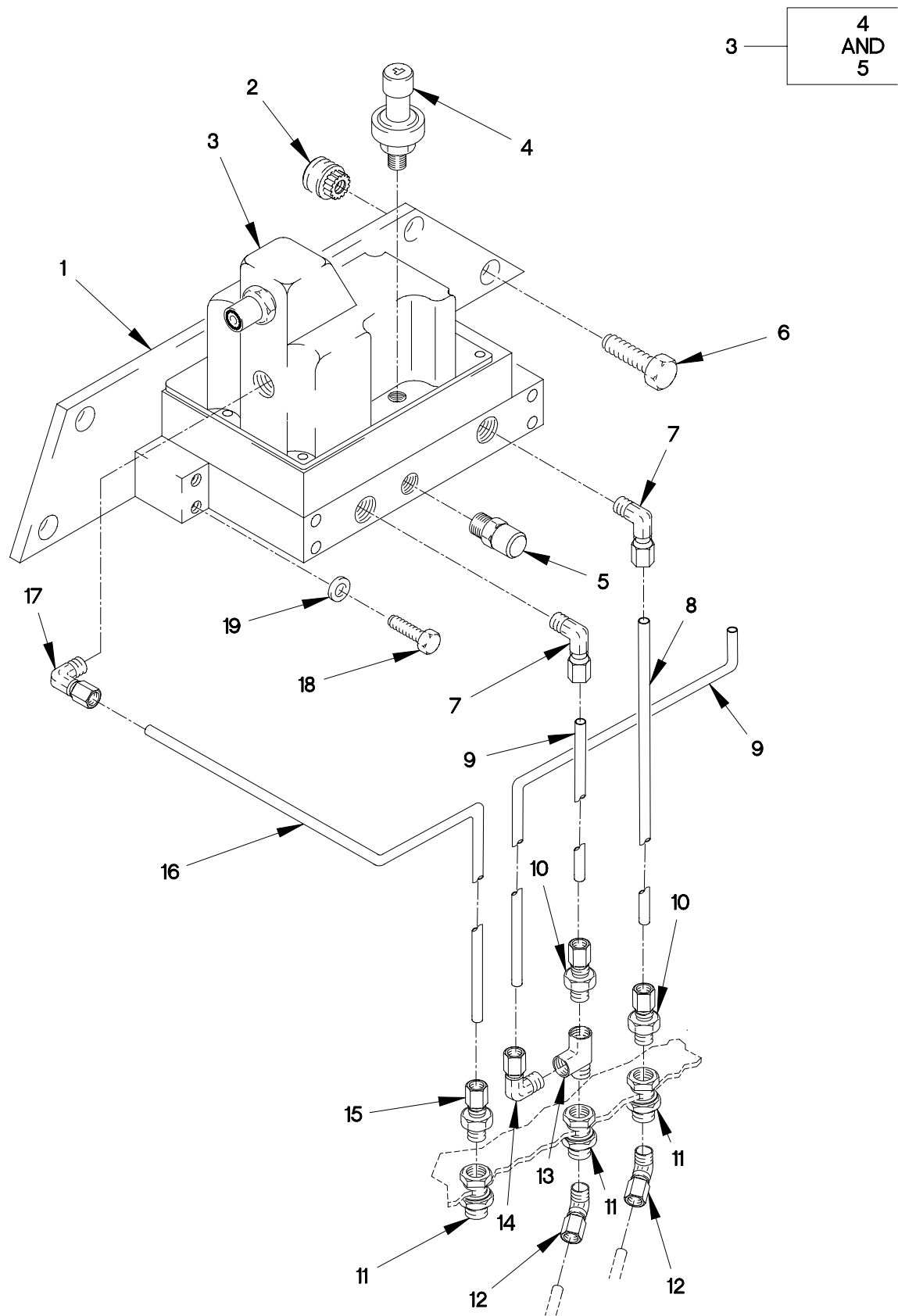
FIGURE 204. MANIFOLD VALVE, HOSES AND FITTINGS
