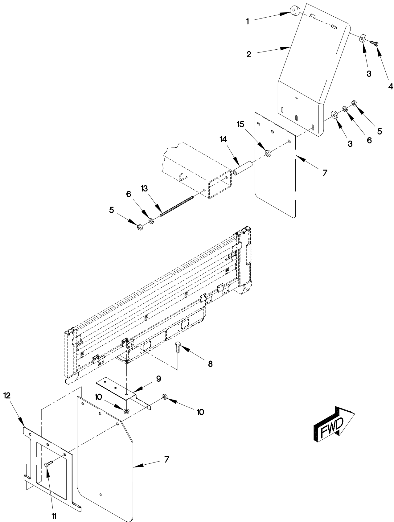
FIGURE 260. M1084 REAR FENDERS AND SPLASH GUARDS
