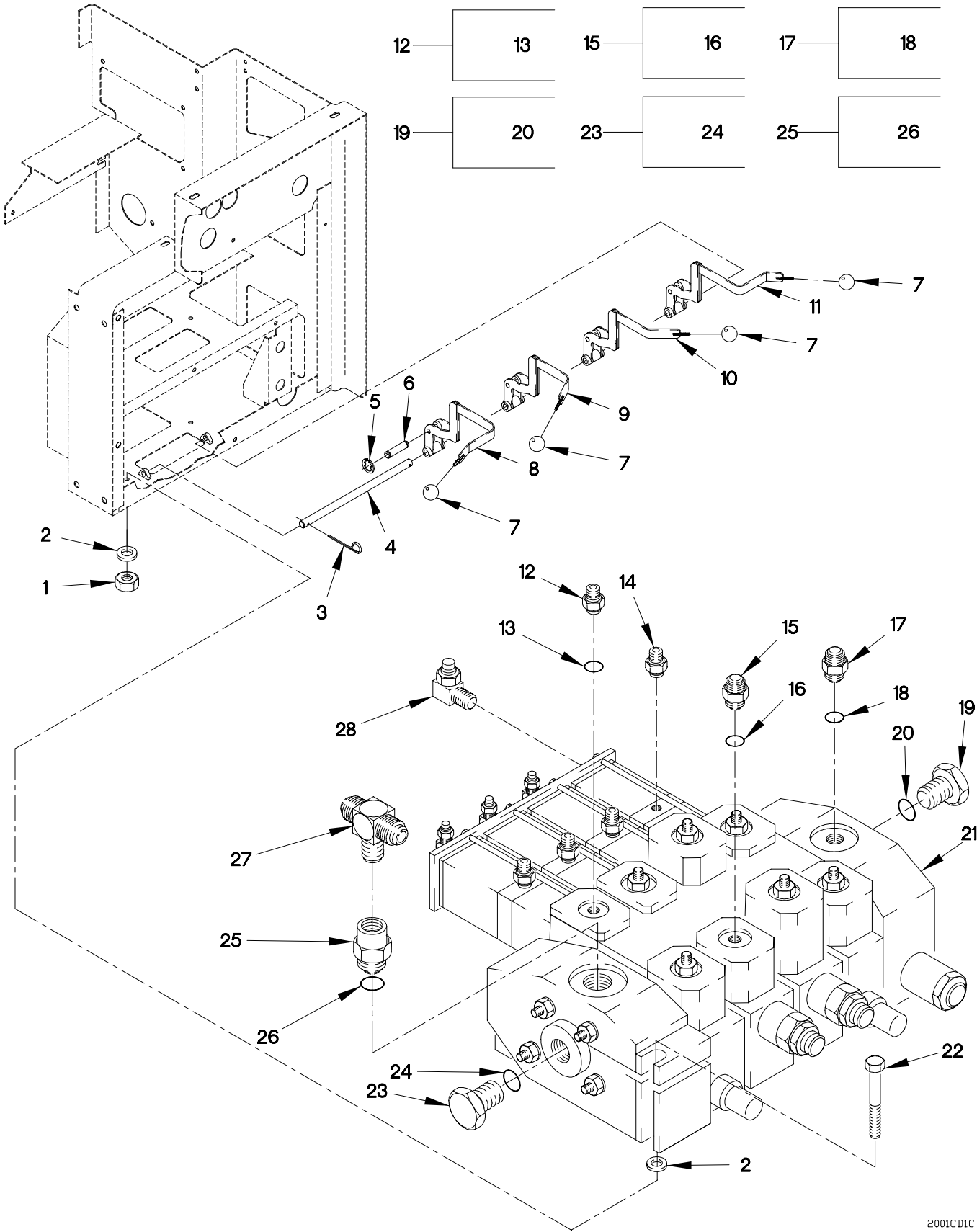
FIGURE 366. M1089 LOWER CONTROL VALVE ASSEMBLY AND HANDLES
