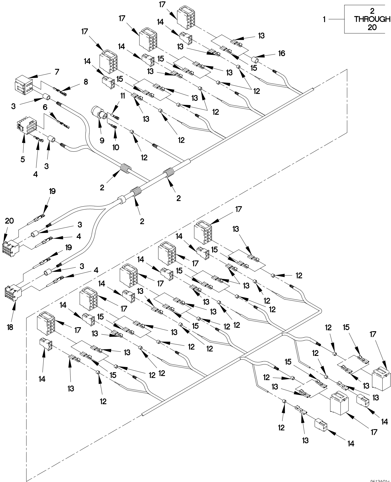
FIGURE 121. AUXILLARY PANEL CABLE ASSEMBLY
