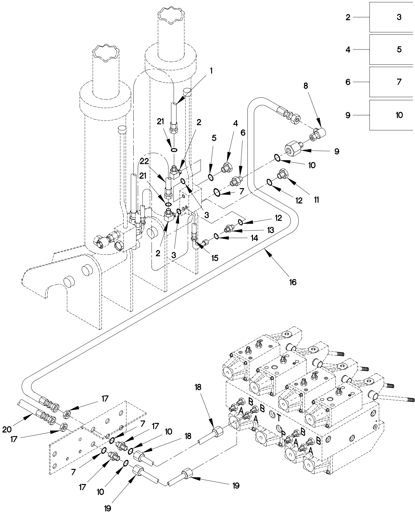
FIGURE 340. M1089 HYDRAULIC LIFT HOSES AND FITTINGS
