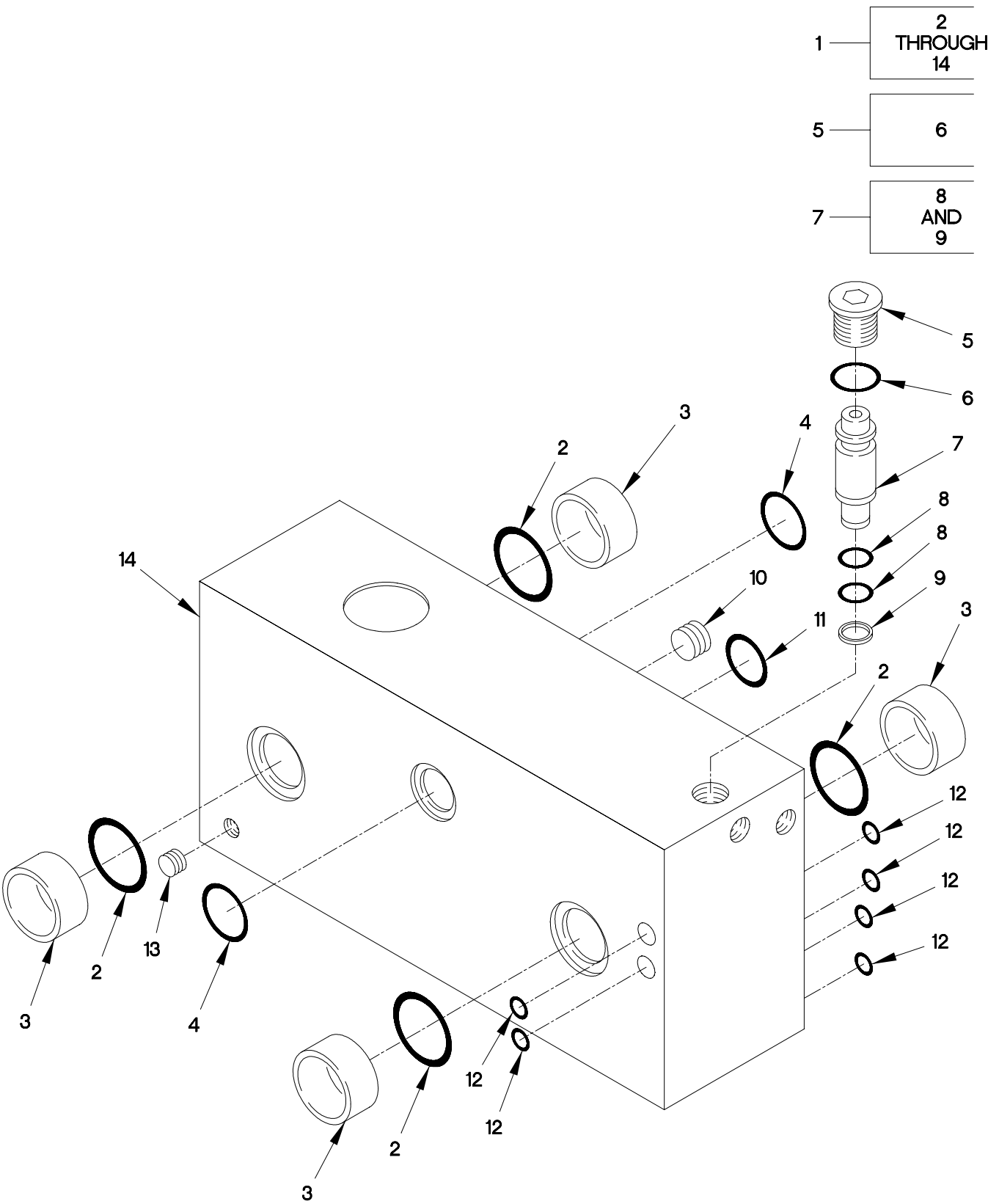
FIGURE 409. M1084 AND M1086 FOUR WAY CENTER MANIFOLD
