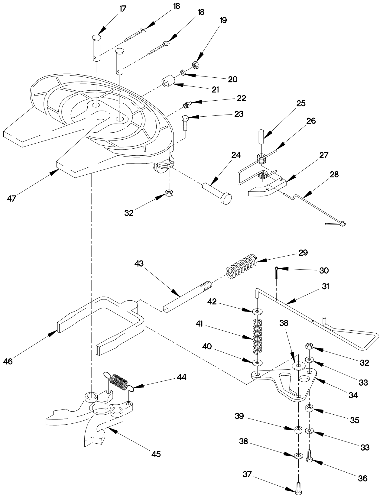
FIGURE 237. M1088 FIFTH WHEEL ASSEMBLY (SHEET 2 OF 4)
