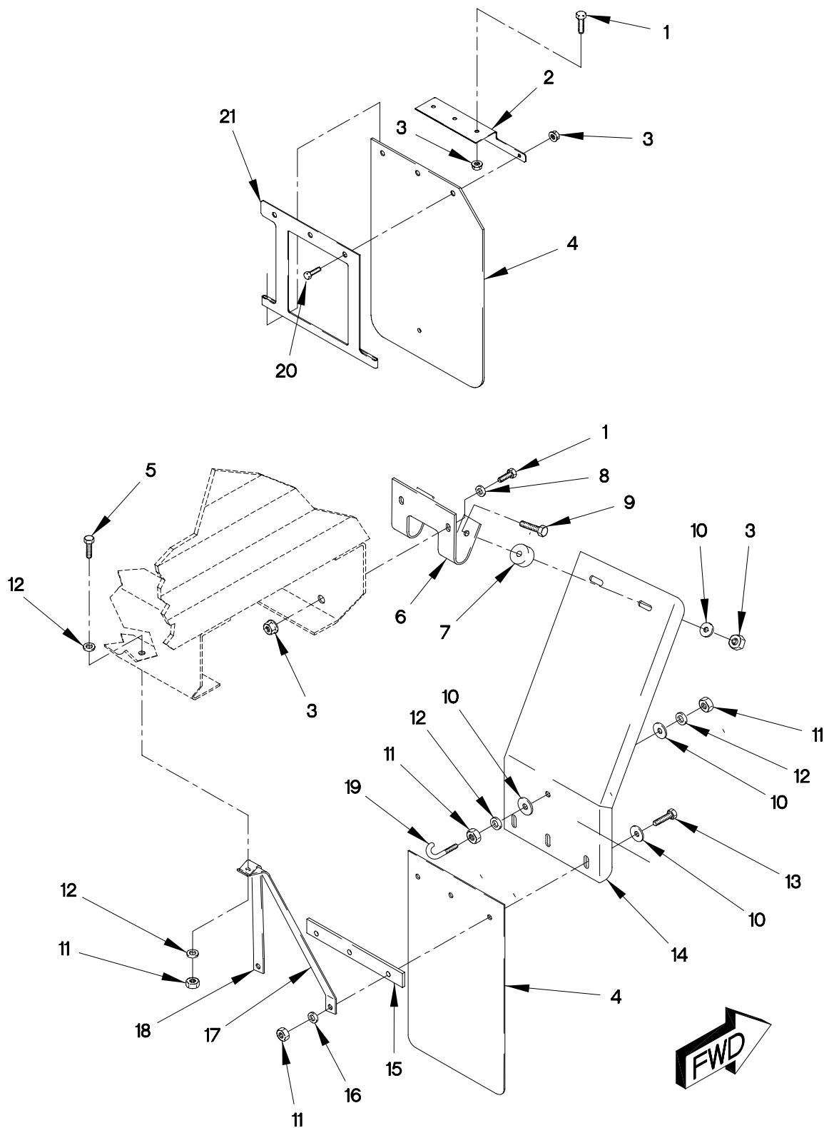
FIGURE 261. M1085 REAR FENDERS AND SPLASH GUARDS
