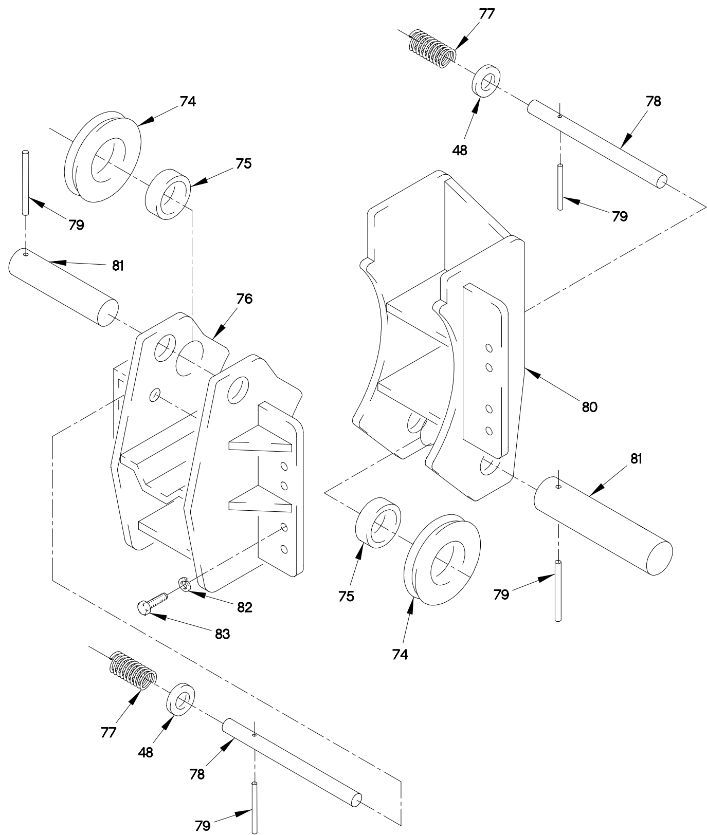
FIGURE 299. 15K SELF RECOVERY WINCH ASSEMBLY (SHEET 4 OF 4)
