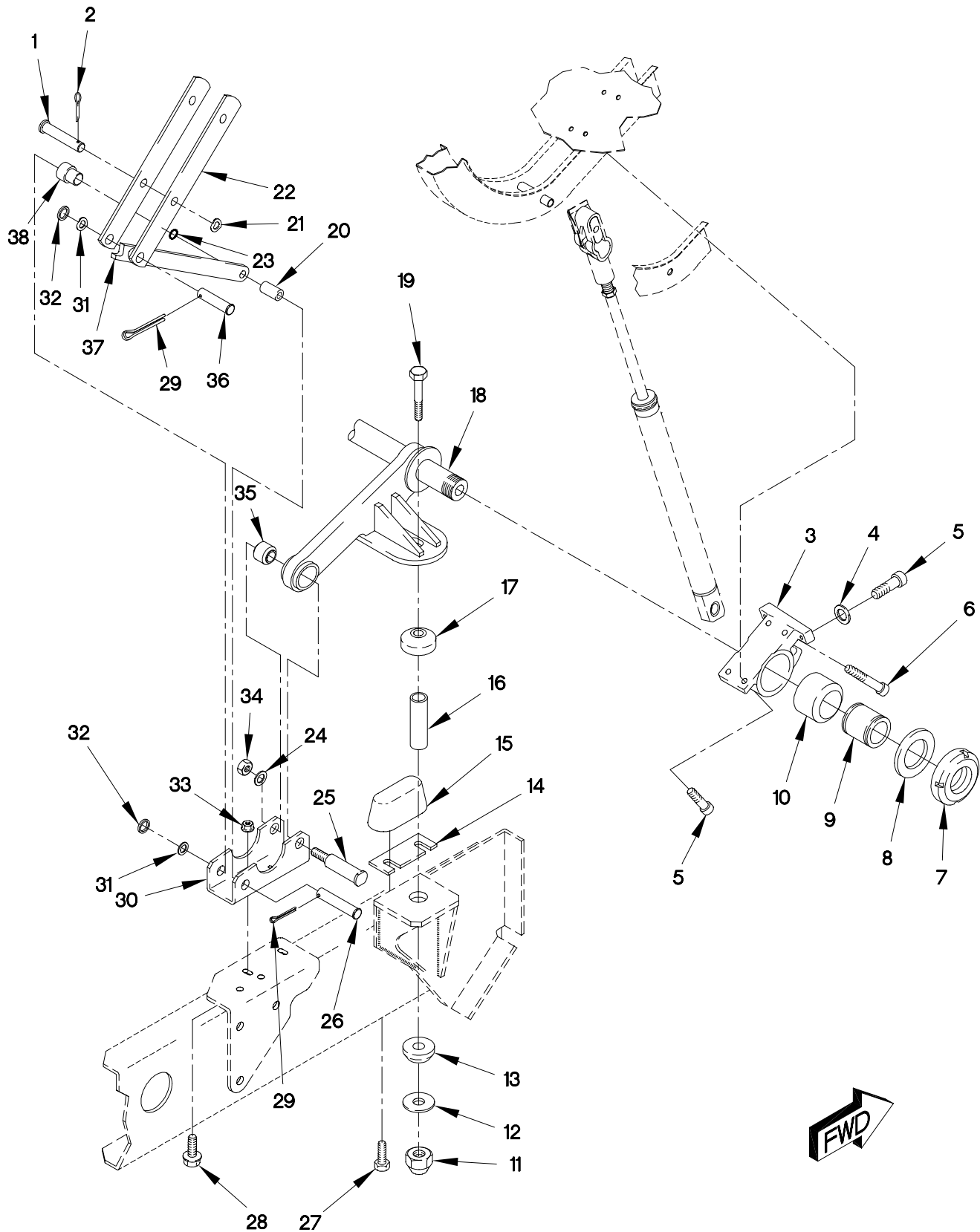
FIGURE 253. FRONT CAB SUPPORTS
