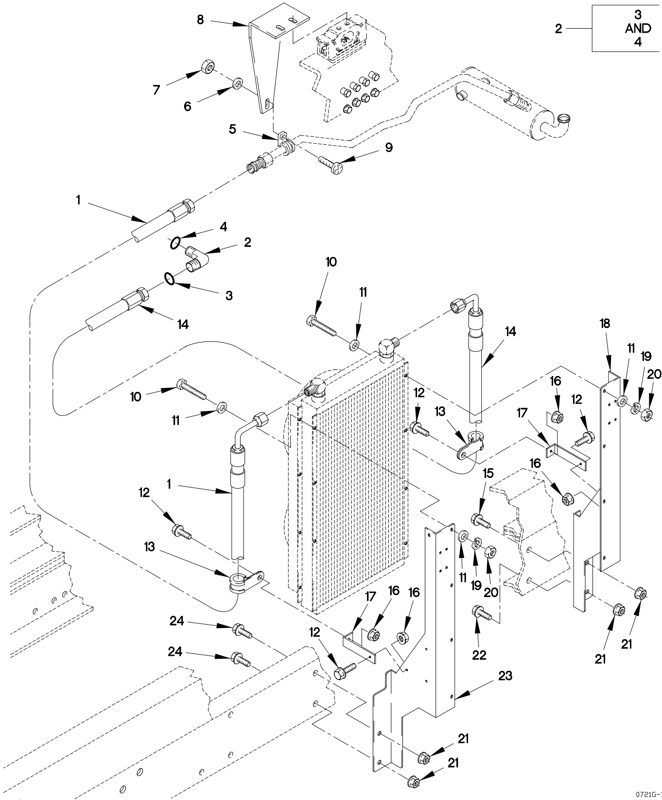
FIGURE 148. M1088 AND M1089 TRANSMISSION AUXILLIARY OIL COOLER (SHEET 1 OF 2)
