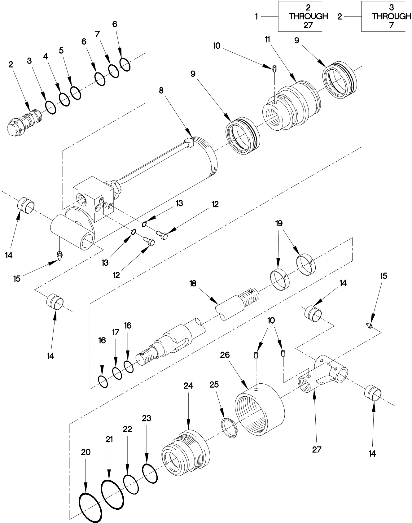
FIGURE 385. M1084 AND M1086 ERECTION CYLINDER ASSEMBLY
