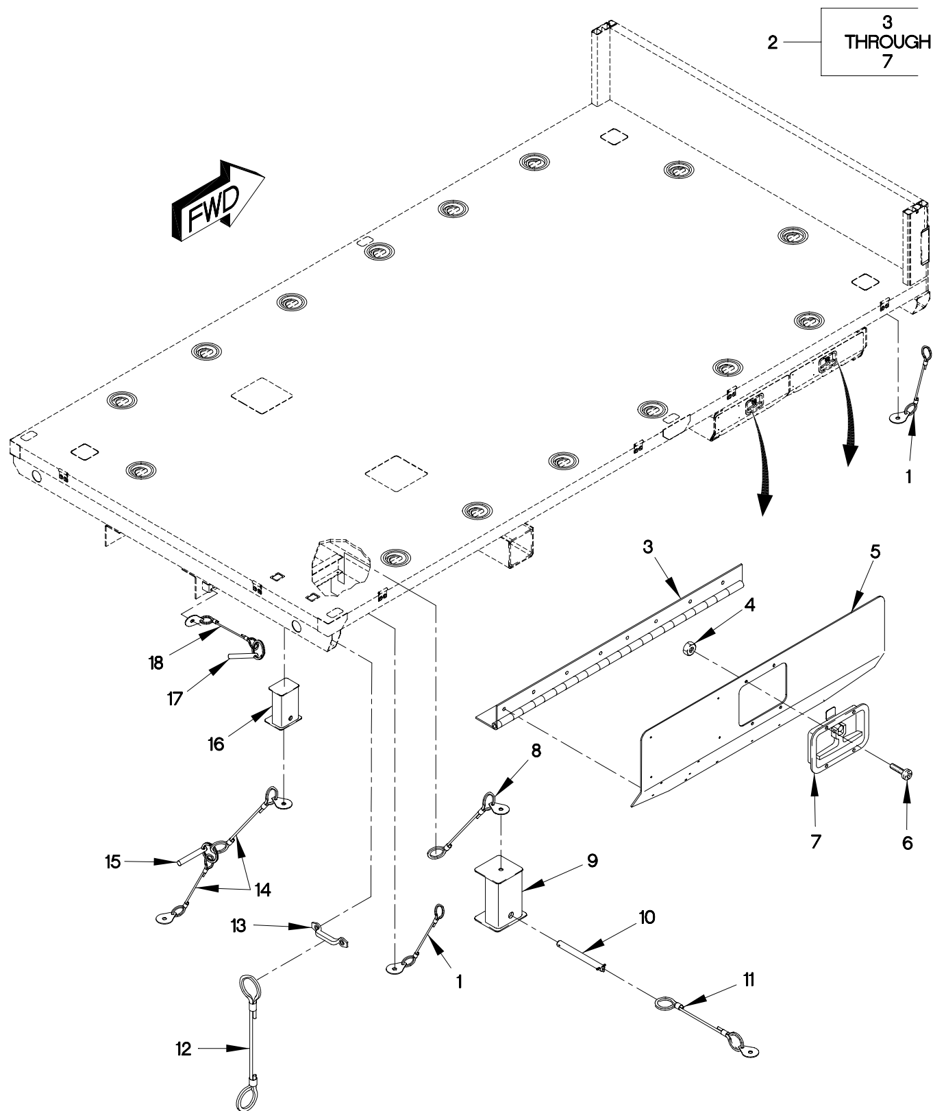
FIGURE 280. M1083, M1084 AND M1093 CARGO BED DOORS, LATCHES AND FITTINGS
