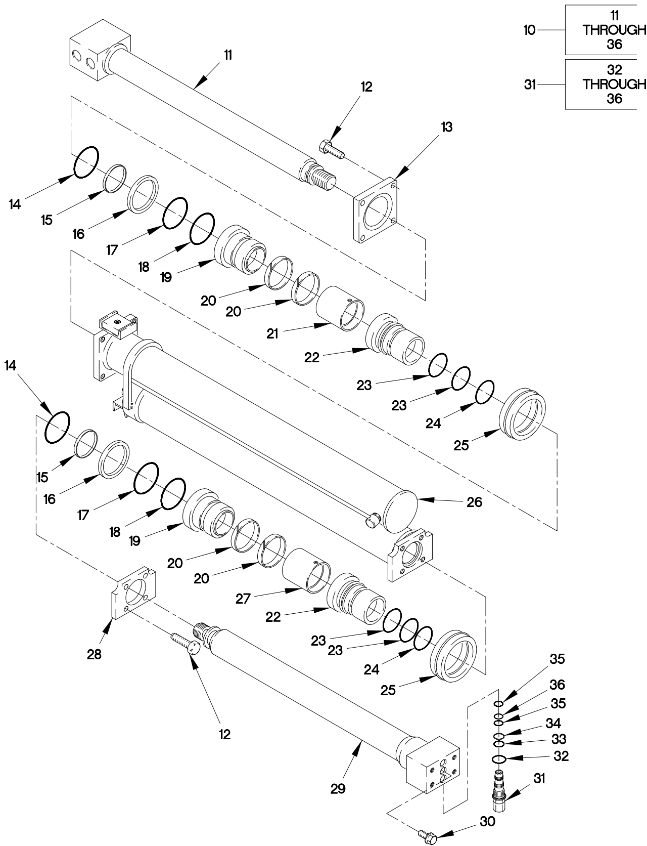
FIGURE 389. M1084 AND M1086 TELESCOPE CYLINDER ASSEMBLY (SHEET 2 OF 2)
