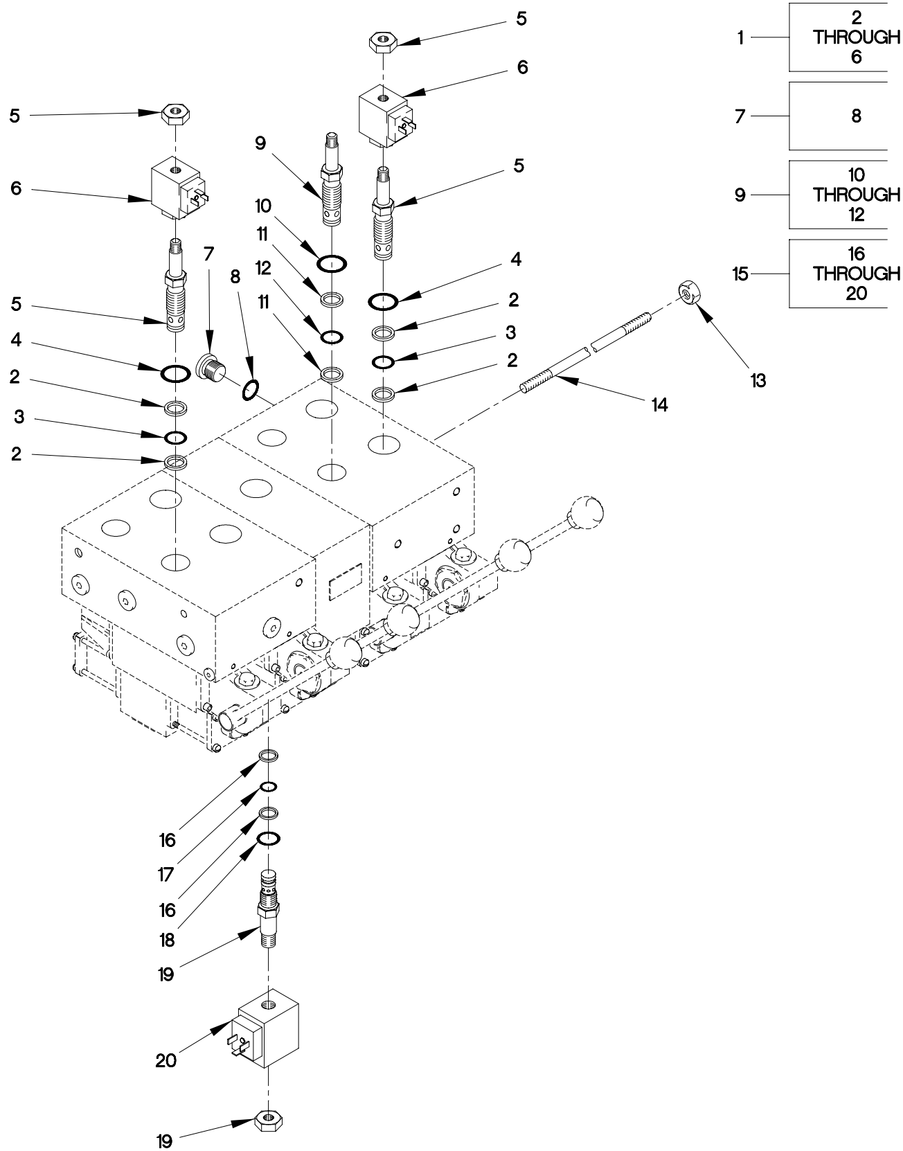
FIGURE 407. M1084 AND M1086 FOUR WAY DIRECTIONAL AND RELIEF VALVES
