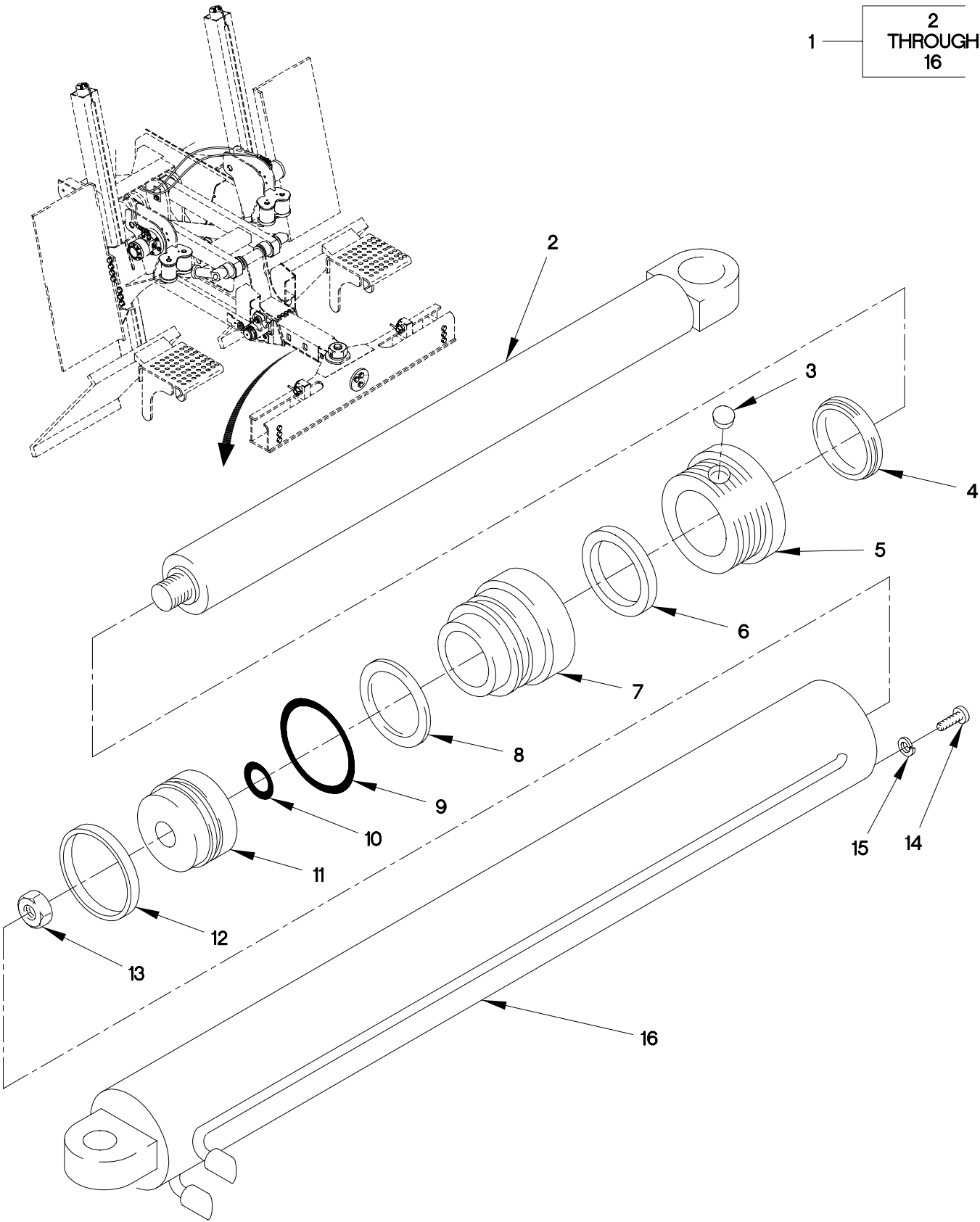
FIGURE 304. M1089 UNDERLIFT STINGER CYLINDER ASSEMBLY
