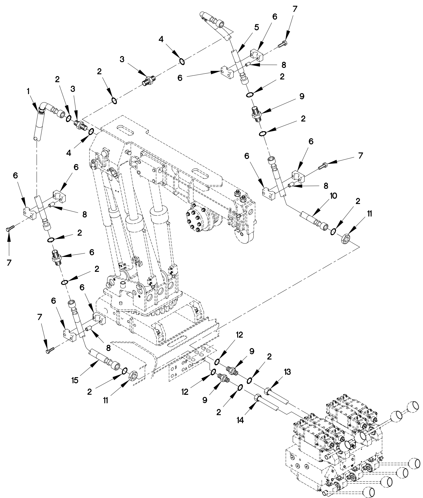
FIGURE 342. M1089 HYDRAULIC TELESCOPE HOSES AND FITTINGS
