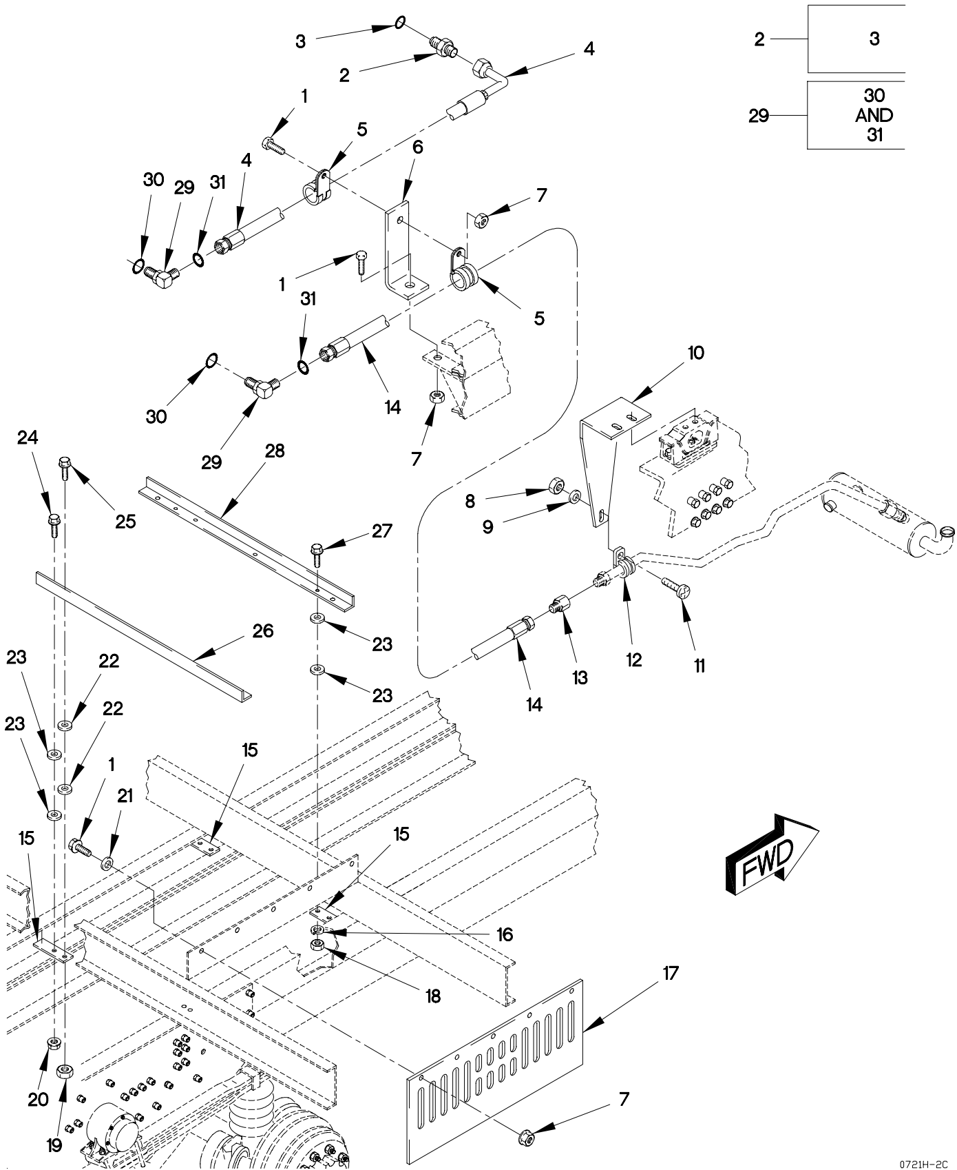
FIGURE 150. M1083, M1084, M1085, M1086, M1090 AND M1094 TRANSMISSION AUXILLIARY OIL COOLER BRACKETS, HOSES AND FITTINGS
