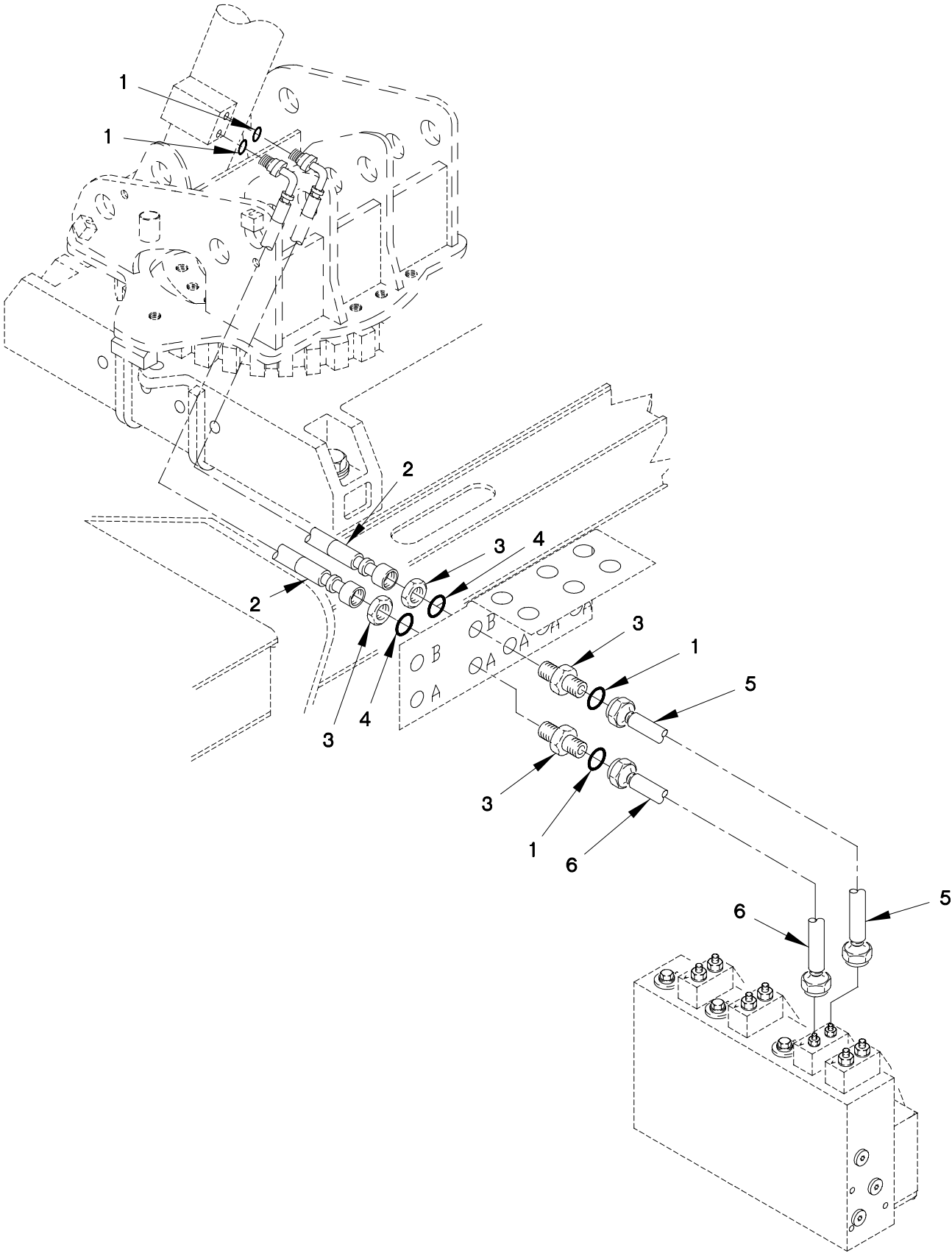
FIGURE 343. M1089 HYDRAULIC ERECTION HOSES AND FITTINGS
