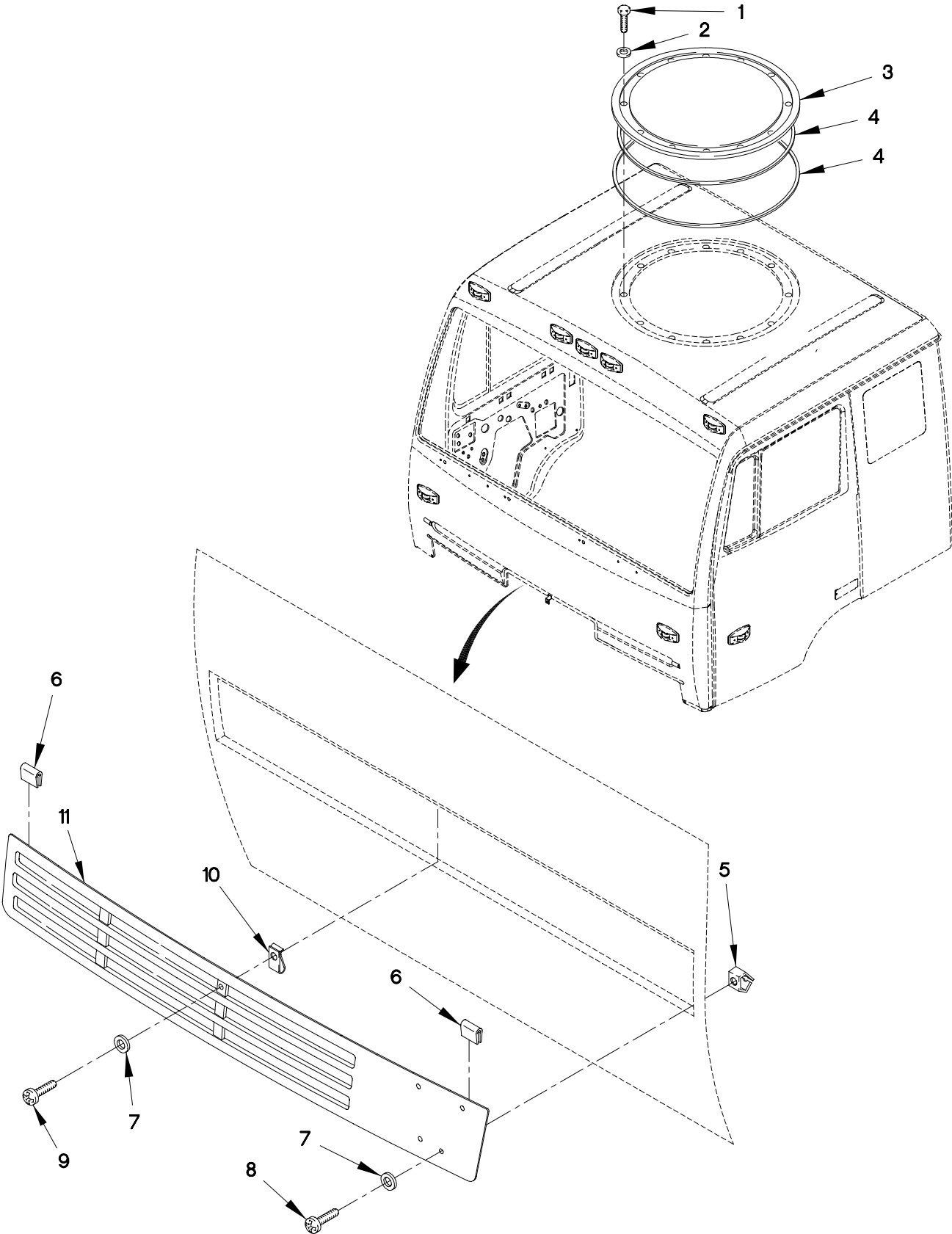
FIGURE 248. CAB ROOF HATCH AND FRONT GRILLE
