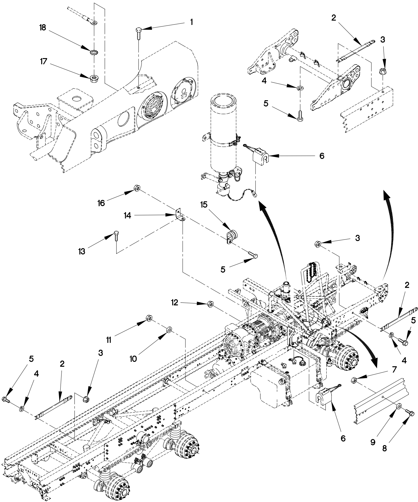
FIGURE 120. STARTER TO CHASSIS GROUND CABLE AND CLAMPS
