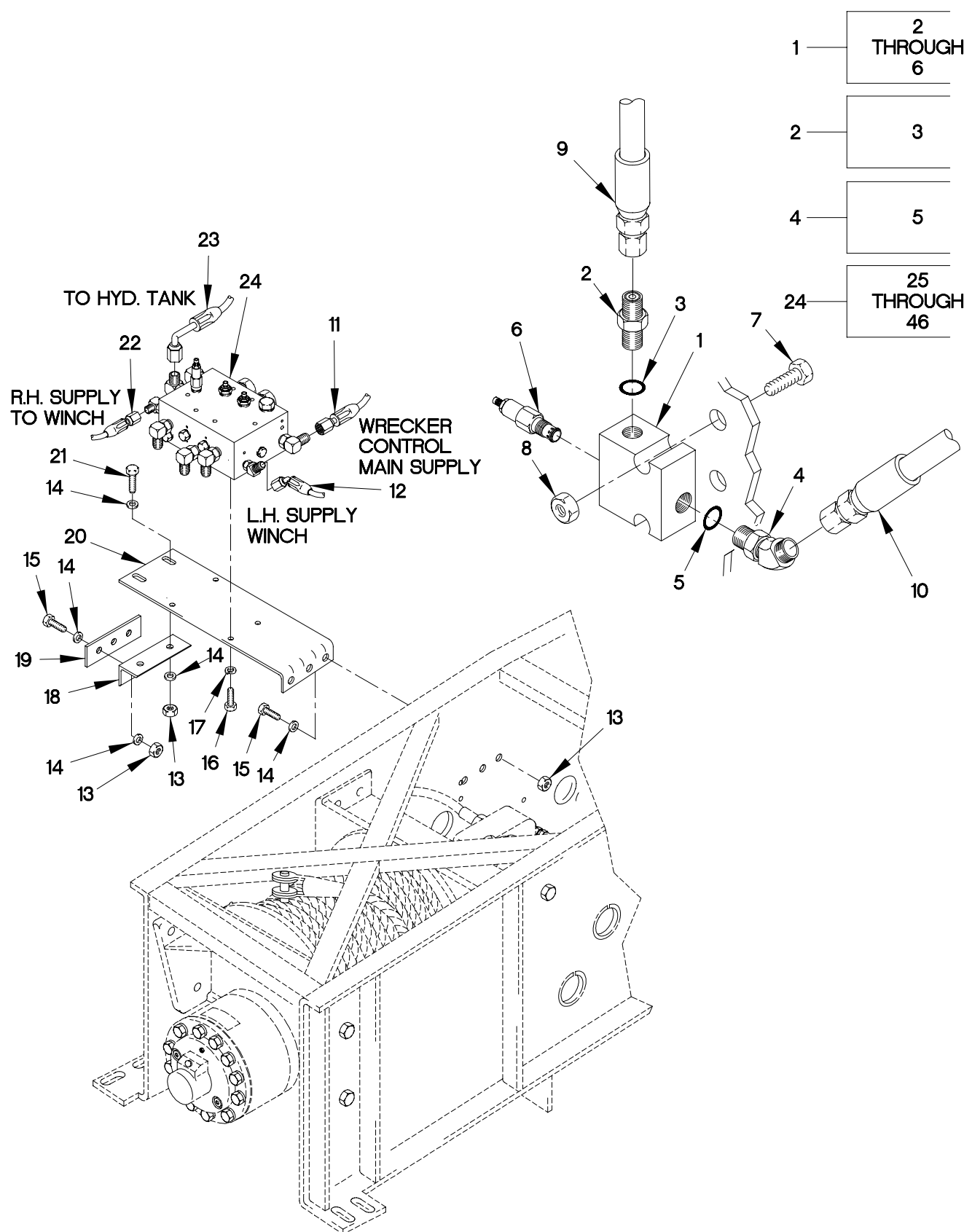
FIGURE 298. M1089 MONOBLOCK AND RELIEF VALVE (SHEET 1 OF 2)
