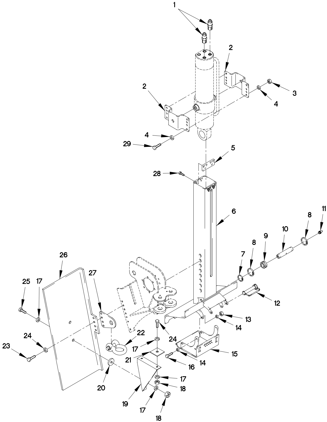
FIGURE 305. M1089 UNDERLIFT RIGHT AND LEFT STIFFLEG (SHEET 1 OF 2)
