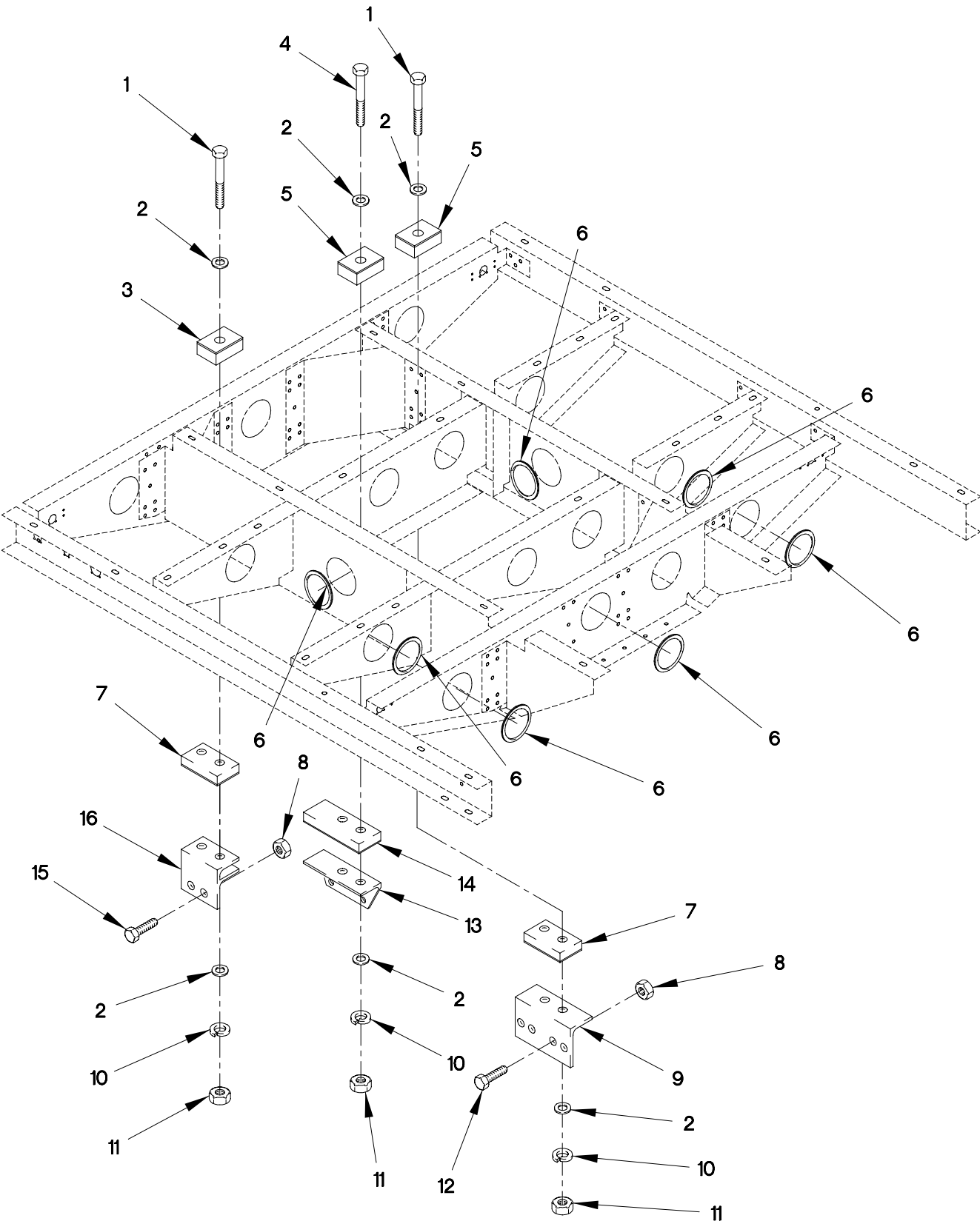
FIGURE 230. M1089 STOWAGE BOX MOUNT BRACKETS AND CUSHIONS
