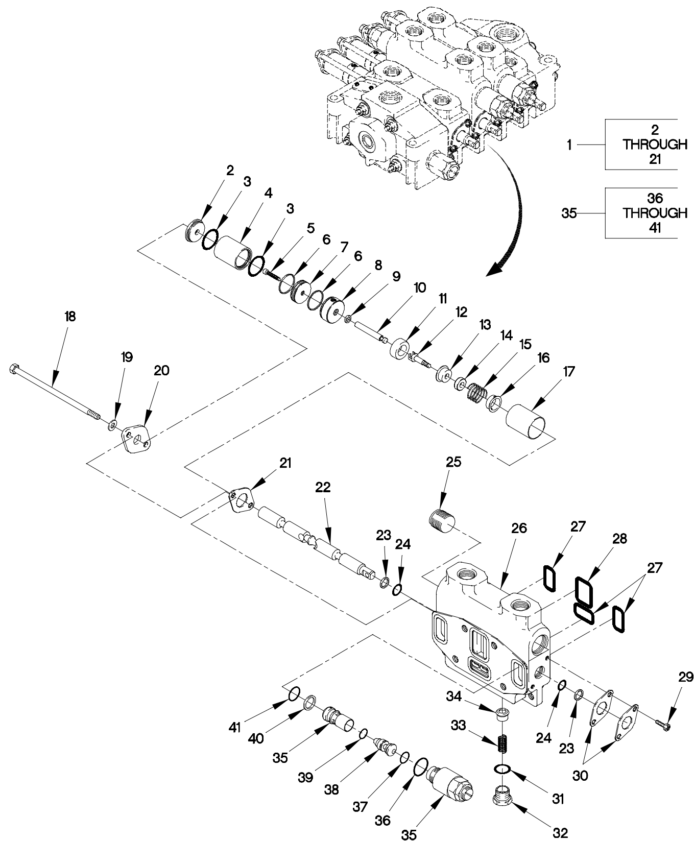
FIGURE 369. M1089 UNDERLIFT FOLD POSITION CONTROL VALVE
