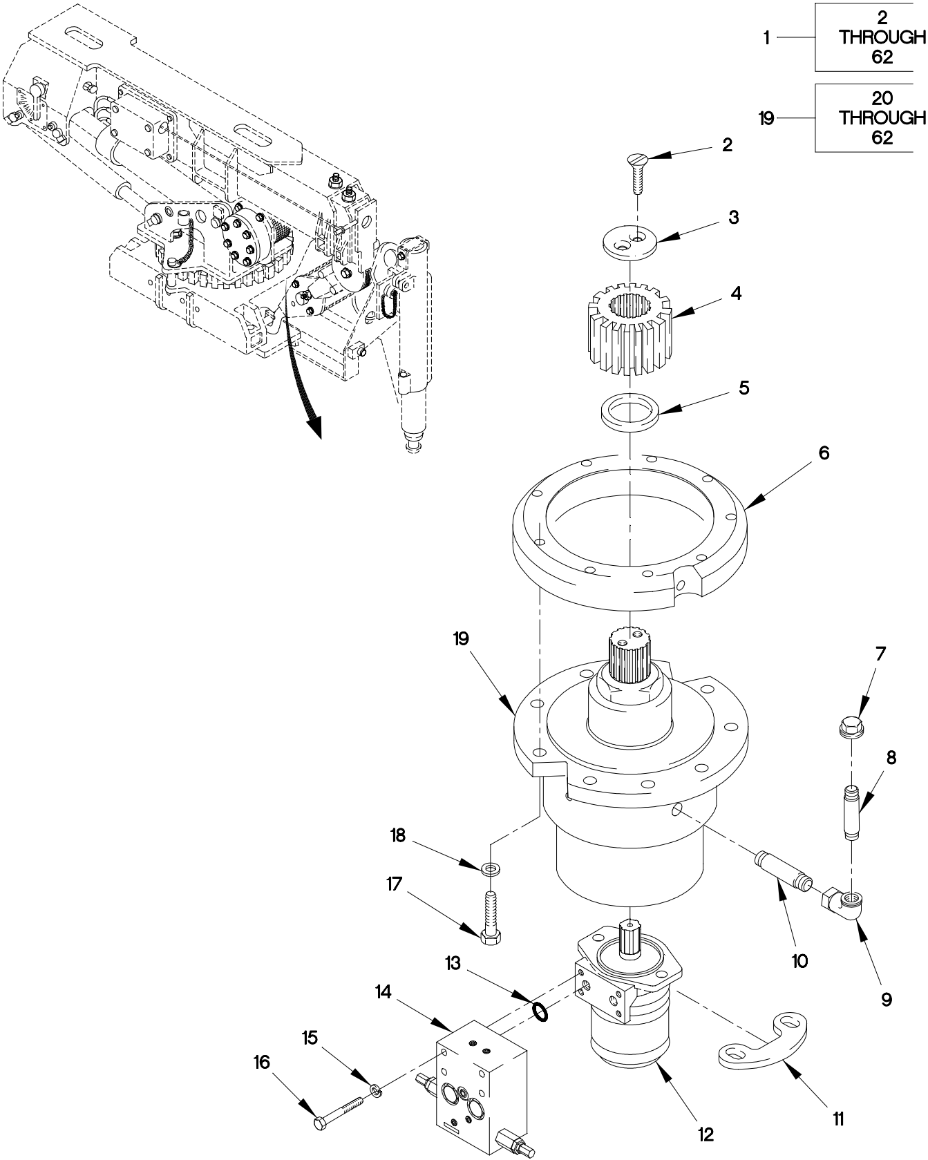
FIGURE 392. M1084 AND M1086 SWING DRIVE ASSEMBLY, HYDRAULIC MOTOR AND CROSS RELIEF VALVE (SHEET 1 OF 2)
