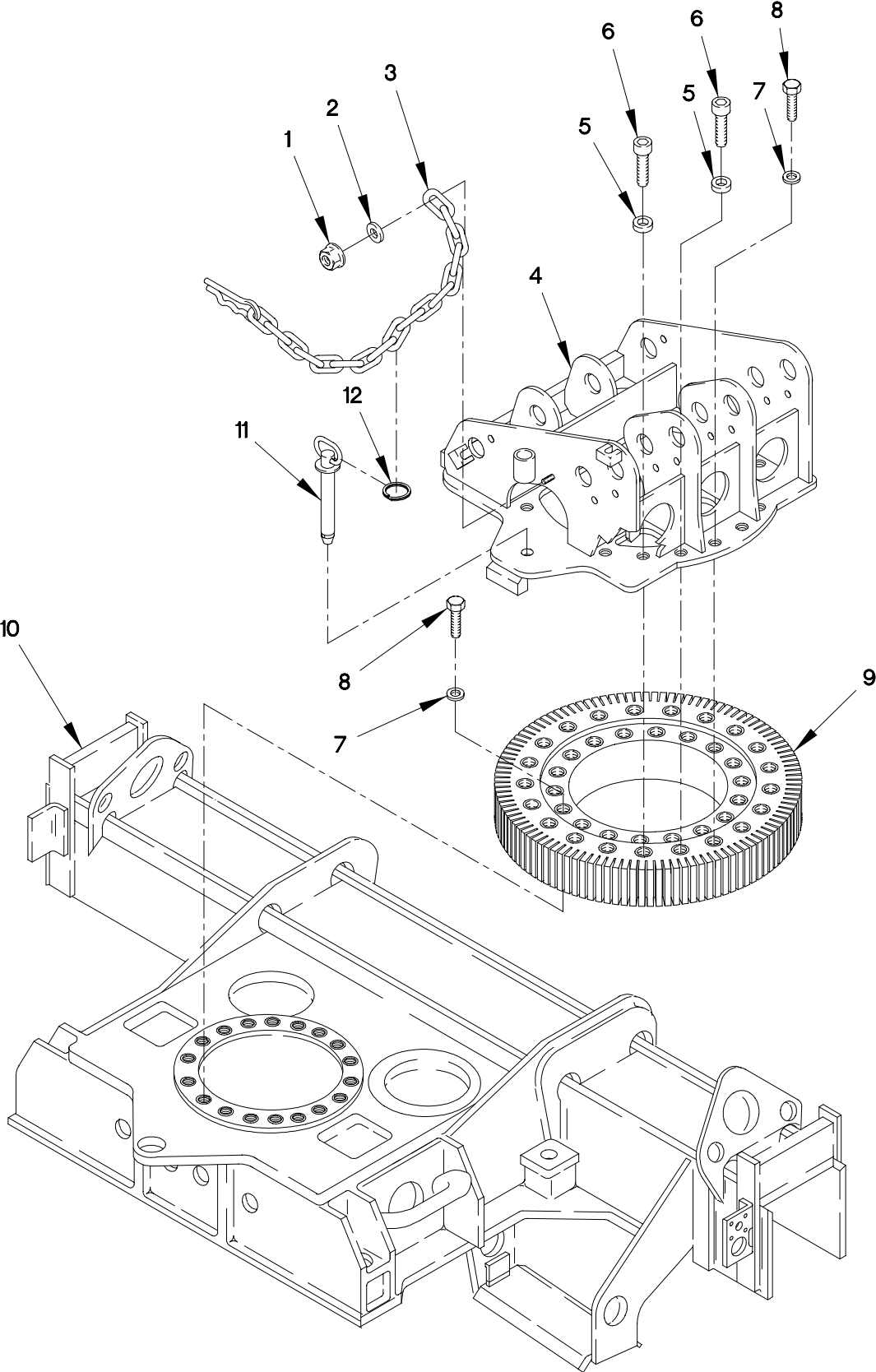
FIGURE 317. M1089 TURNTABLE AND SUBFRAME
