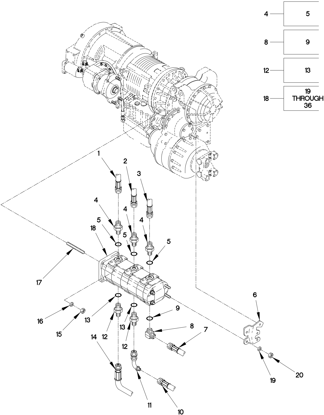
FIGURE 358. M1089 THREE STAGE HYDRAULIC PUMP, HOSES AND FITTINGS (SHEET 1 OF 2)
