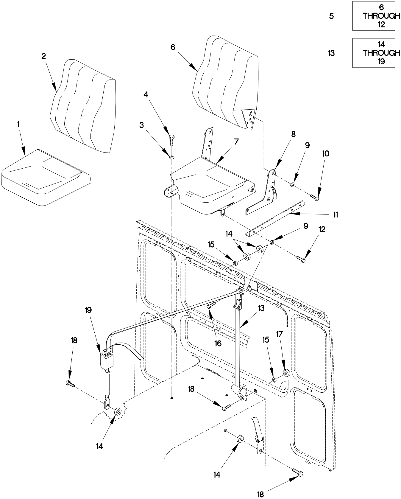
FIGURE 270. CENTER SEAT AND SEAT BELT
