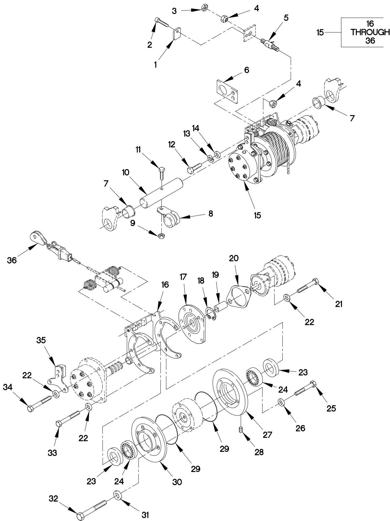
FIGURE 325. M1089 HOIST ASSEMBLY
