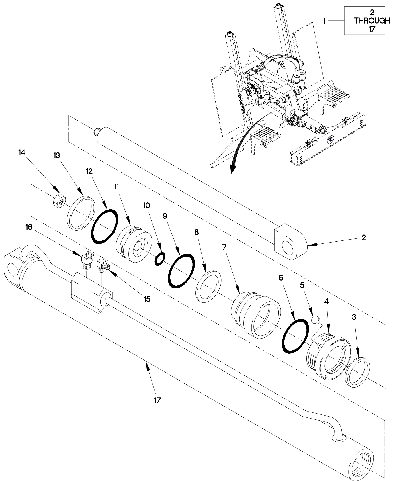
FIGURE 309. M1089 UNDERLIFT FOLD CYLINDER ASSEMBLY
