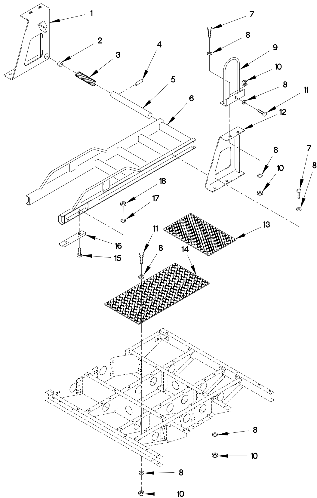
FIGURE 292. M1089 LADDER
