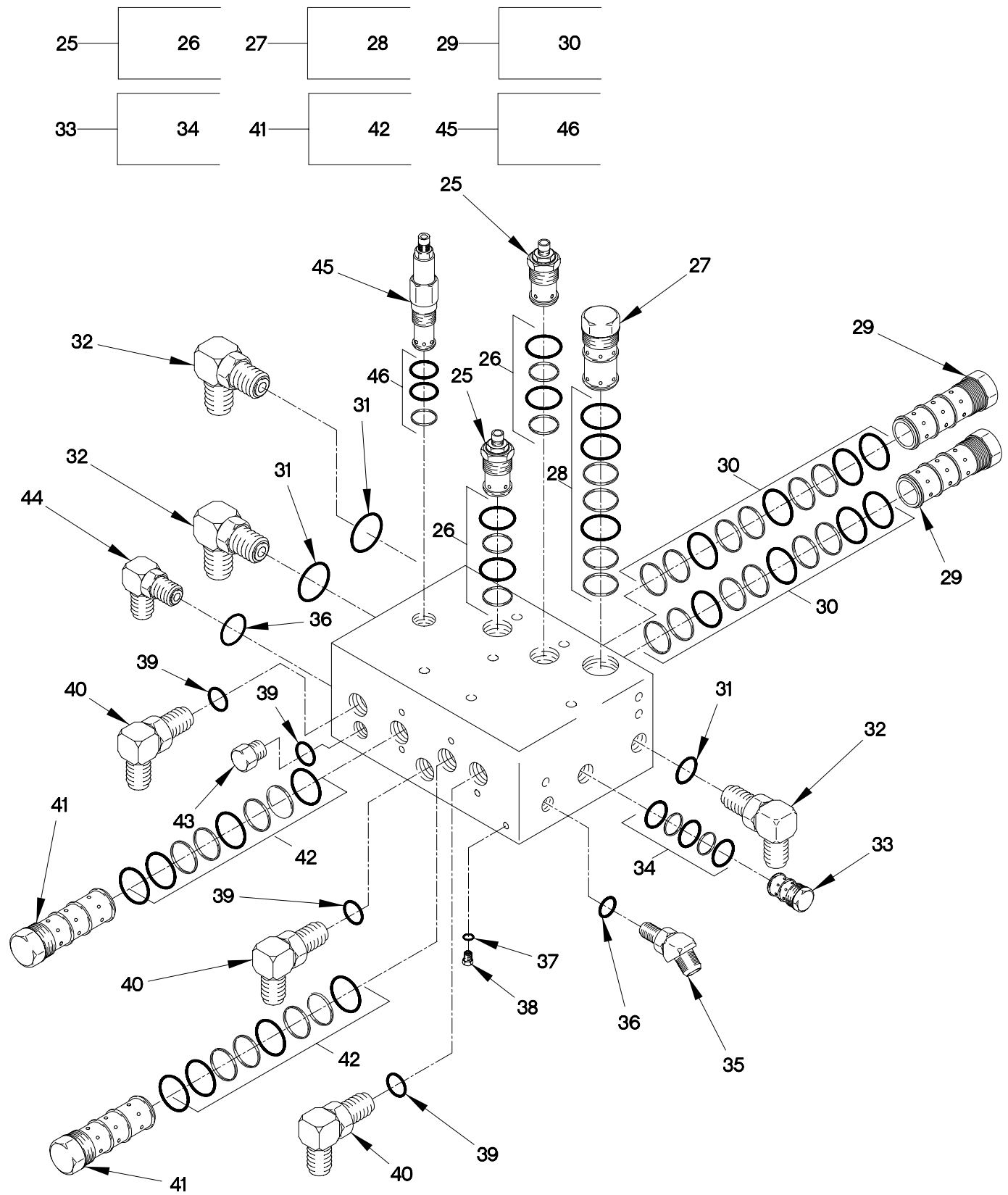
FIGURE 298. M1089 MONOBLOCK AND RELIEF VALVE (SHEET 2 OF 2)
