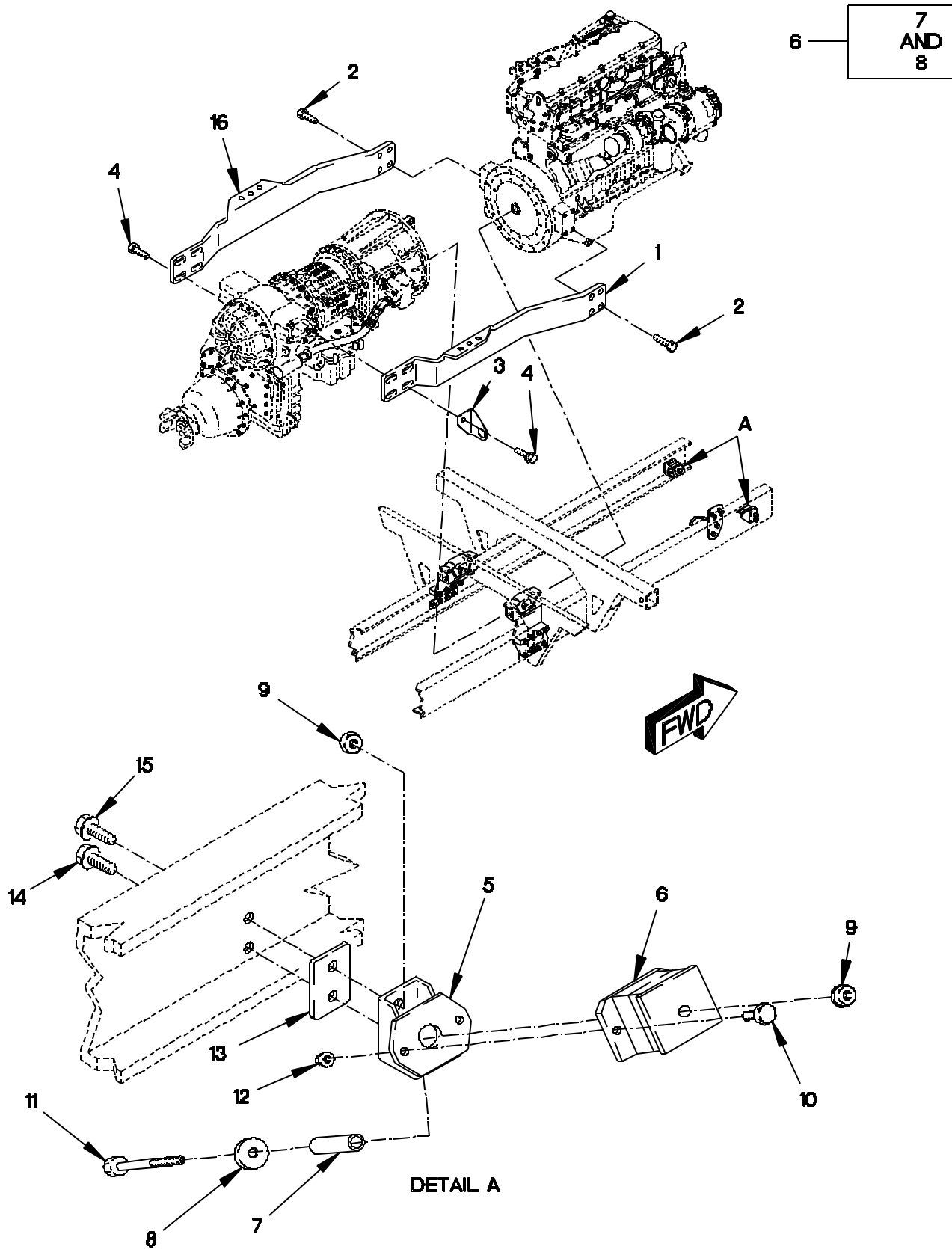
FIGURE 2. ENGINE MOUNTS
