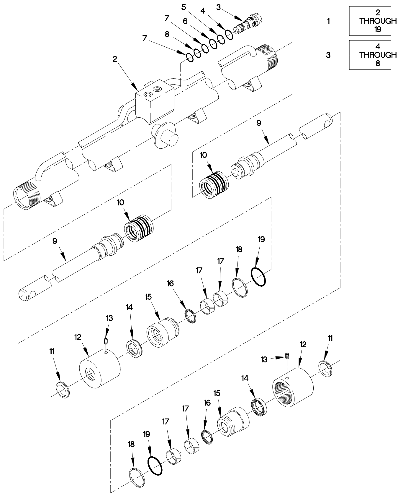
FIGURE 336. M1089 OUTRIGGER EXTEND CYLINDER
