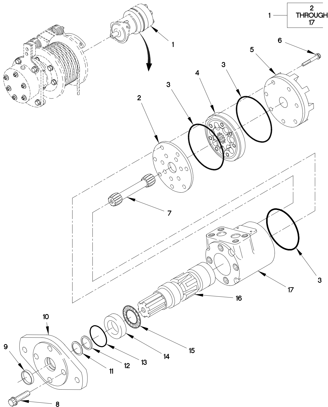
FIGURE 379. M1084 AND M1086 HOIST HYDRAULIC MOTOR
