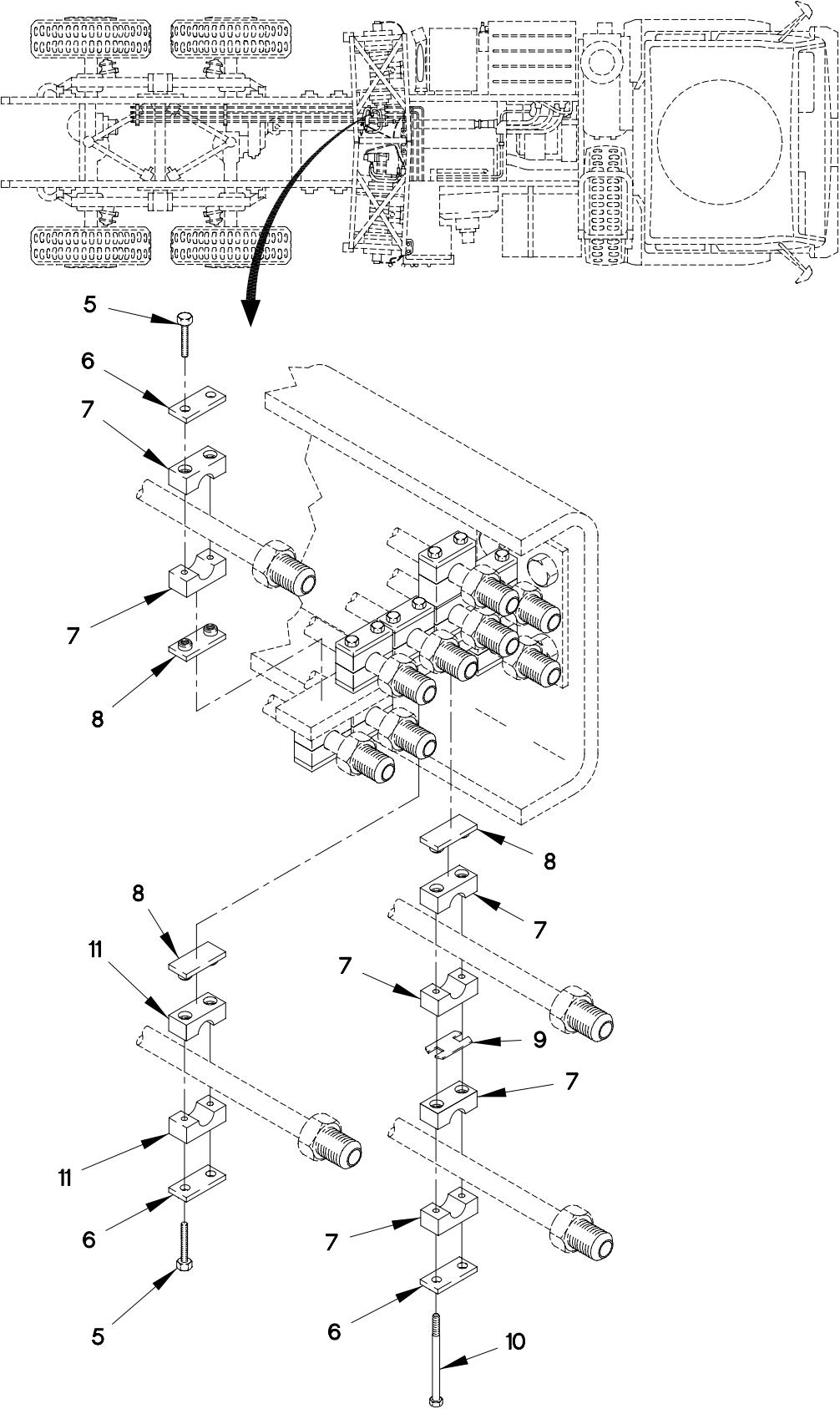
FIGURE 357. M1089 HYDRAULIC HOSES, TUBES AND FITTINGS (SHEET 2 OF 5)
