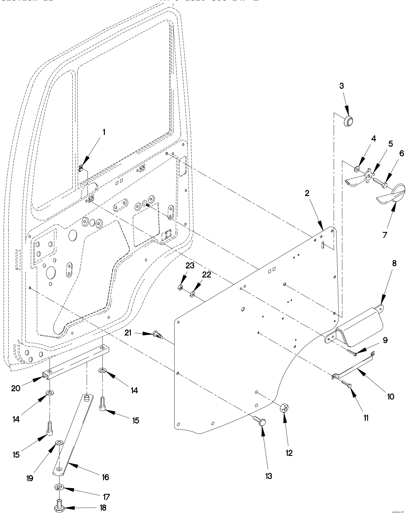
FIGURE 250. CAB DOOR FITTINGS
