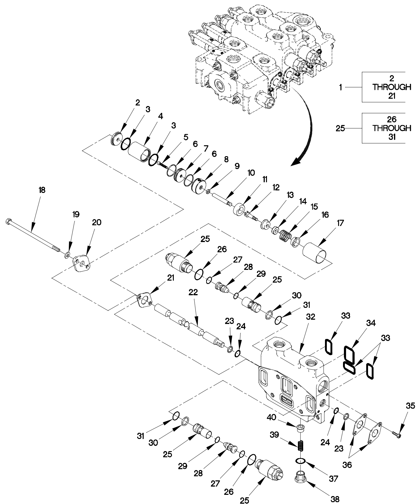
FIGURE 368. M1089 UNDERLIFT FOLD CONTROL VALVE
