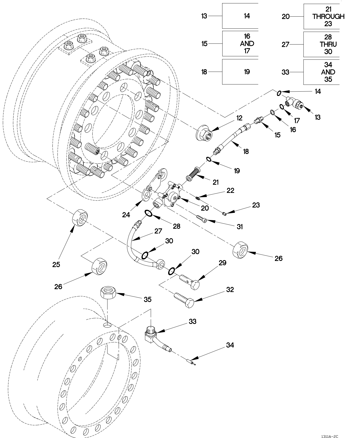
FIGURE 207. WHEEL ASSEMBLY AND CTIS VALVE (SHEET 2 OF 2)
