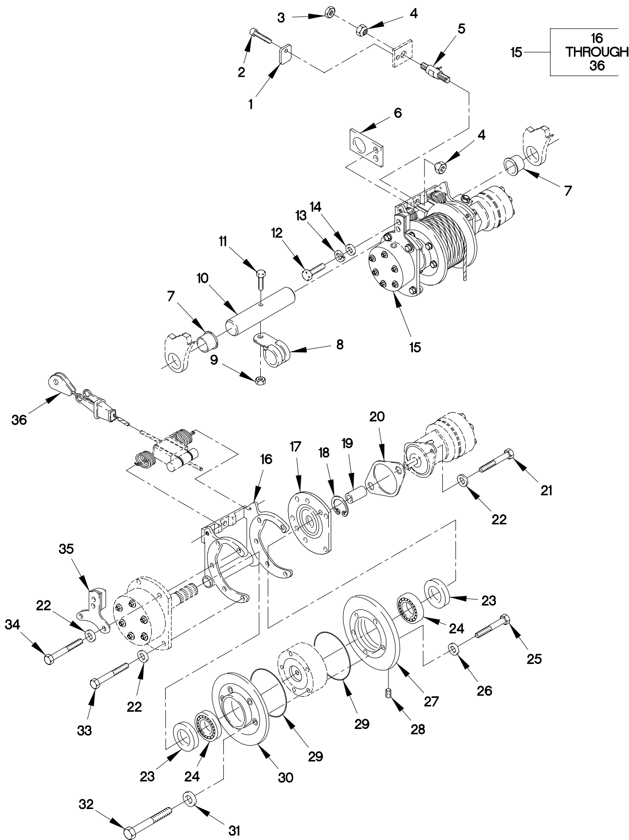
Figure 378. M1084 AND M1086 HOIST ASSEMBLY AND TENSION LOAD CELL
