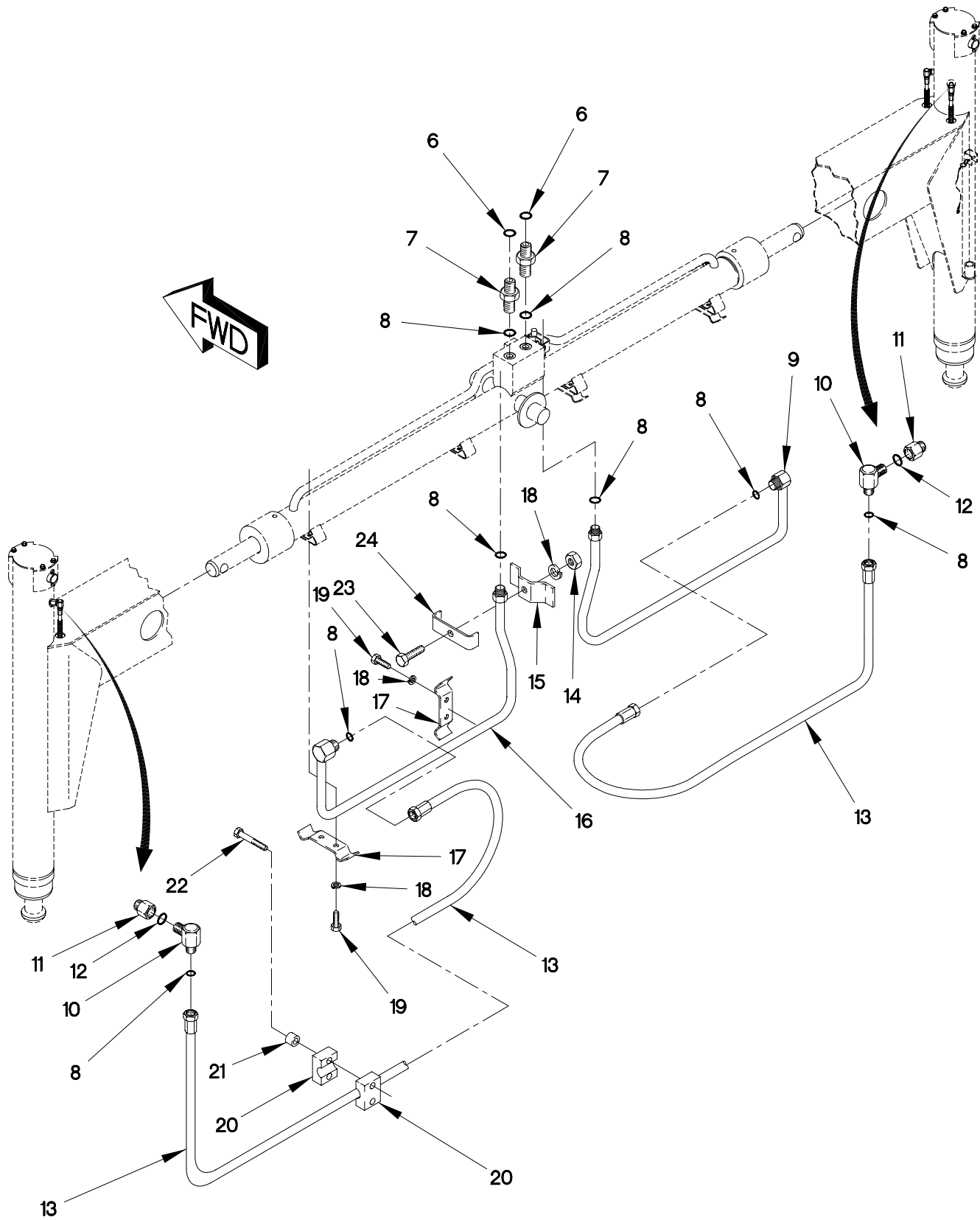
FIGURE 335. M1089 OUTRIGGER BEAM, HOSES AND FITTINGS (SHEET 2 OF 3)
