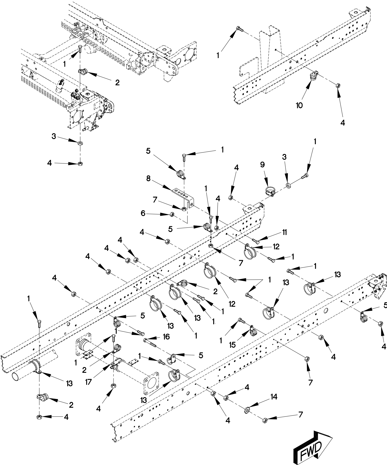
FIGURE 191. M1083 AND M1092 PNEUMATIC HOSE ROUTING LOOP CLAMPS AND BRACKETS (SHEET 1 OF 3)
