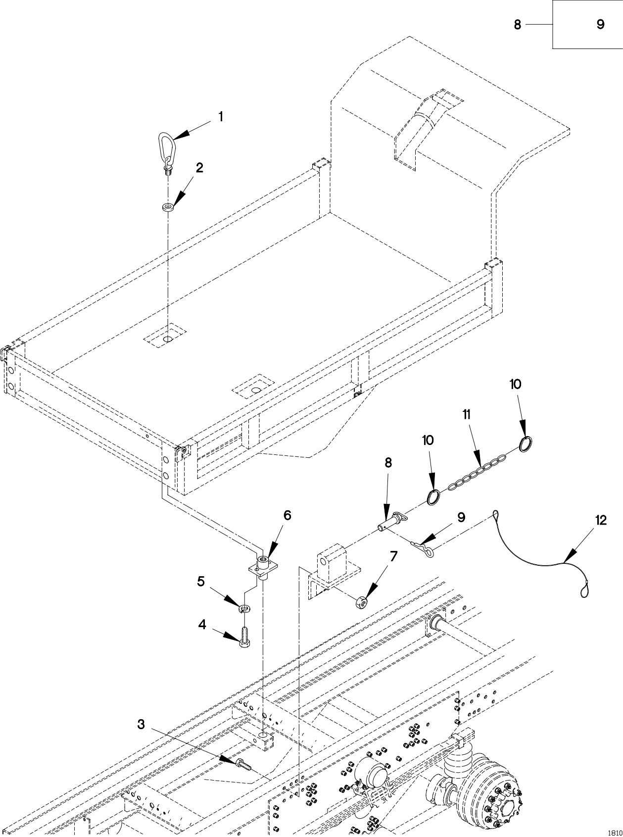
FIGURE 289. M1090 AIRDROP REAR LIFTING EYE AND BED HOLD DOWN BRACKET
