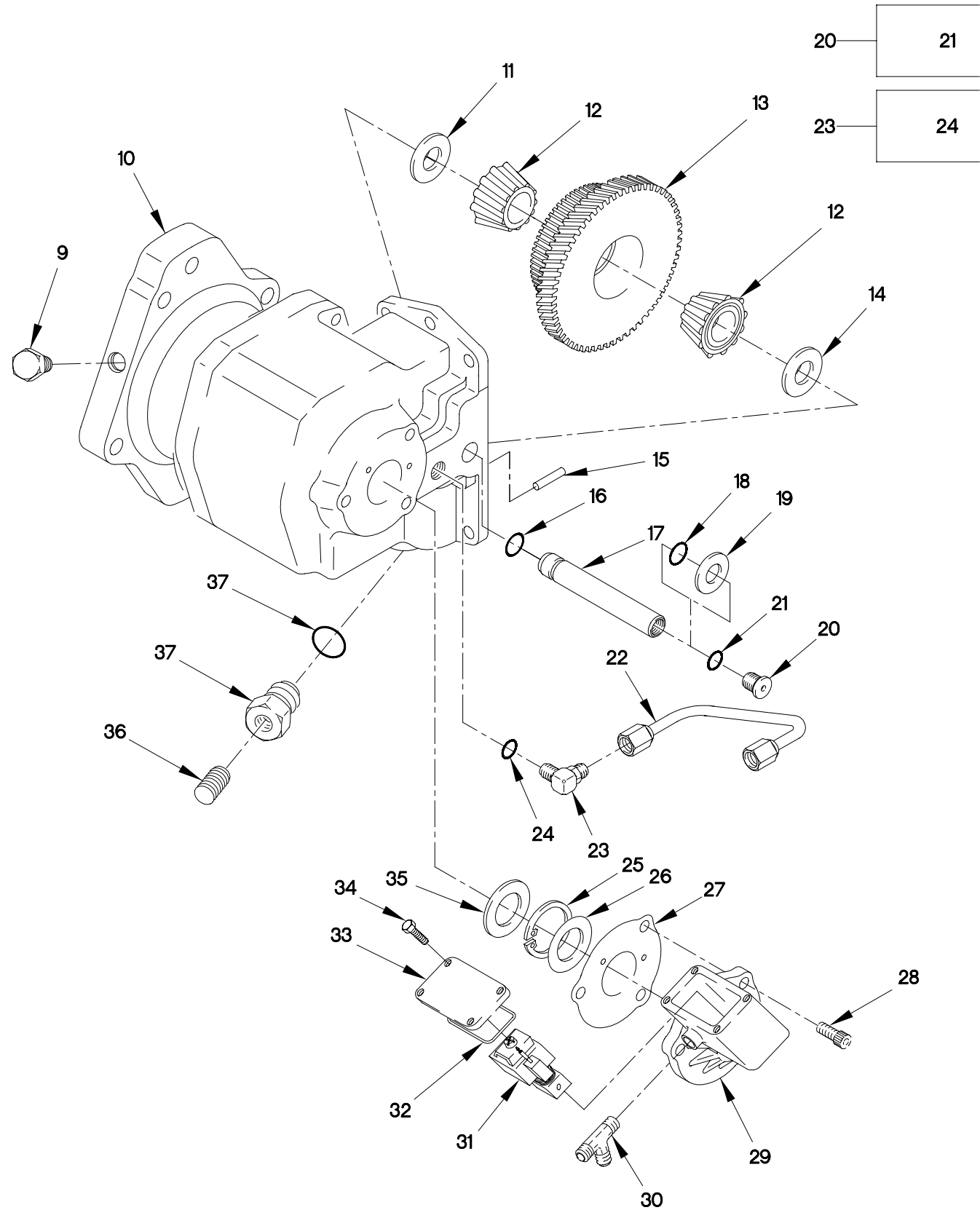
FIGURE 417. POWER TAKE-OFF ASSEMBLY (SHEET 2 OF 3)
