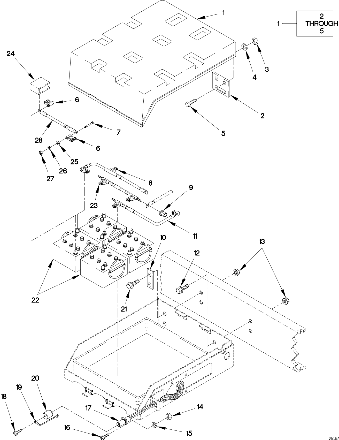
FIGURE 79. BATTERIES, BOX, GUARD AND CABLES (SHEET 1 of 3)
