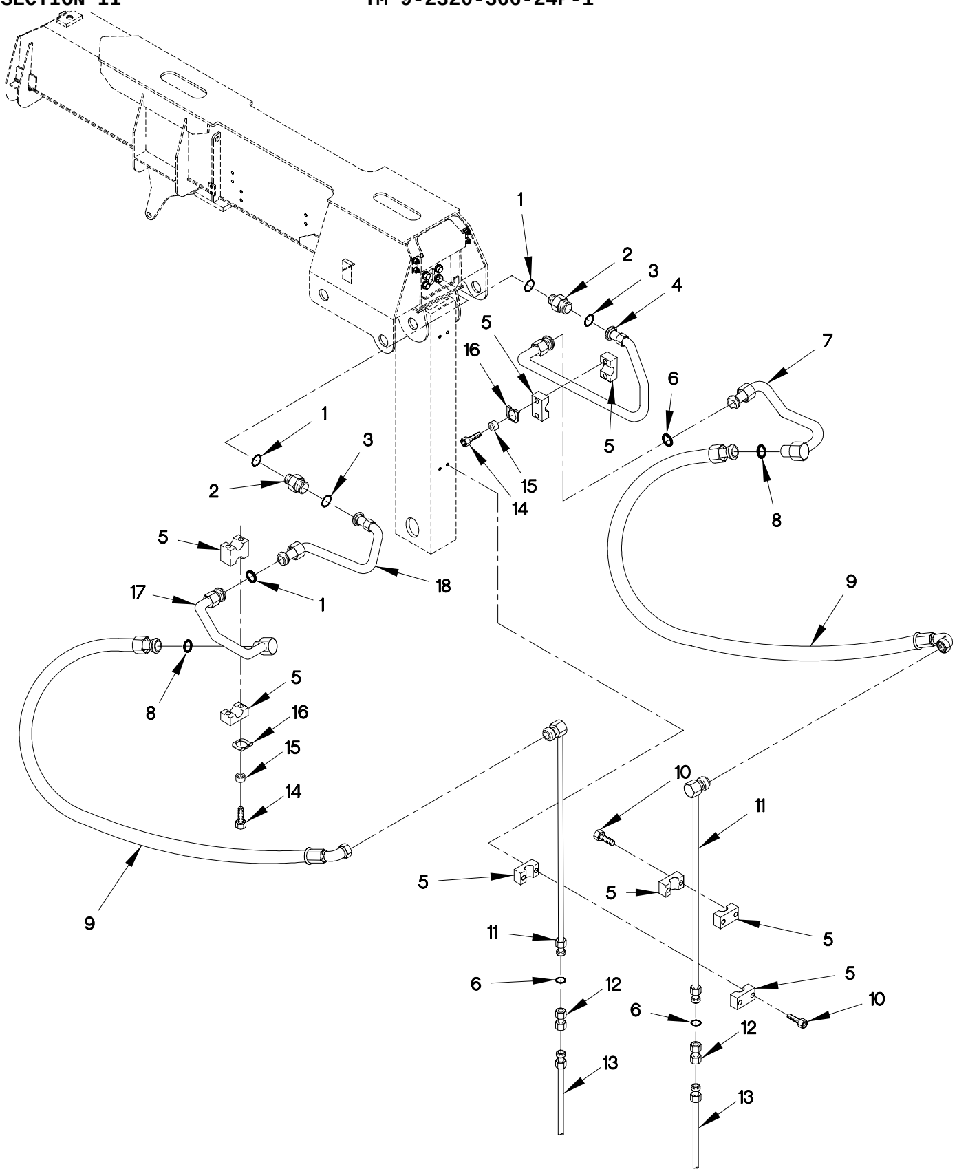
FIGURE 397. M1084 AND M1086 HYDRAULIC TELESCOPE HOSES (SHEET 1 OF 2)
