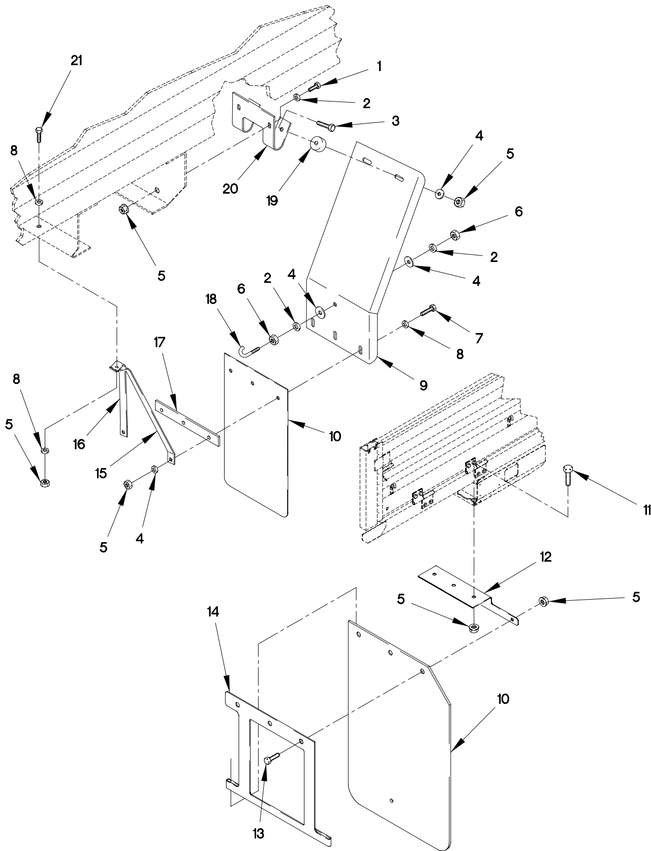
FIGURE 262. M1086 REAR FENDERS AND SPLASH GUARDS
