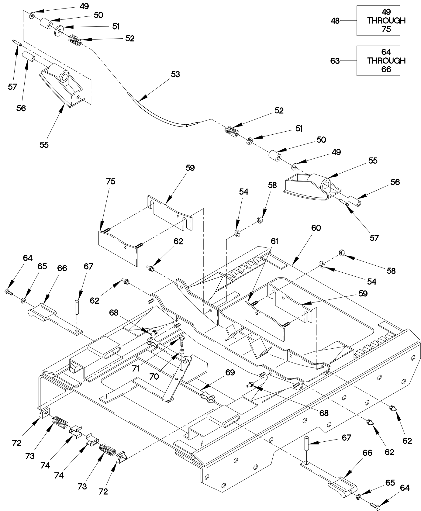
FIGURE 237. M1088 FIFTH WHEEL ASSEMBLY (SHEET 3 OF 4)
