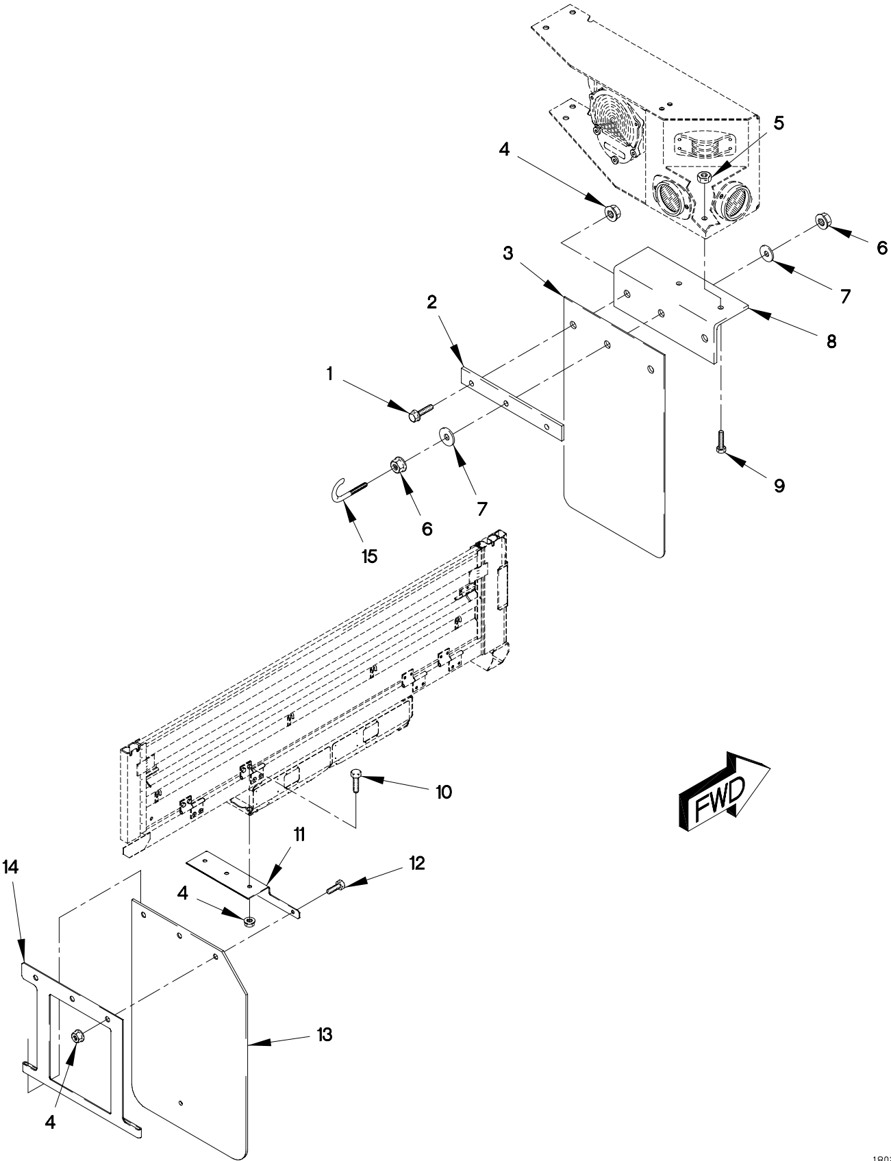
FIGURE 259. M1083 REAR FENDERS AND SPLASH GUARDS
