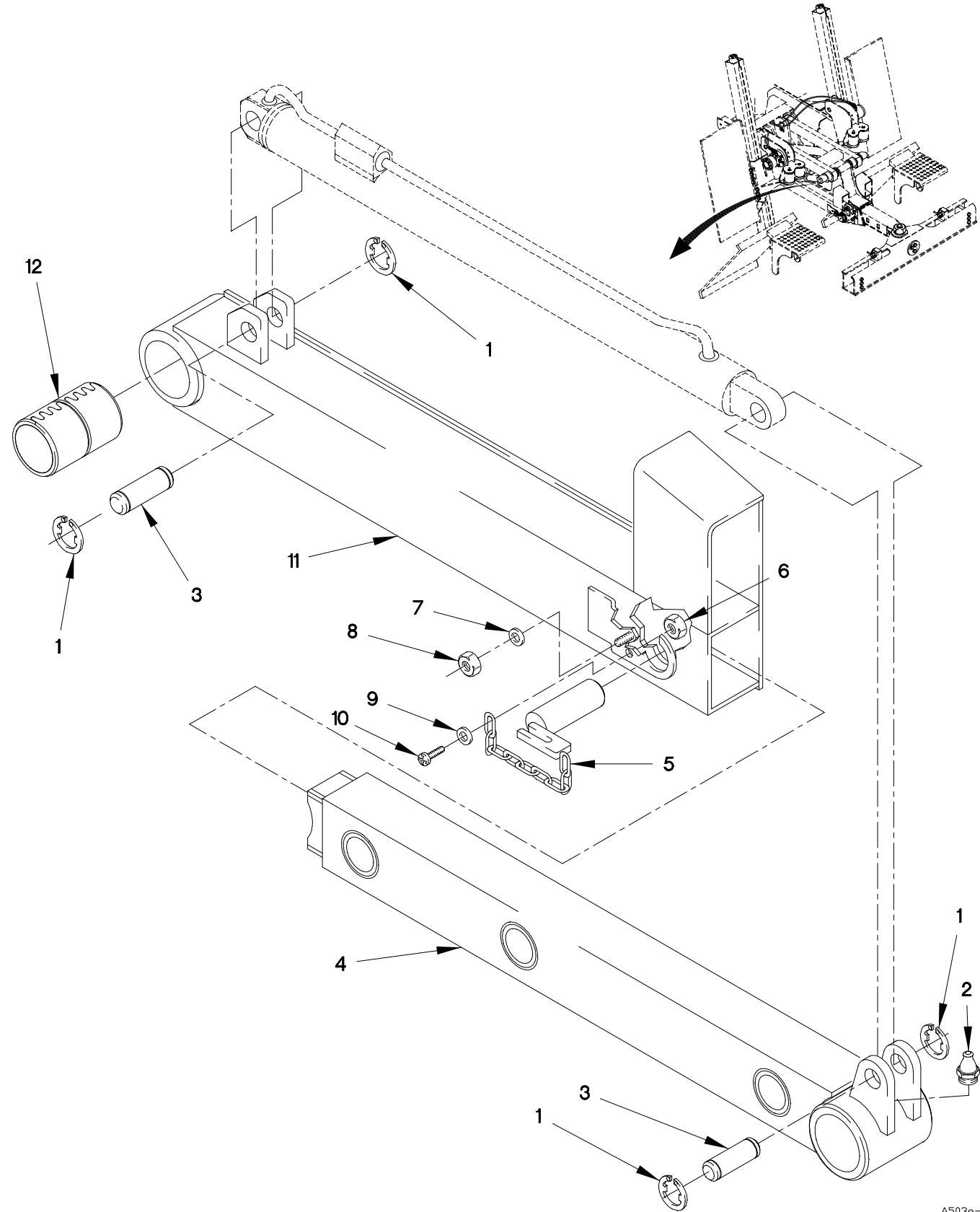
FIGURE 303. M1089 UNDERLIFT LOWER ARM FOLDING BOOM CYLINDER
