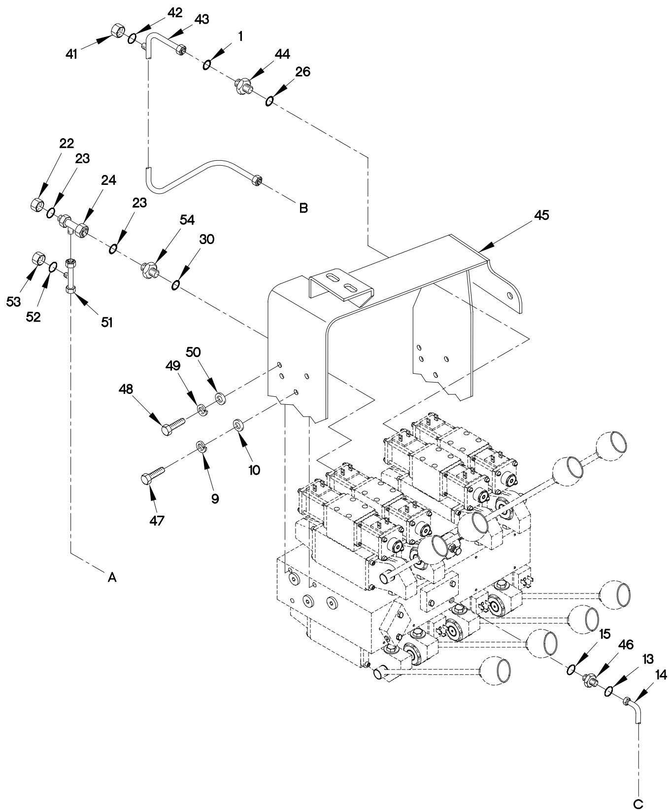
FIGURE 345. M1089 EIGHT BANK VALVE HOUSING ASSEMBLY (SHEET 2 OF 2)
