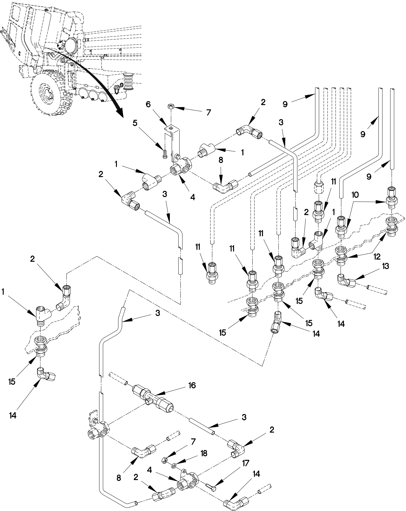
FIGURE 203. PARK CONTROL, EMERGENCY/SERVICE GLADHAND TWO-WAY CHECK VALVE, HOSES AND FITTINGS
