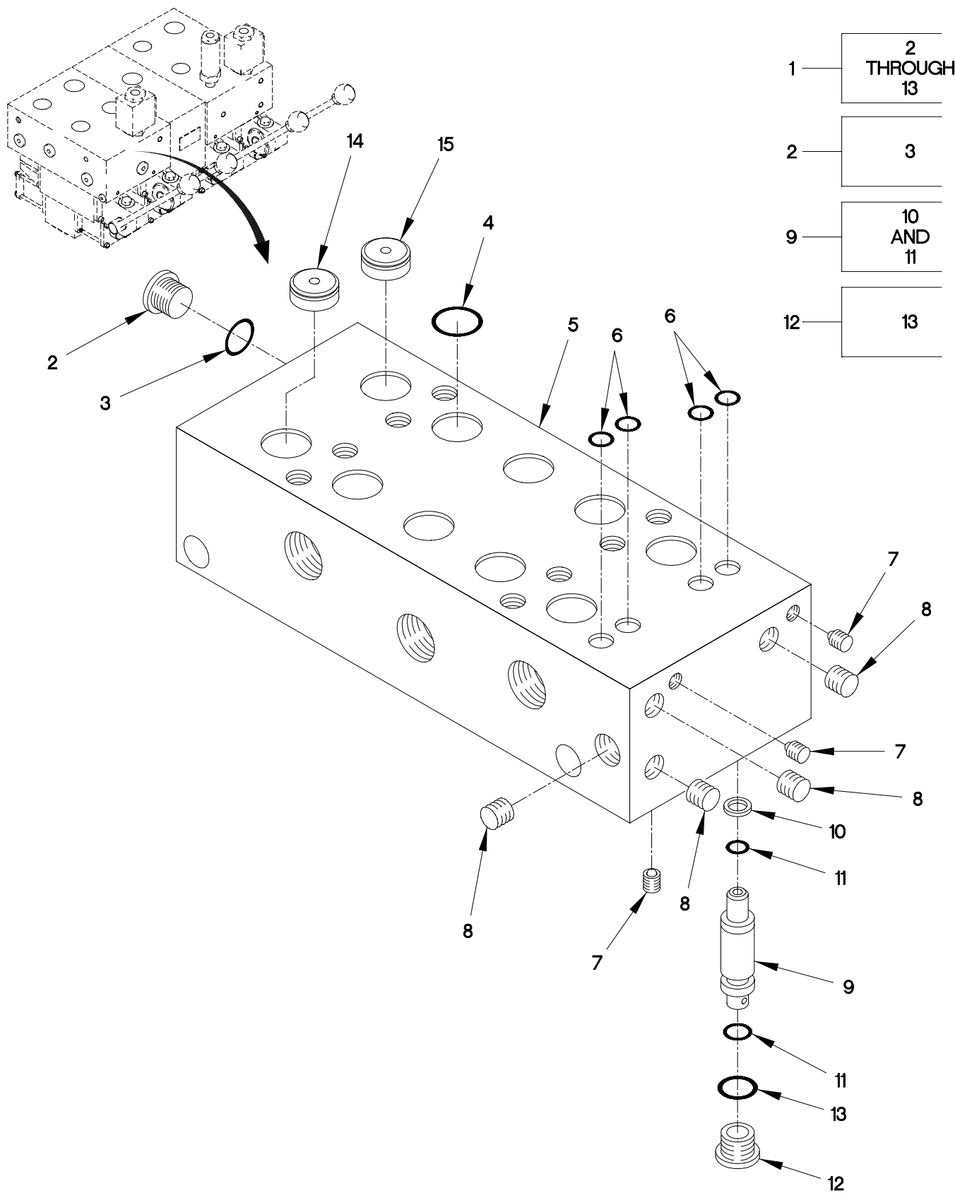
FIGURE 408. M1084 AND M1086 FOUR WAY LIFT/HOIST VALVES MANIFOLD
