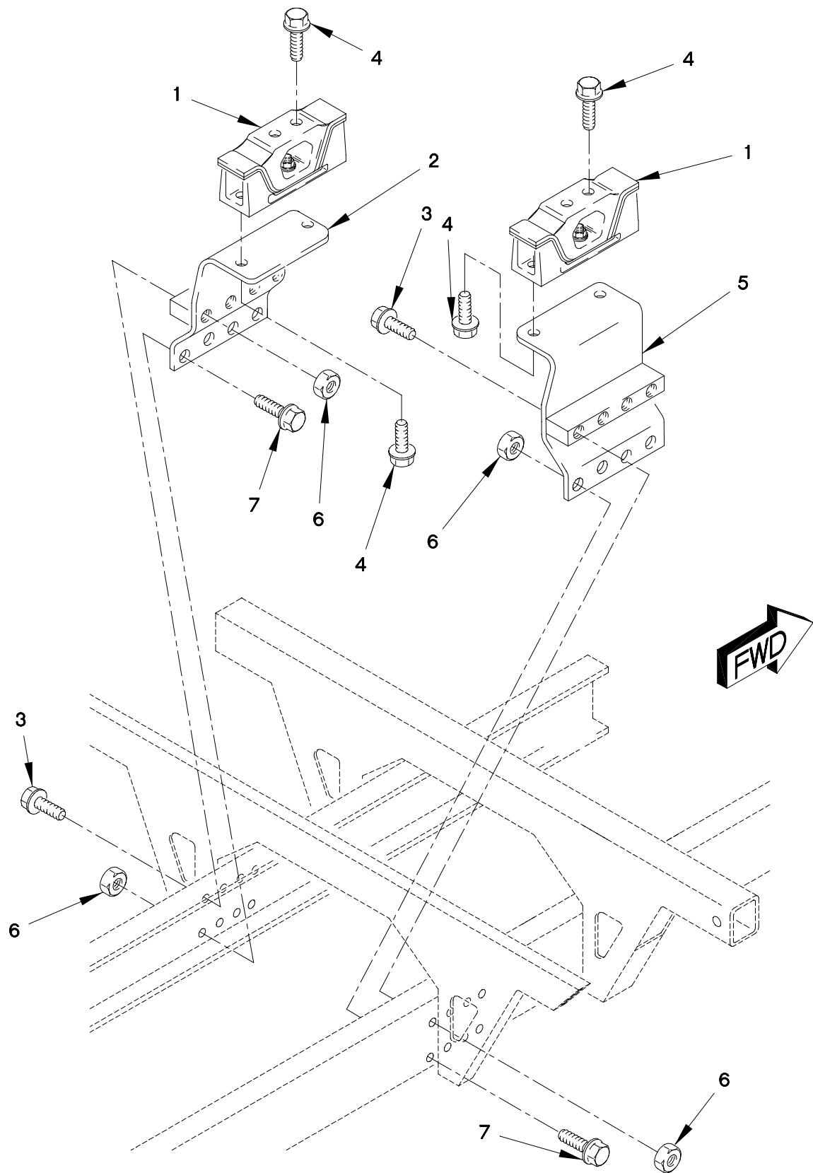
FIGURE 134. TRANSMISSION MOUNTS
