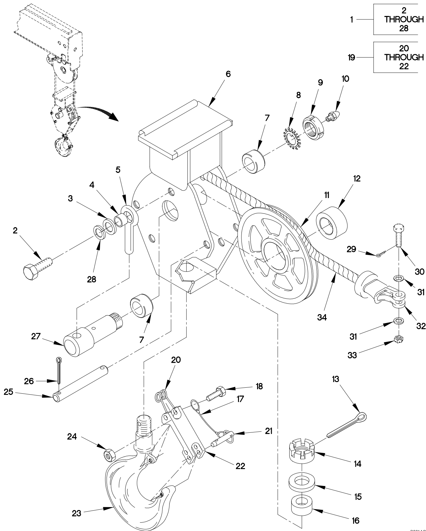
FIGURE 344. M1089 HOOK BLOCK AND CABLE ASSEMBLY
