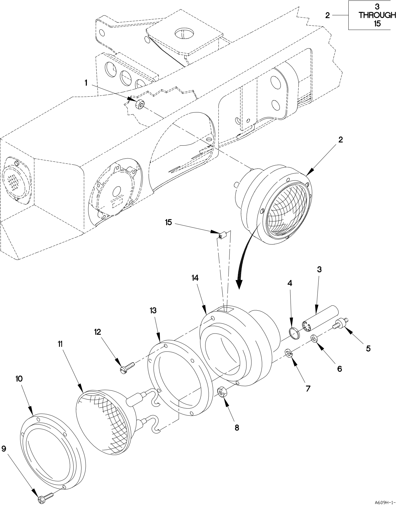
FIGURE 66. HEADLAMP ASSEMBLY
