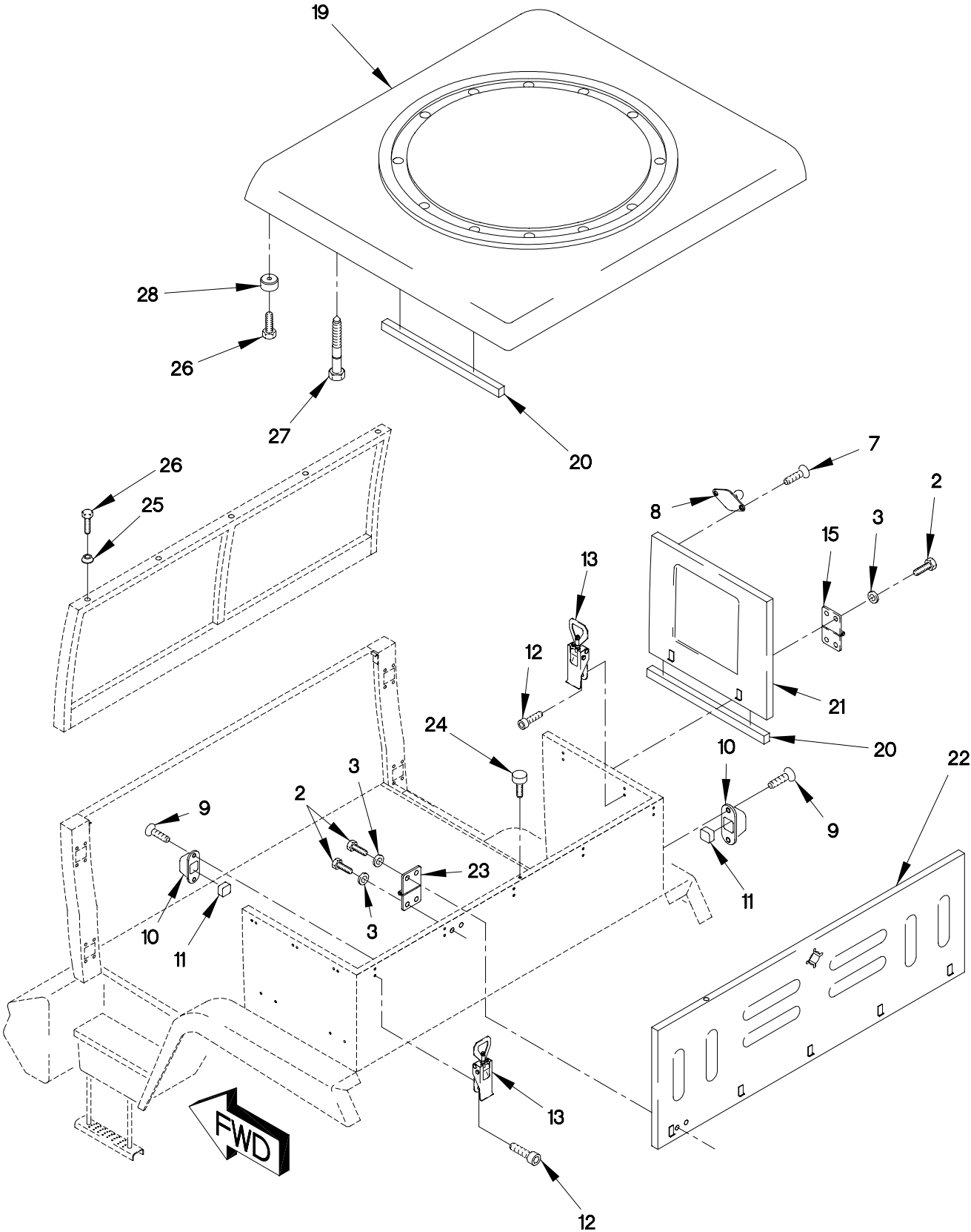
FIGURE 246. AIR DROP CAB ASSEMBLY, DOORS AND HINGES (SHEET 2 OF 4)
