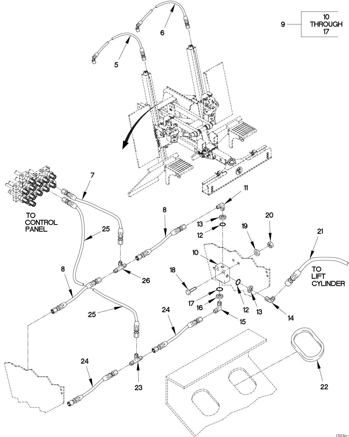
FIGURE 313. M1089 UNDERLIFT HYDRAULIC VALVES, HOSES AND FITTINGS (SHEET 2 OF 2)
