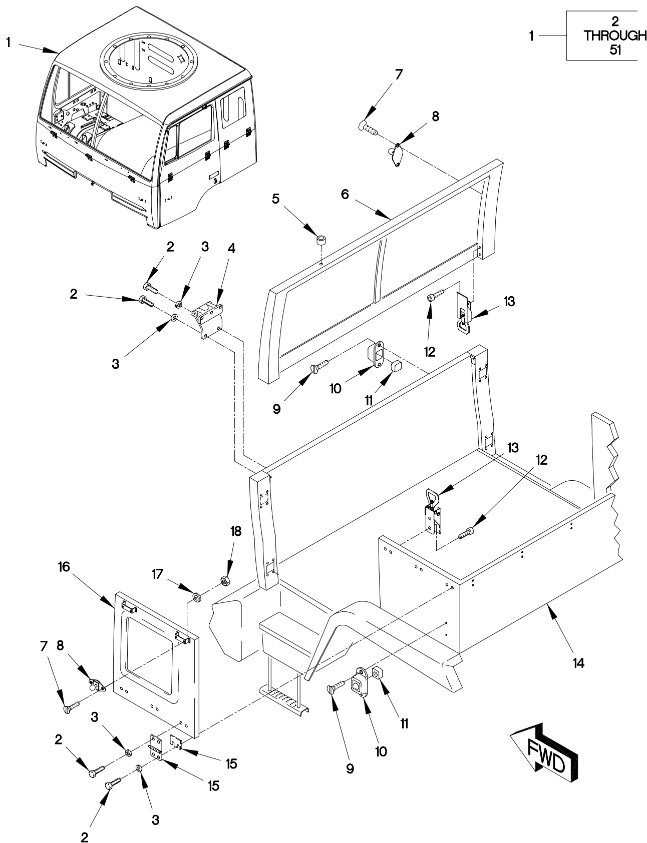
FIGURE 246. AIR DROP CAB ASSEMBLY, D00RS AND HINGES (SHEET 1 OF 4)
