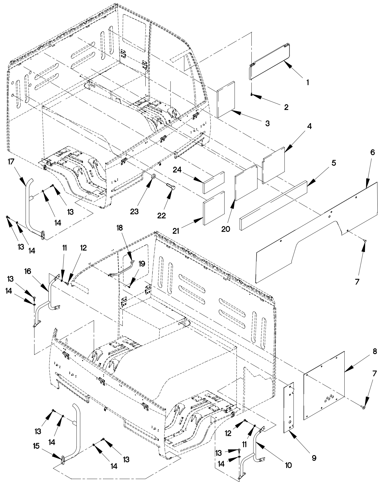
FIGURE 269. AIR DROP PANELS, VISORS AND BOARDING HANDLES
