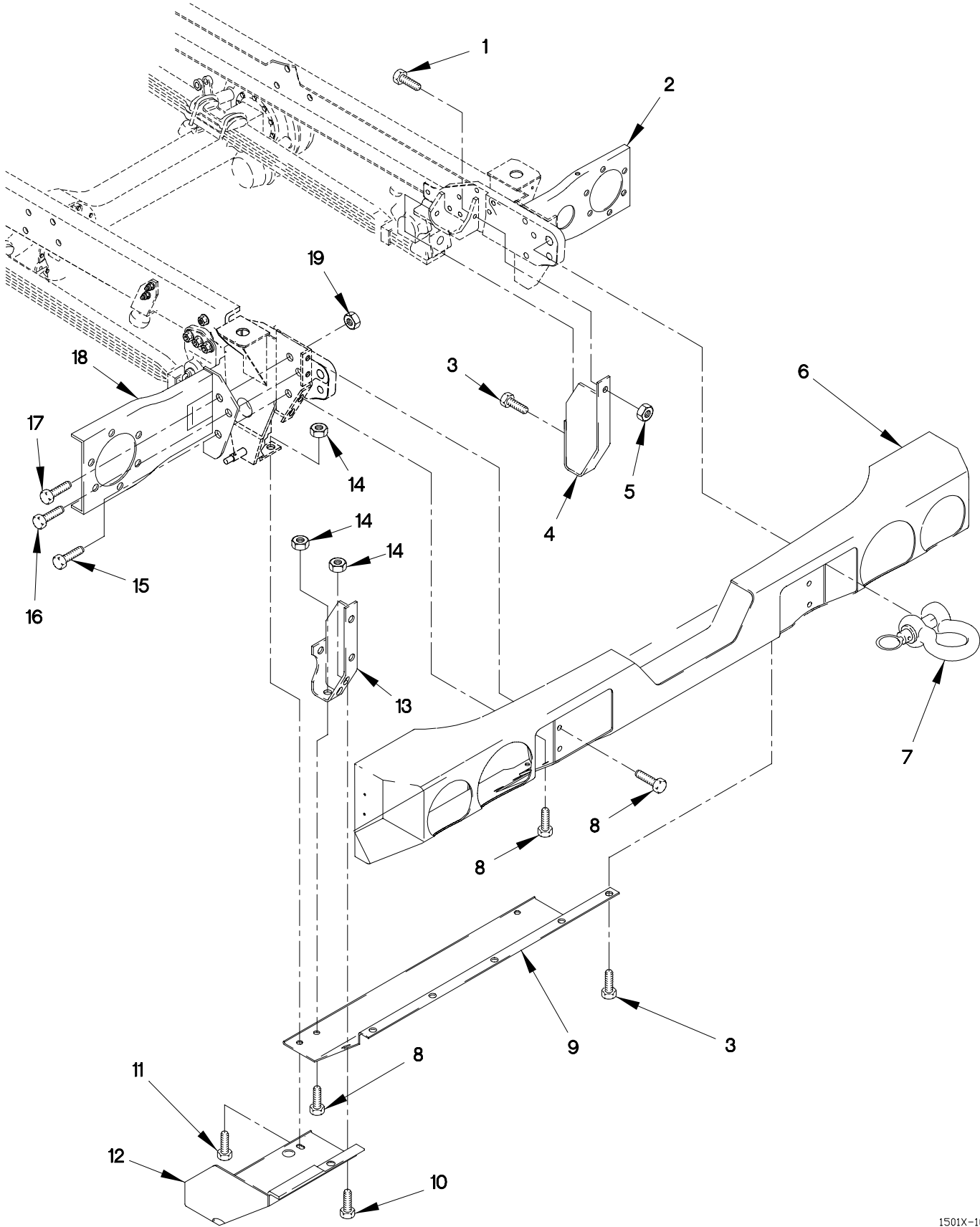
FIGURE 232. FRONT BUMPER AND GRAVEL DEFLECTOR
