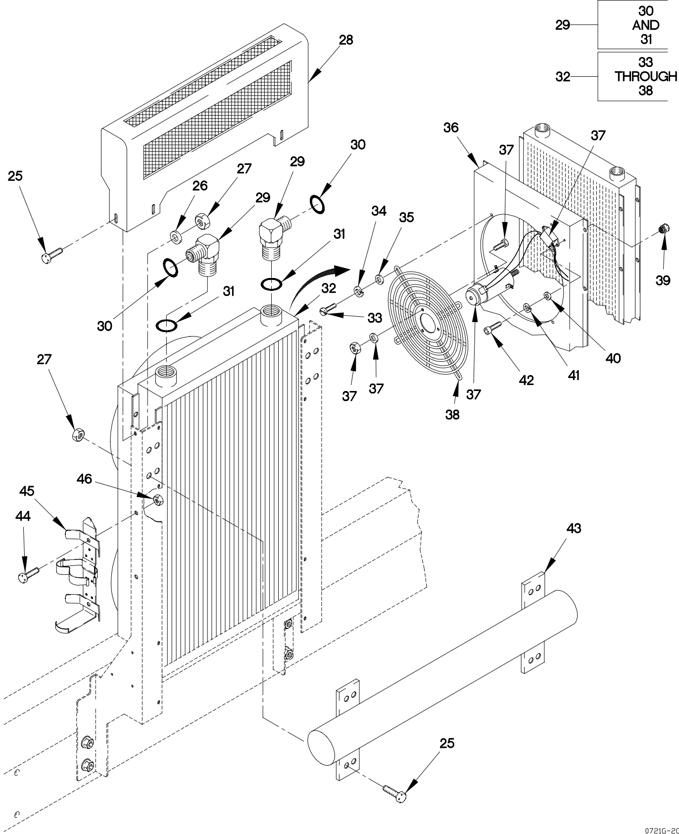
FIGURE 148. M1088 AND M1089 TRANSMISSION AUXILLIARY OIL COOLER (SHEET 2 OF 2)
