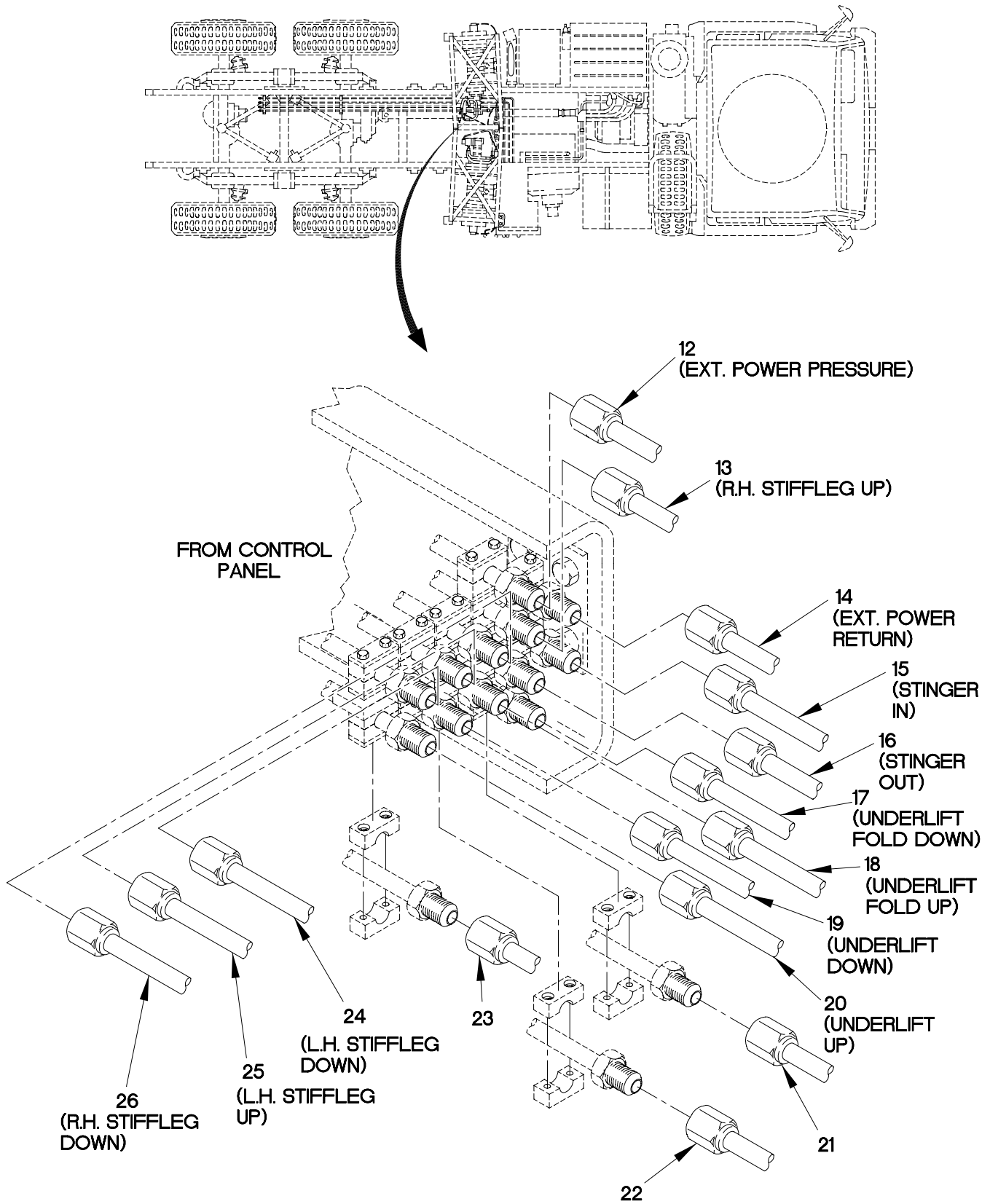
FIGURE 357. M1089 HYDRAULIC HOSES, TUBES AND FITTINGS (SHEET 3 OF 5)
