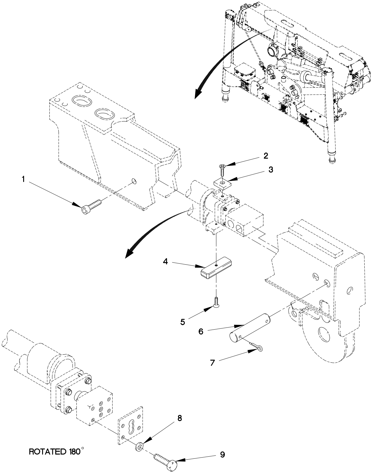
FIGURE 389. M1084 AND M1086 TELESCOPE CYLINDER ASSEMBLY (SHEET 1 OF 2)
