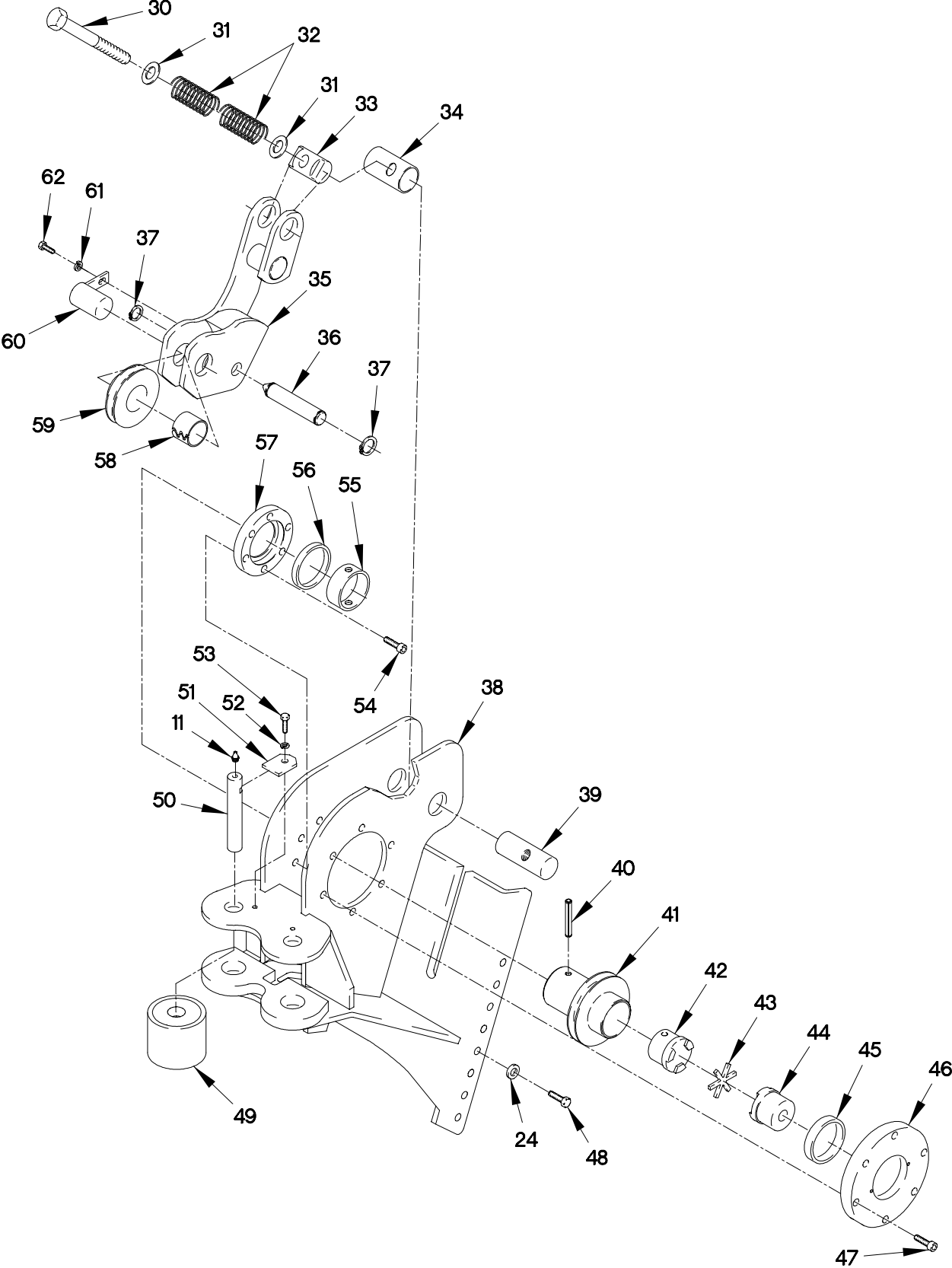
FIGURE 305. M1089 UNDERLIFT RIGHT AND LEFT STIFFLEG (SHEET 2 OF 2)
