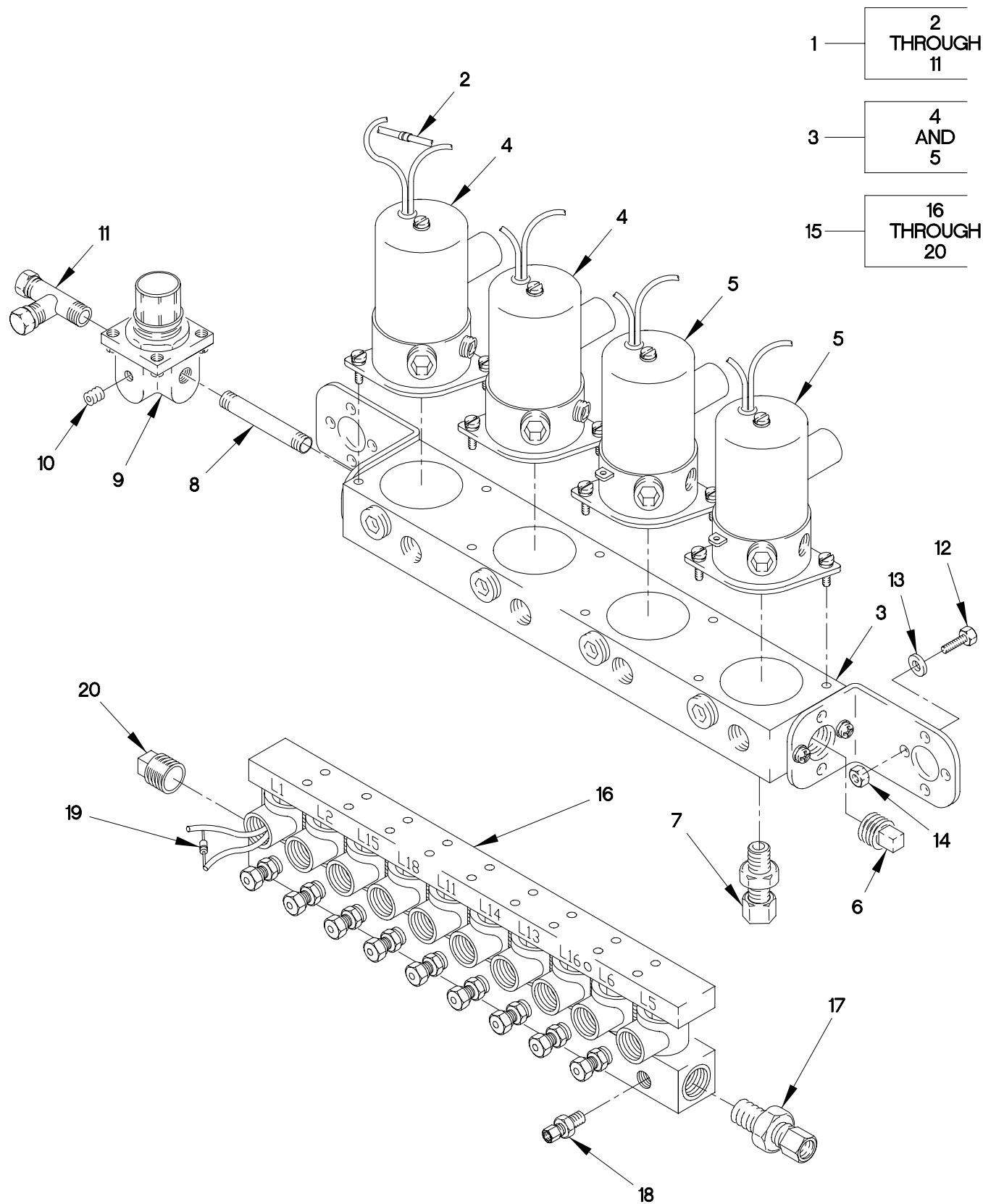
FIGURE 295. 30K WINCH PNEUMATIC AND VALVE MANIFOLD ASSEMBLIES
