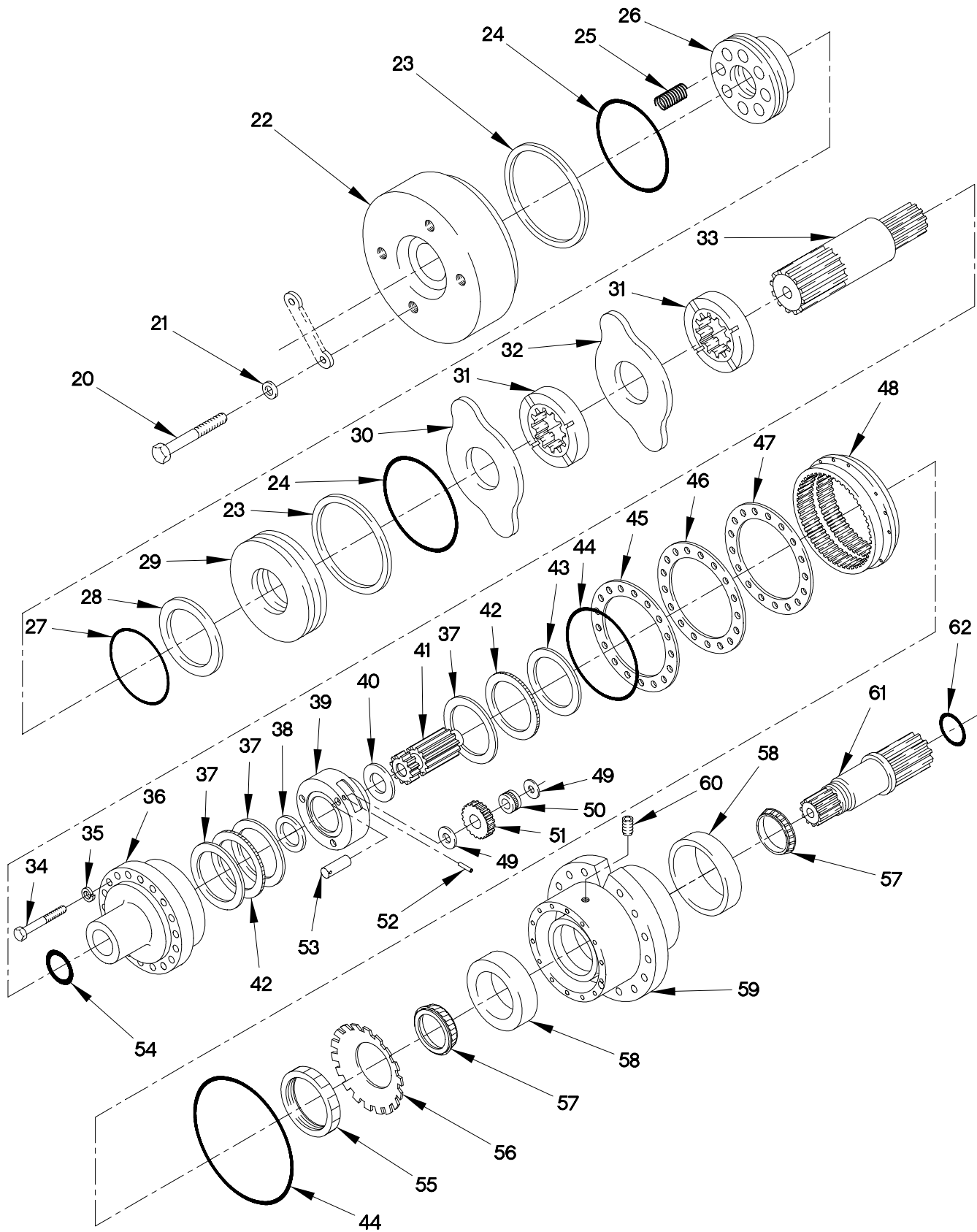
FIGURE 392. M1084 AND M1086 SWING DRIVE ASSEMBLY, HYDRAULIC MOTOR AND CROSS RELIEF VALVE (SHEET 2 OF 2)
