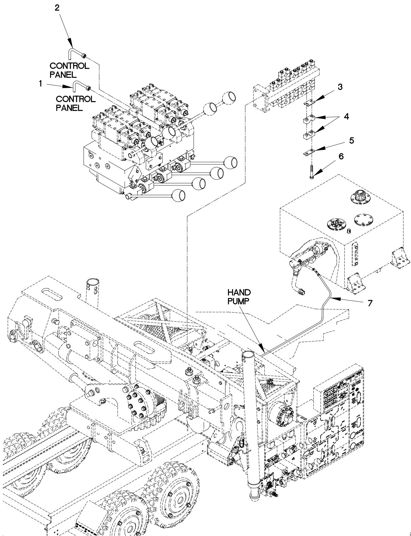
FIGURE 314. M1089 CRANE HYDRAULIC PRESSURE TUBES, HOSES AND CLAMPS
