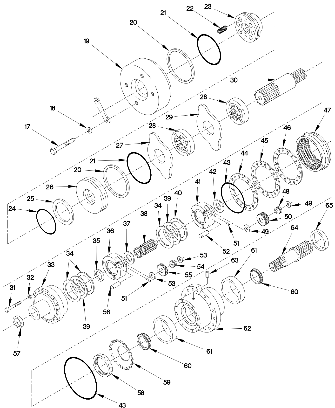
FIGURE 333. M1089 SWING DRIVE ASSEMBLY (SHEET 2 OF 2)
