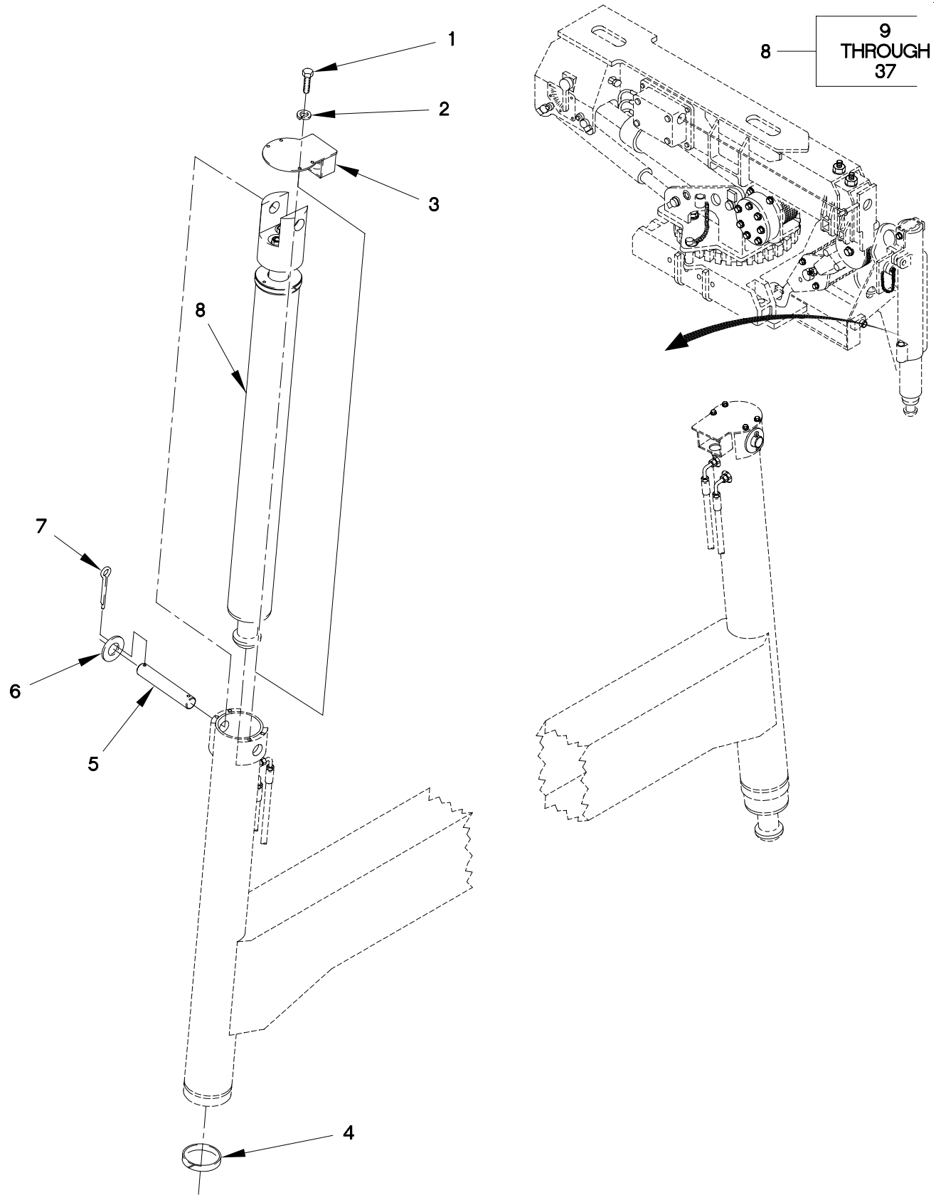
FIGURE 400. M1084 AND M1086 OUTRIGGER JACK CYLINDER ASSEMBLY (SHEET 1 OF 2)
