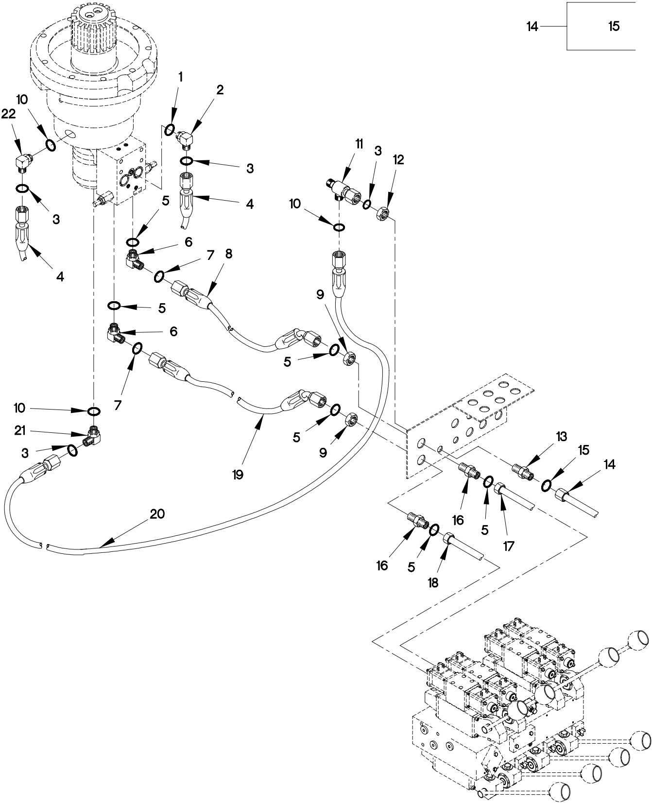
FIGURE 339. M1089 HUDRAULIC SWING HOSES AND FITTINGS
