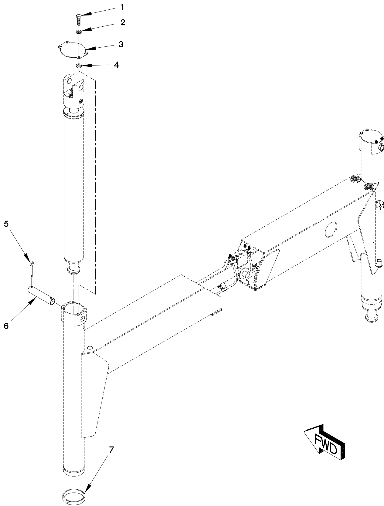
FIGURE 337. M1089 OUTRIGGER JACK CYLINDER (SHEET 1 OF 2)
