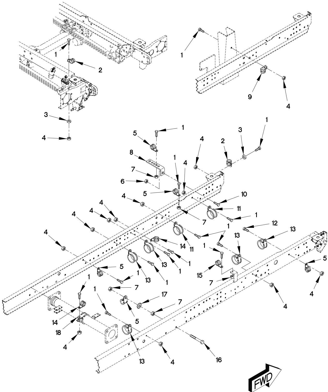
FIGURE 198. M1093 PNEUMATIC HOSE ROUTING LOOP CLAMPS AND BRACKETS (SHEET 1 OF 3)
