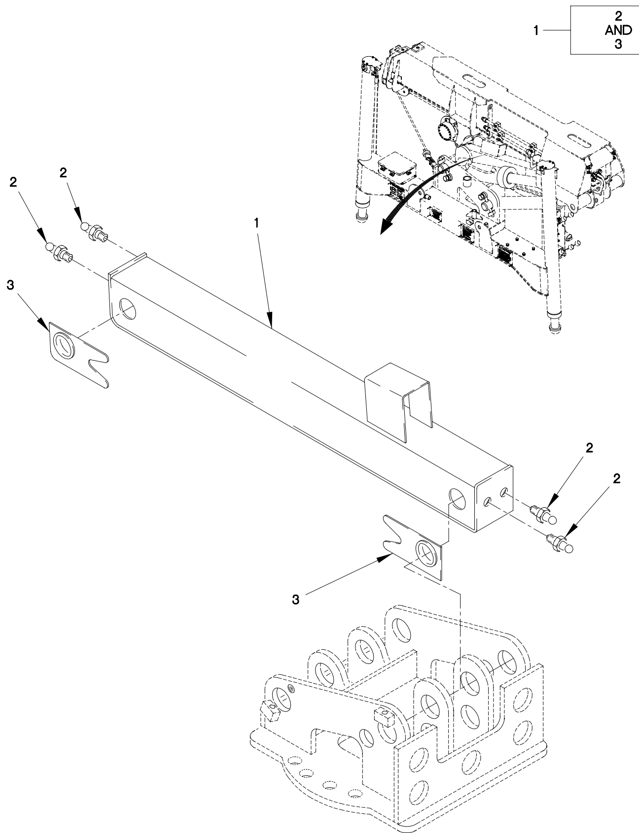
FIGURE 377. M1084 AND M1086 MAST ASSEMBLY
