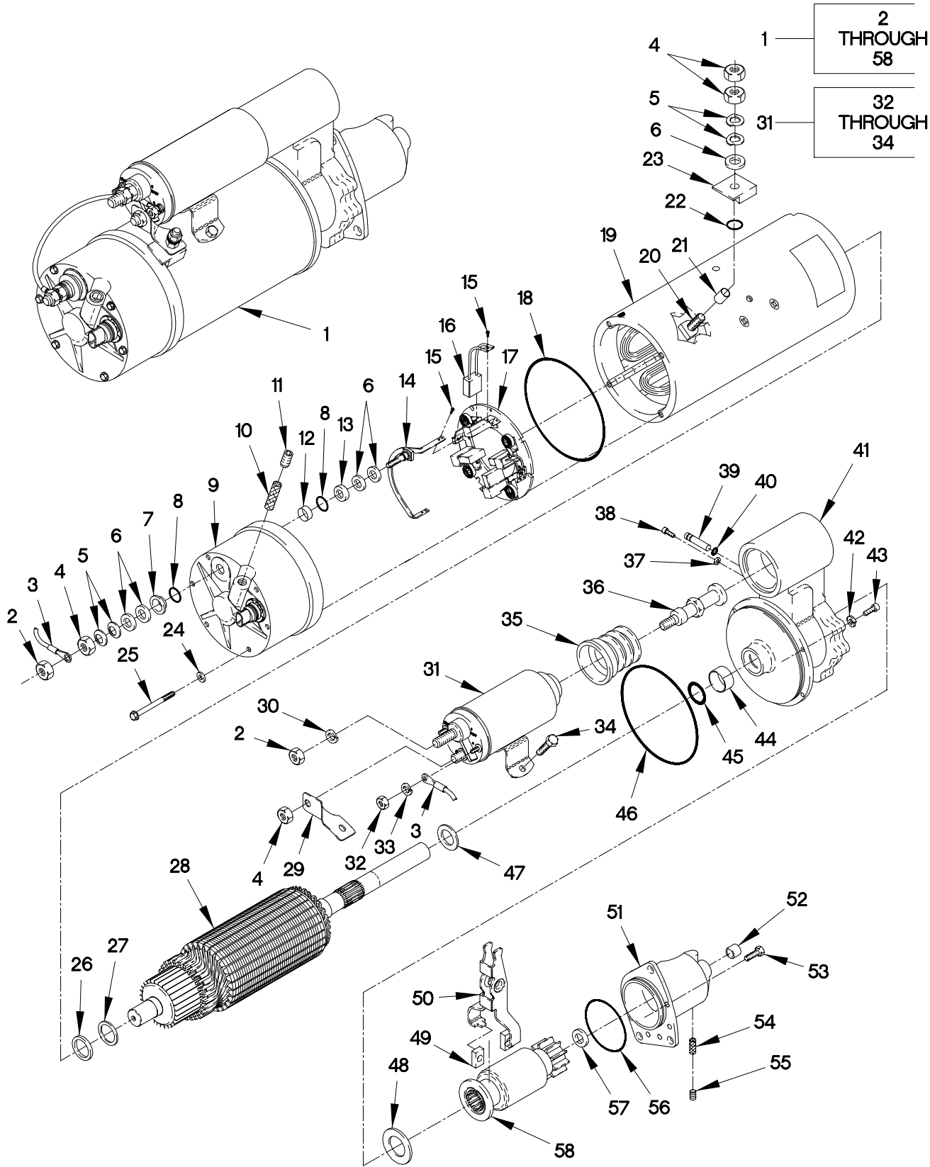
FIGURE 49. M0017705ME STARTER AND SOLENOID
