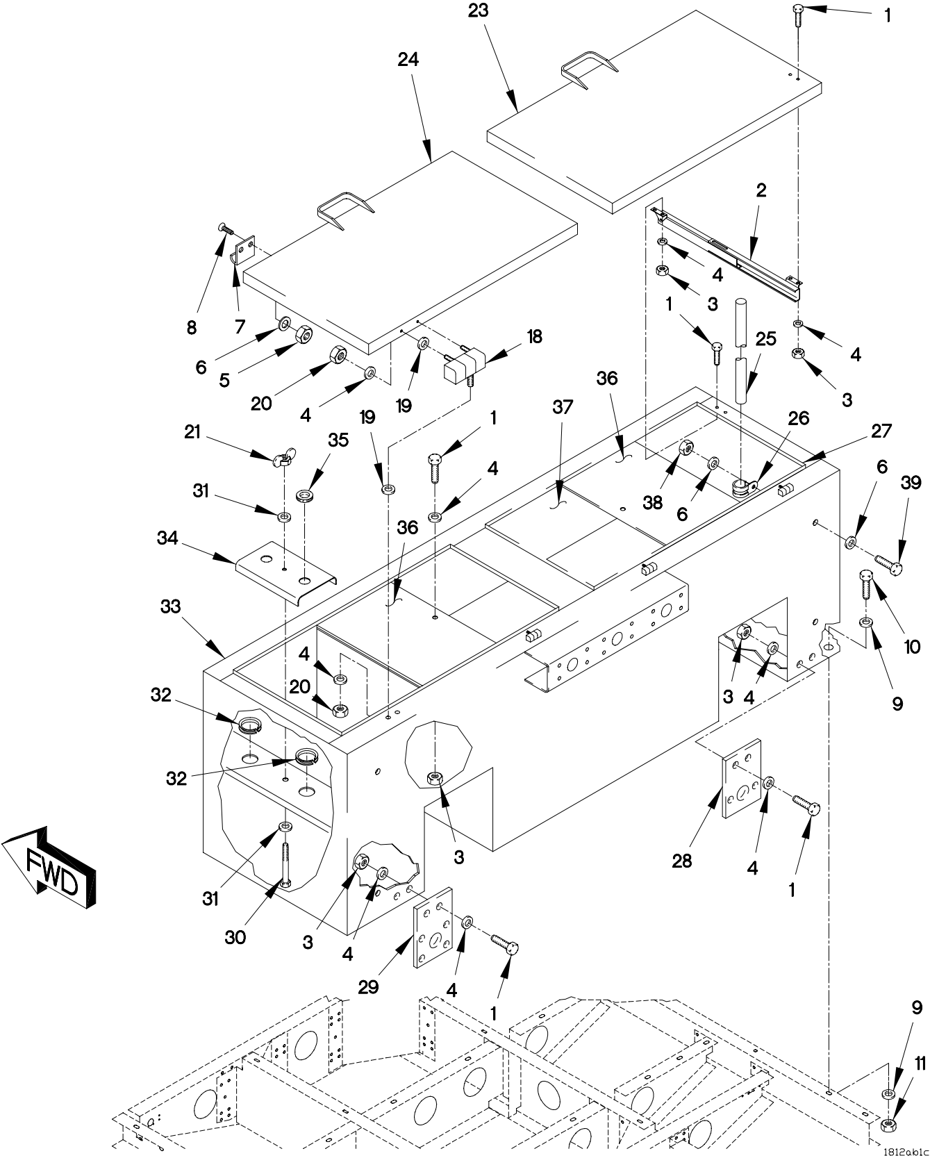
FIGURE 291. M1089 TOOL BOXES (SHEET 2 OF 2)
