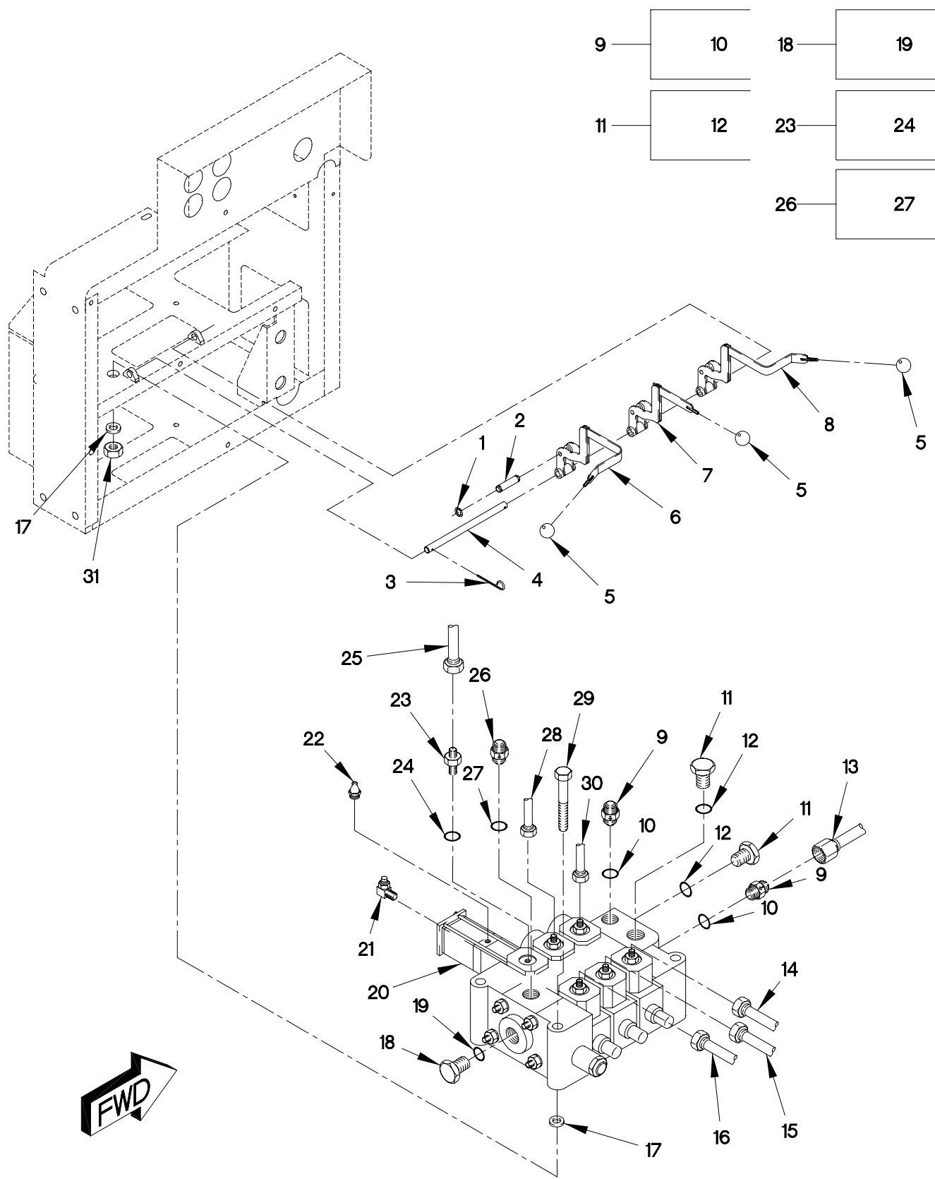
FIGURE 361. M1089 UPPER CONTROL VALVE ASSEMBLY AND HANDLES
