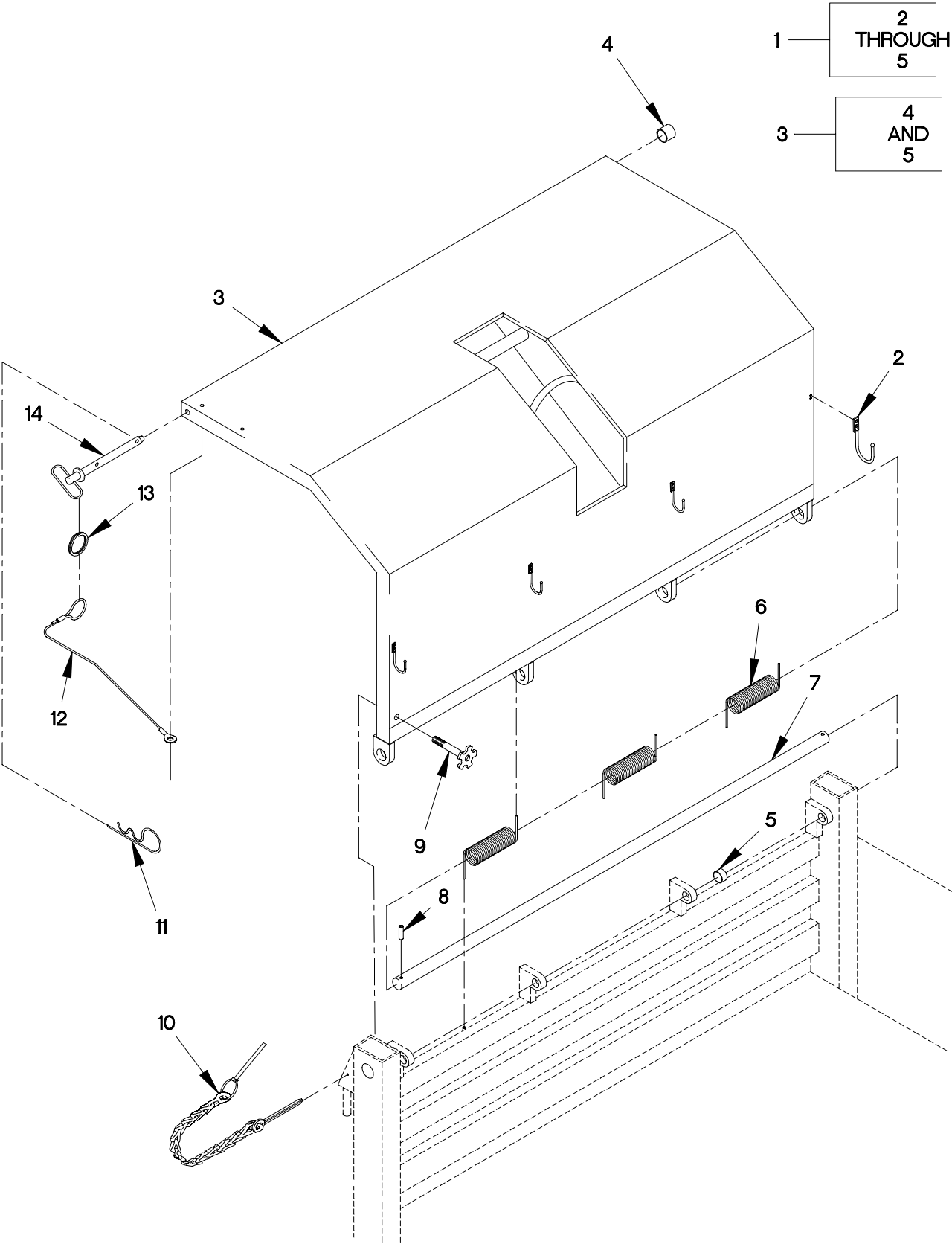
FIGURE 418. M1090 AND M1094 CAB PROTECTOR ASSEMBLY
