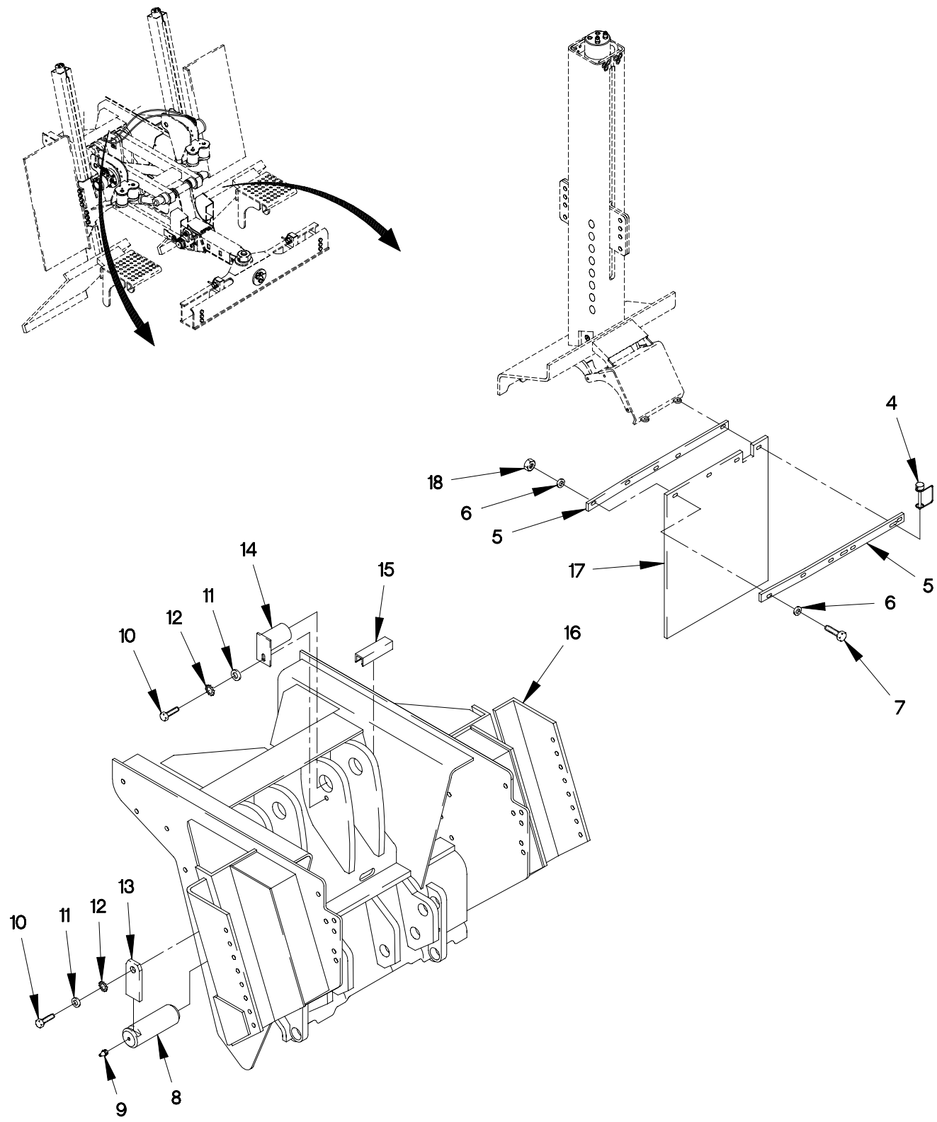
FIGURE 301. M1089 UNDERLIFT ASSEMBLY AND SPLASH GUARDS (SHEET 2 OF 2)
