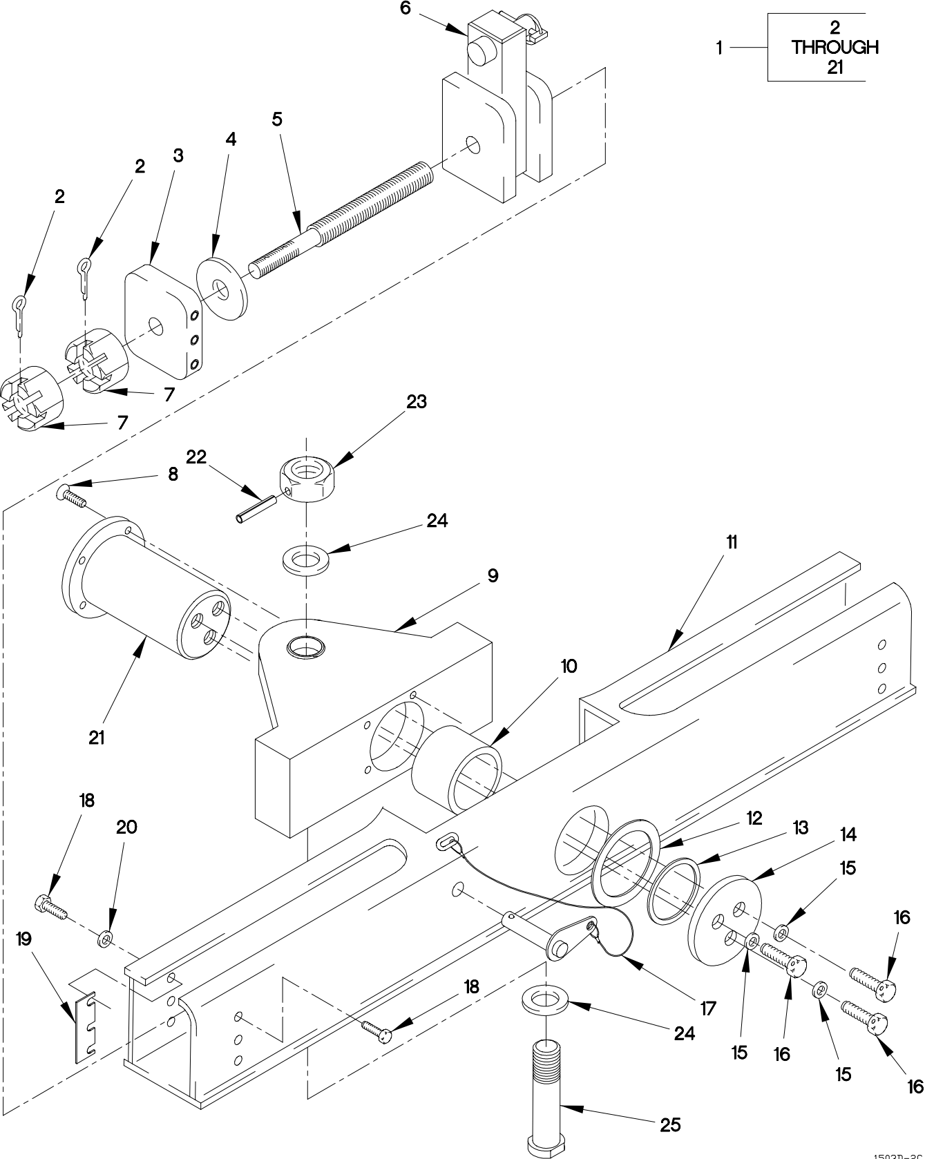
FIGURE 302. M1089 UNDERLIFT CROSSBAR ASSEMBLY AND FRONT TOWING ADAPTER (SHEET 1 OF 2)
