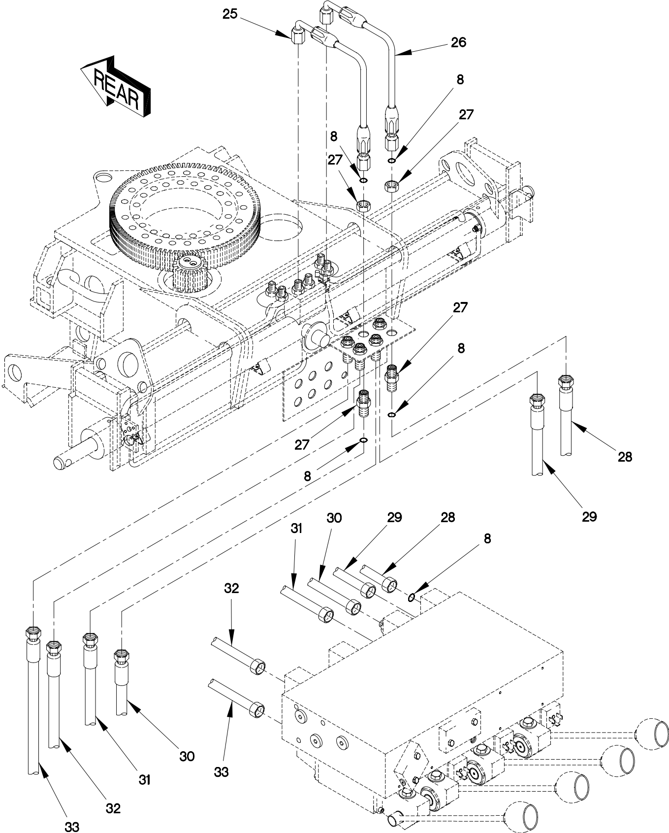
FIGURE 335. M1089 OUTRIGGER BEAM, HOSES AND FITTINGS (SHEET 3 OF 3)
