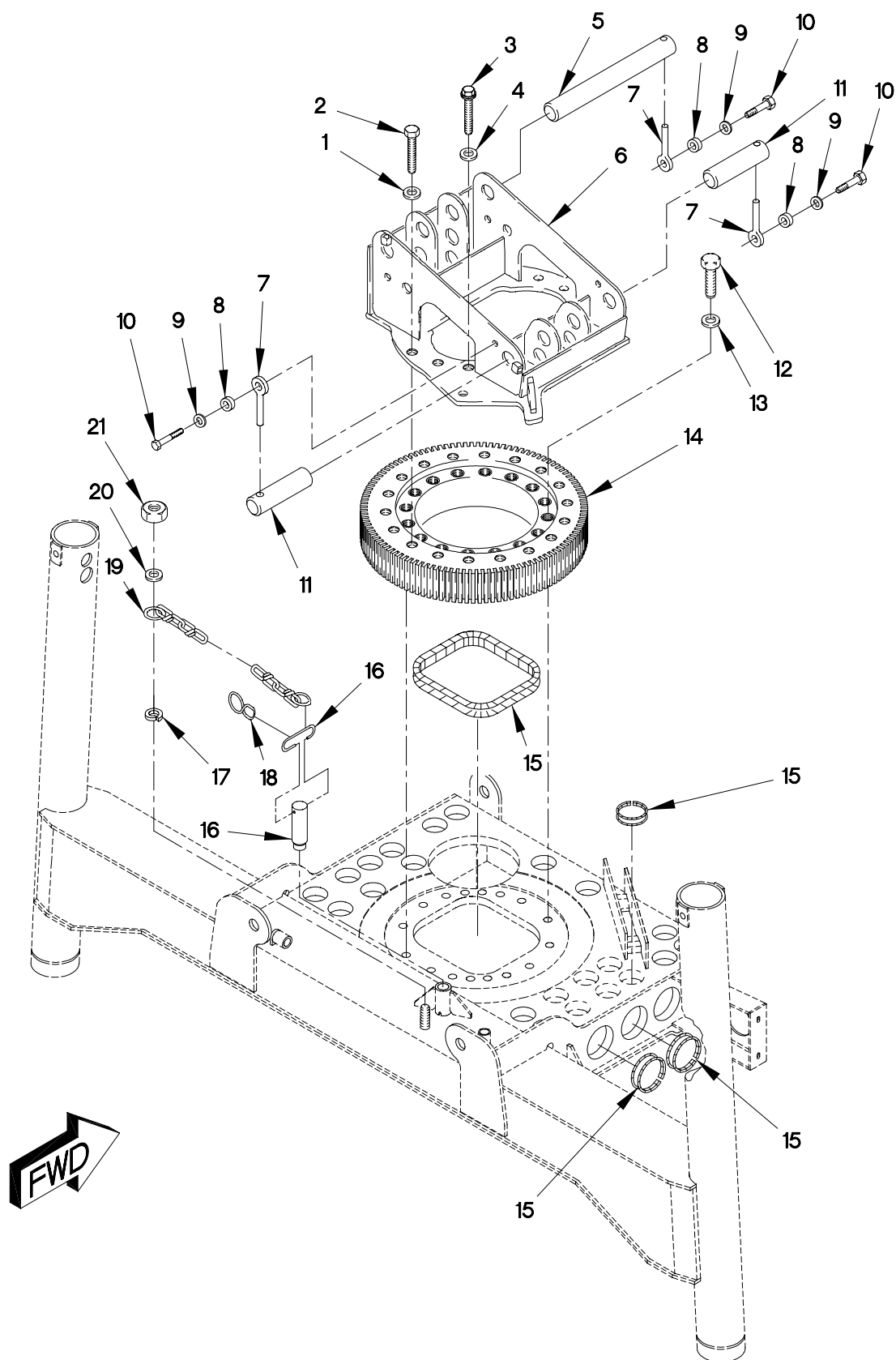
FIGURE 391. M1084 AND M1086 TURNTABLE, LOCK PIN AND CYLINDER MOUNT PINS
