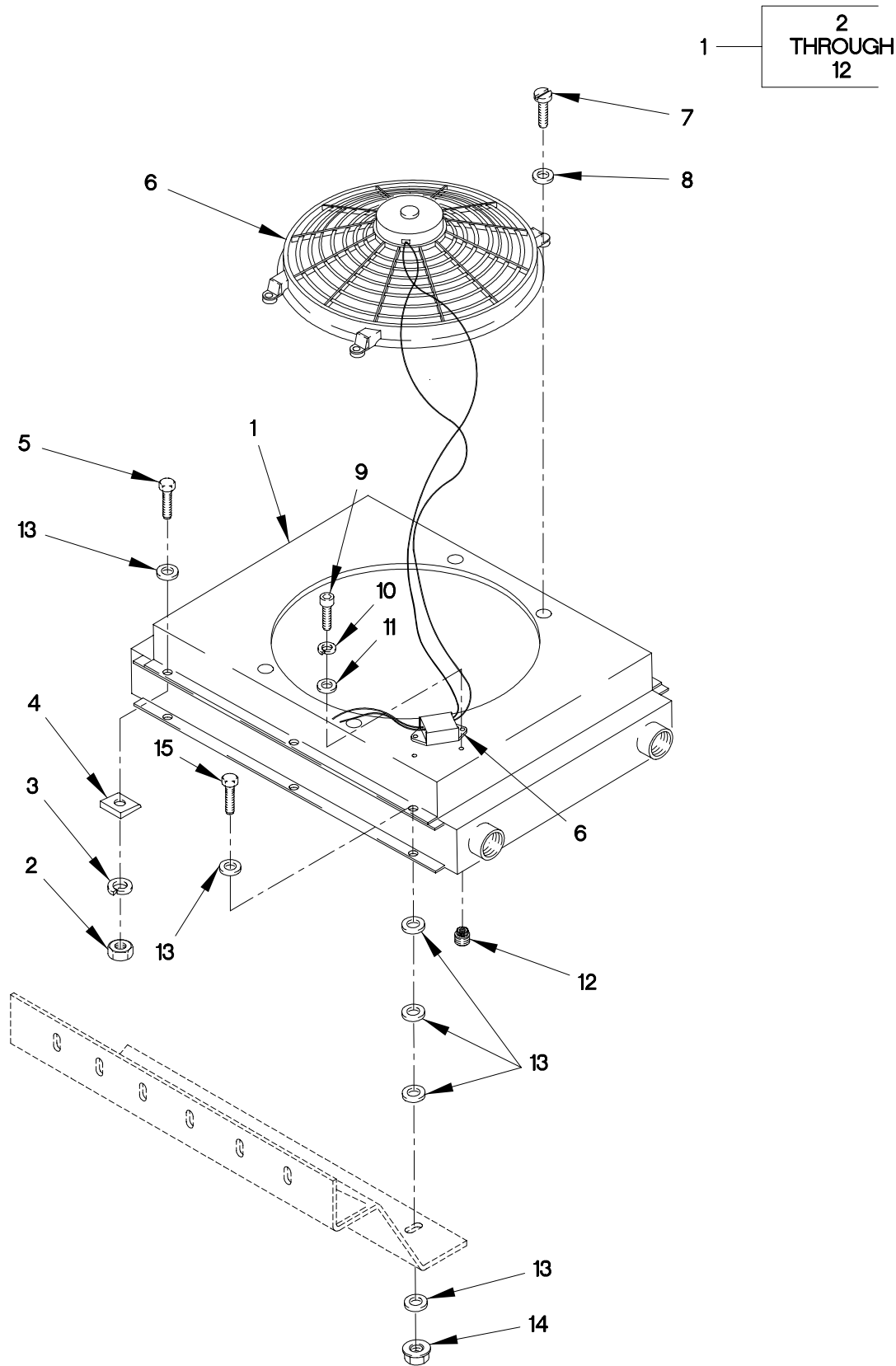
FIGURE 149. M1083, M1084, M1085, M1086, M1090 AND M1094 TRANSMISSION AUXILLIARY OIL COOLER
