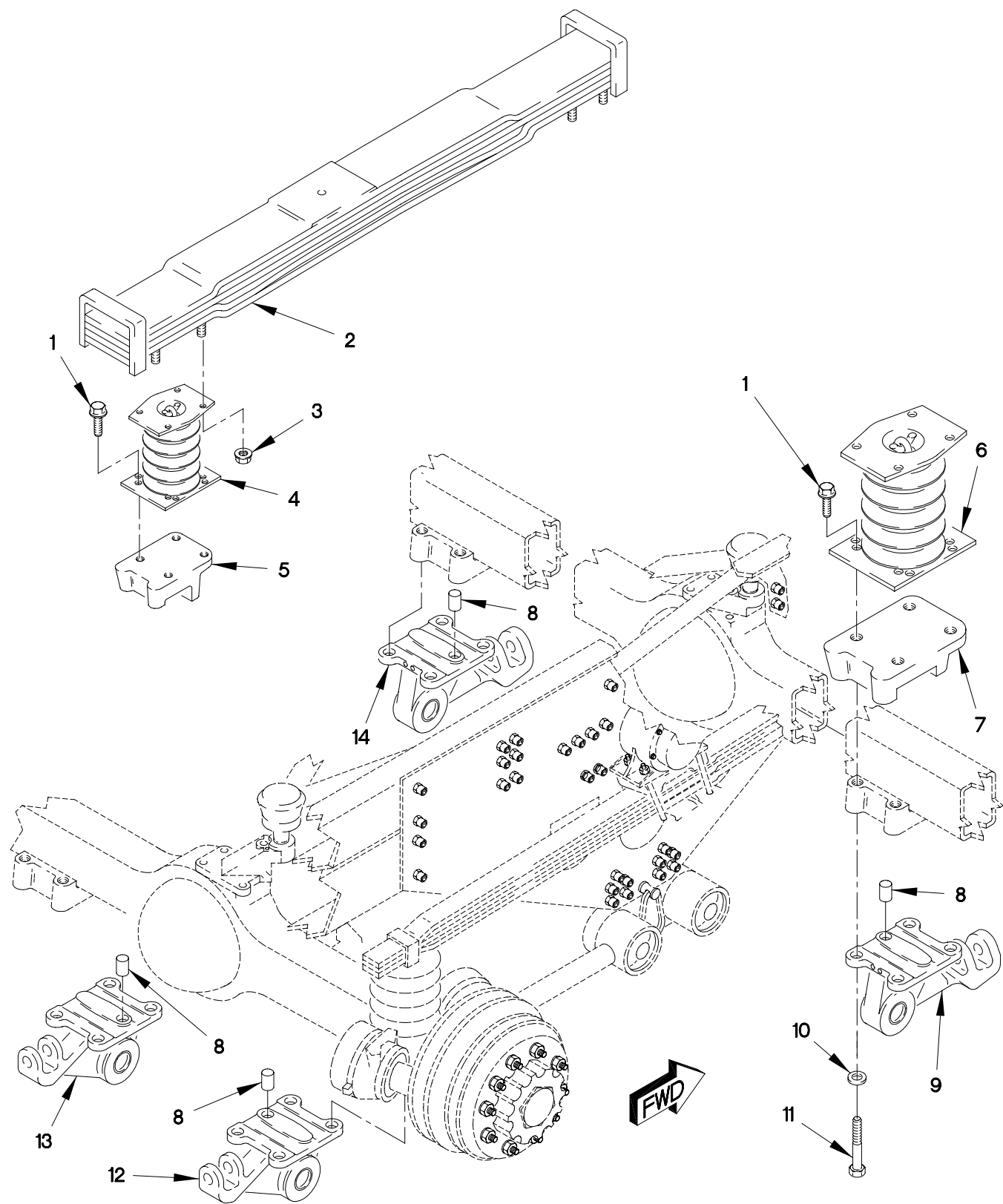
FIGURE 240. REAR LEAF SPRING SUSPENSION AND TORQUE RODS (SHEET 1 OF 3)
