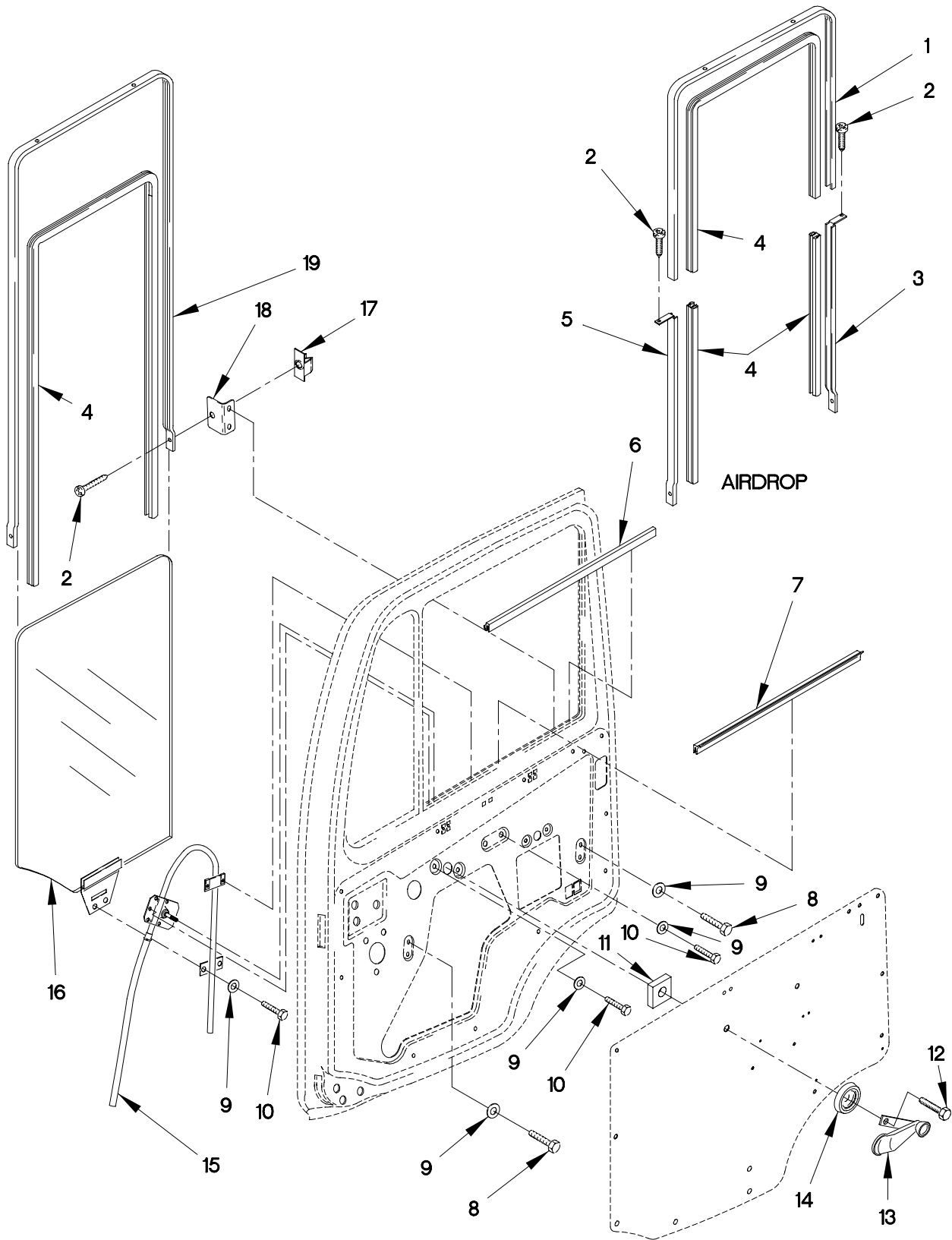
FIGURE 258. CAB DOOR WINDOWS AND FITTINGS
