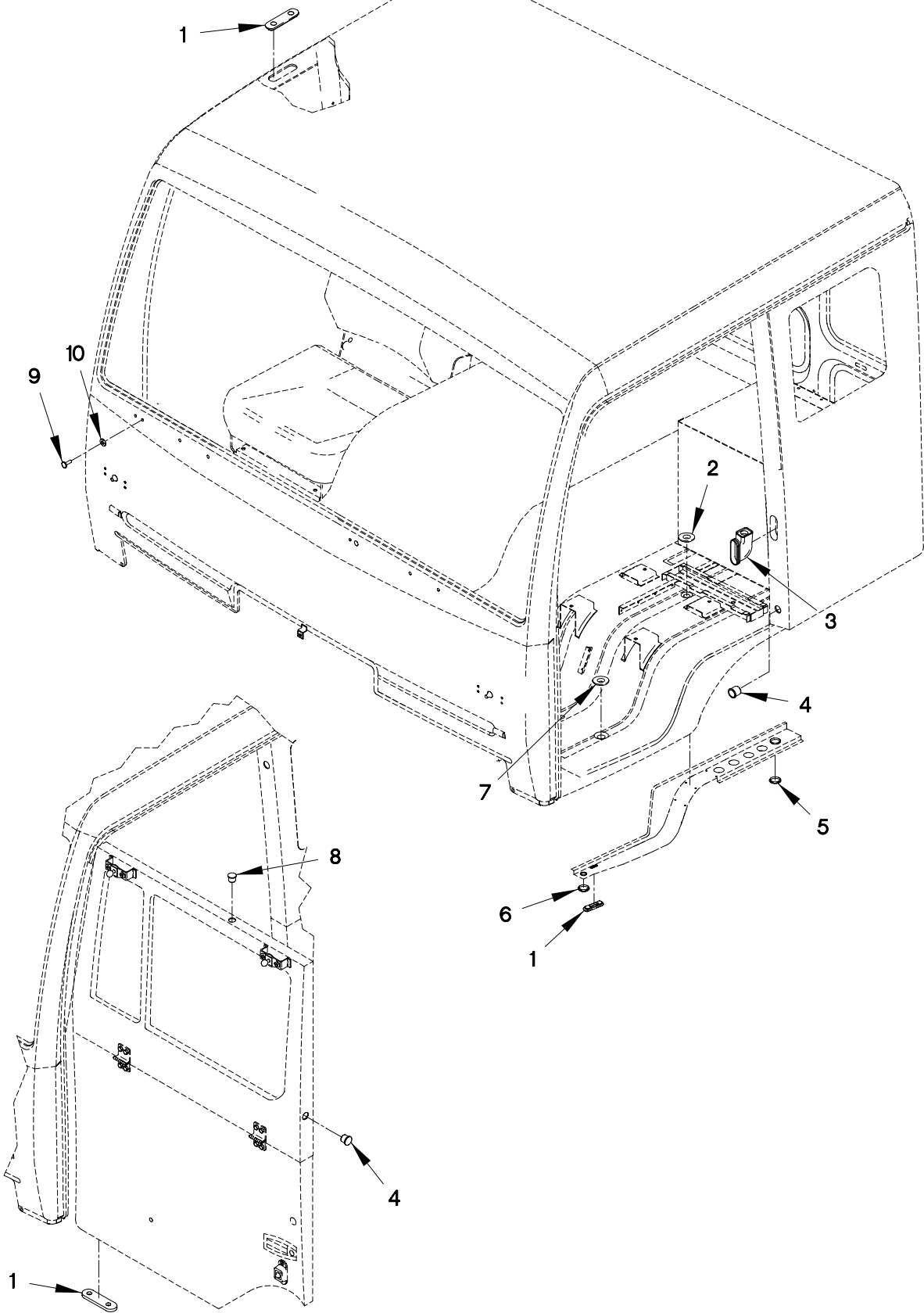
FIGURE 266. CAB DRAIN PLUGS
