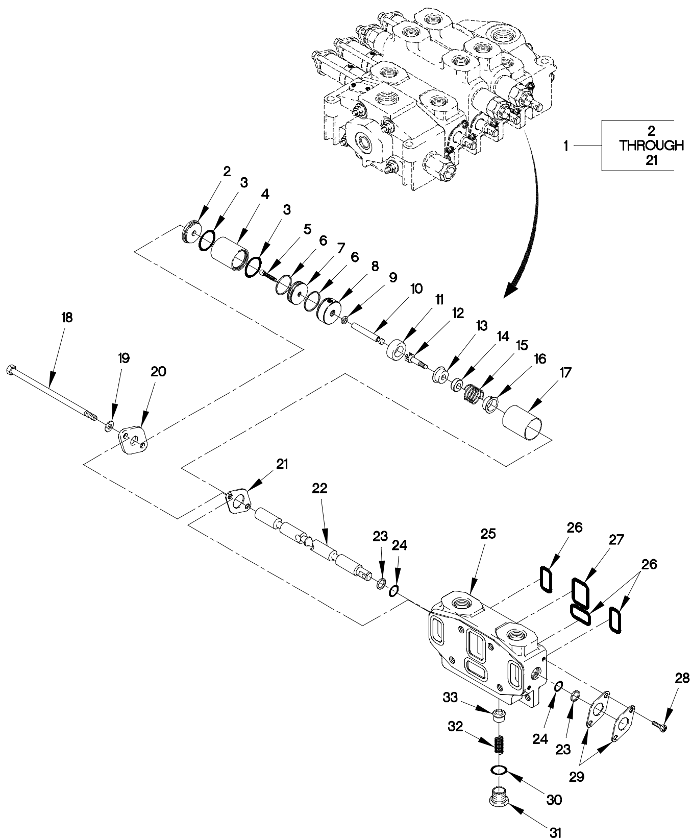
FIGURE 370. M1089 UNDERLIFT STINGER POSITION CONTROL VALVE
