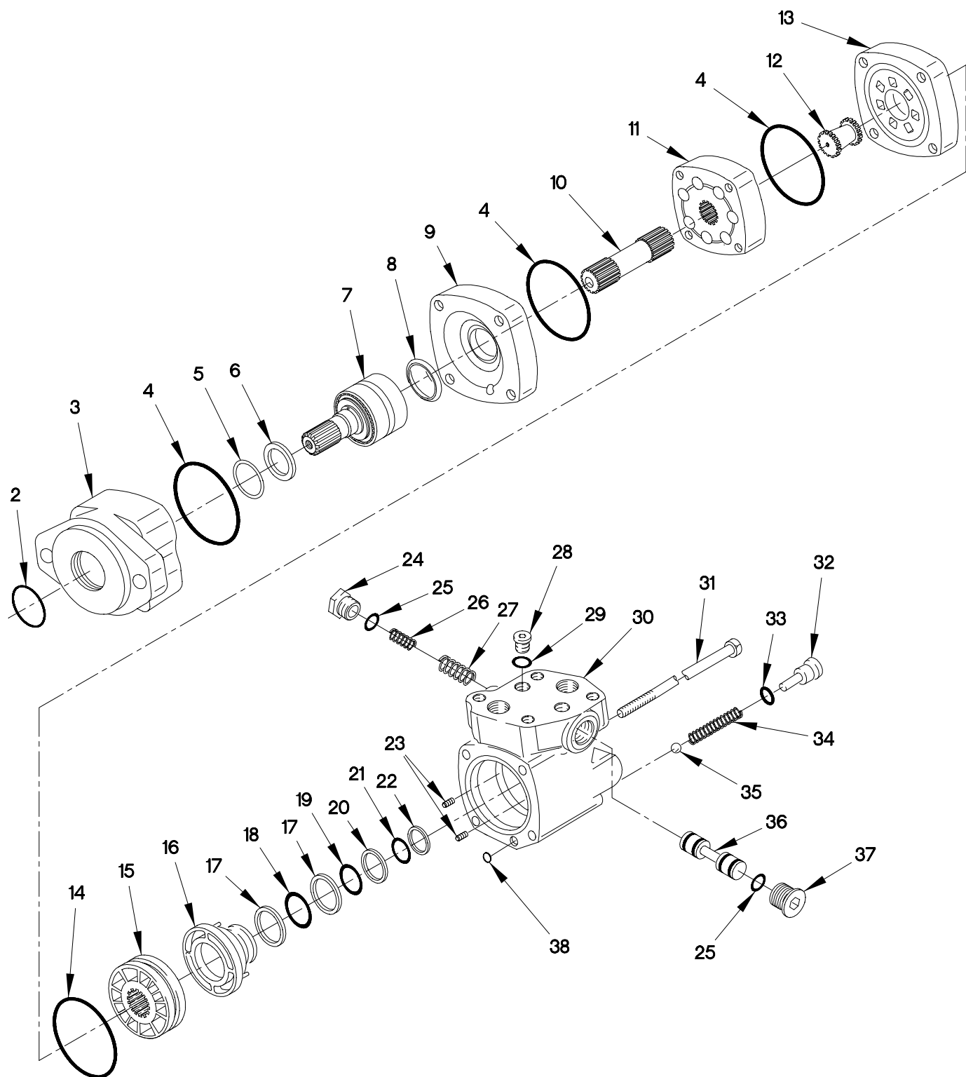
FIGURE 297. 30K WINCH HYDRAULIC MOTOR (SHEET 1 OF 2)
