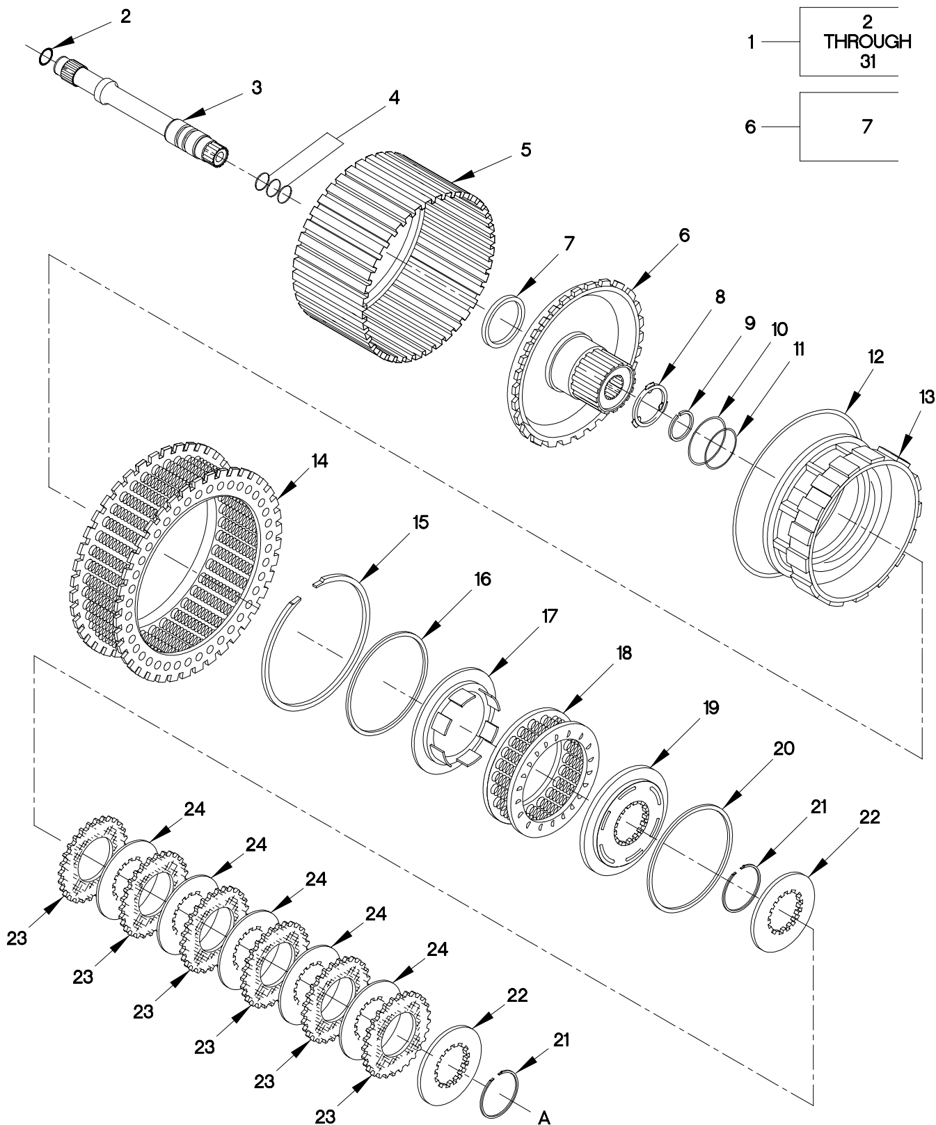
FIGURE 144. ROTATING CLUTCH MODULE (SHEET 1 OF 2)
