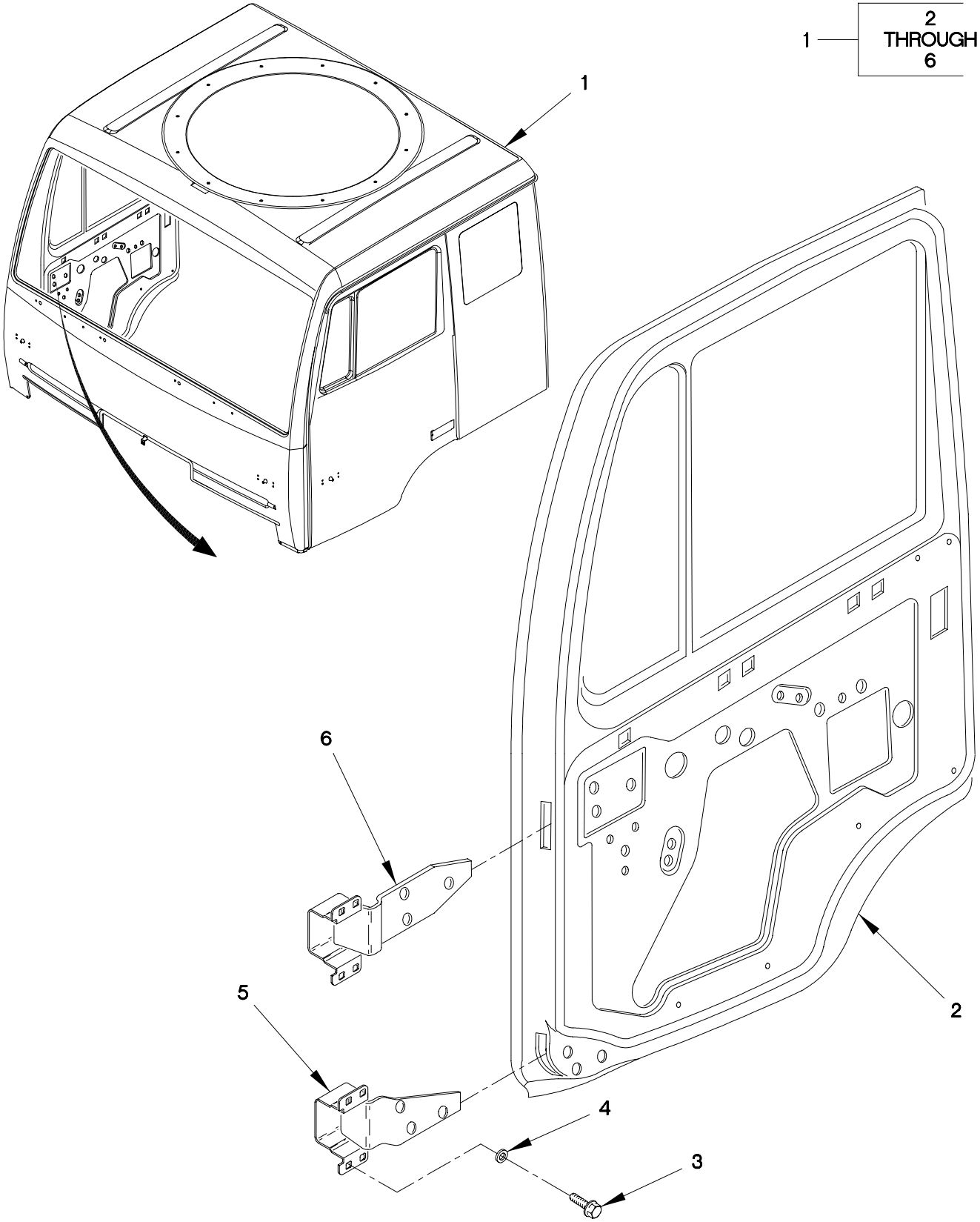
FIGURE 245. STANDARD CAB ASSEMBLY, DOORS AND HINGES
