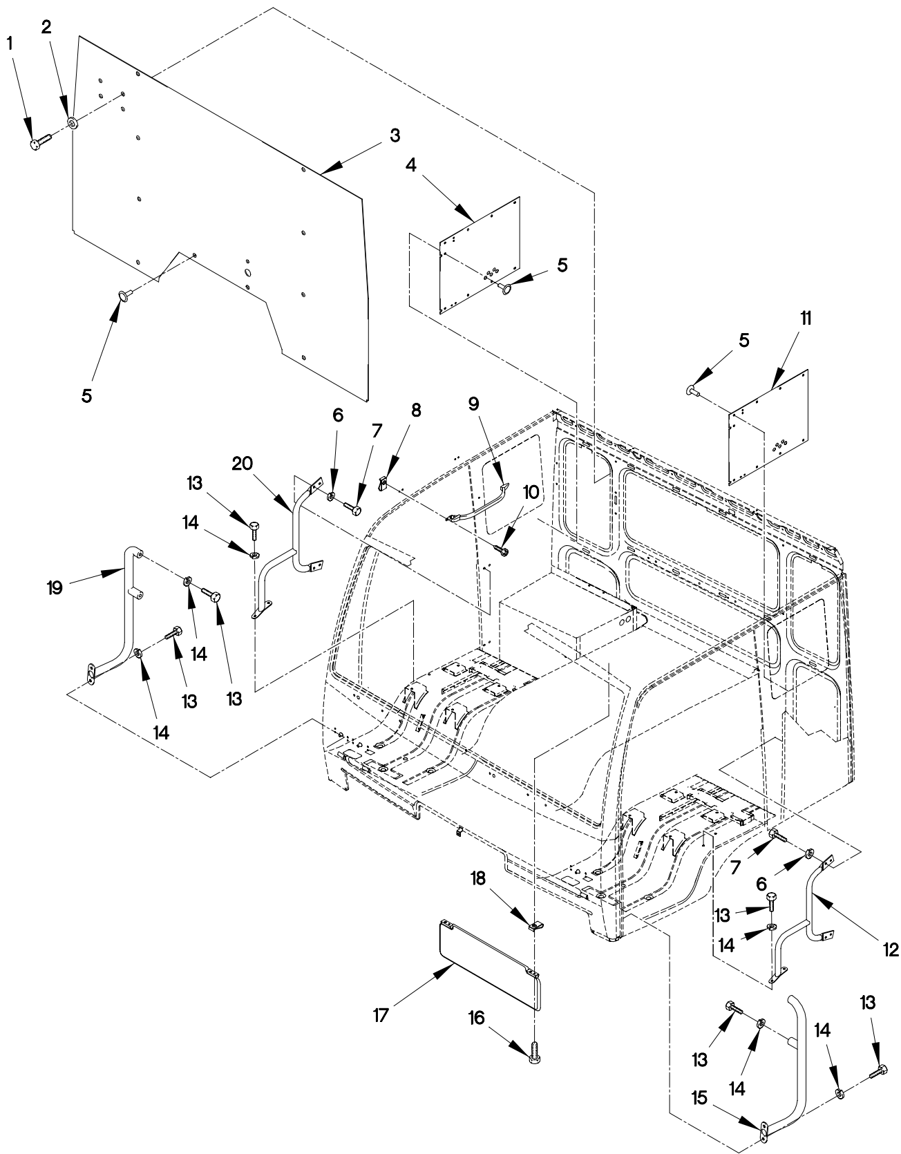
FIGURE 268. STANDARD CAB LINERS, BOARDING HANDLES AND SUN VISORS
