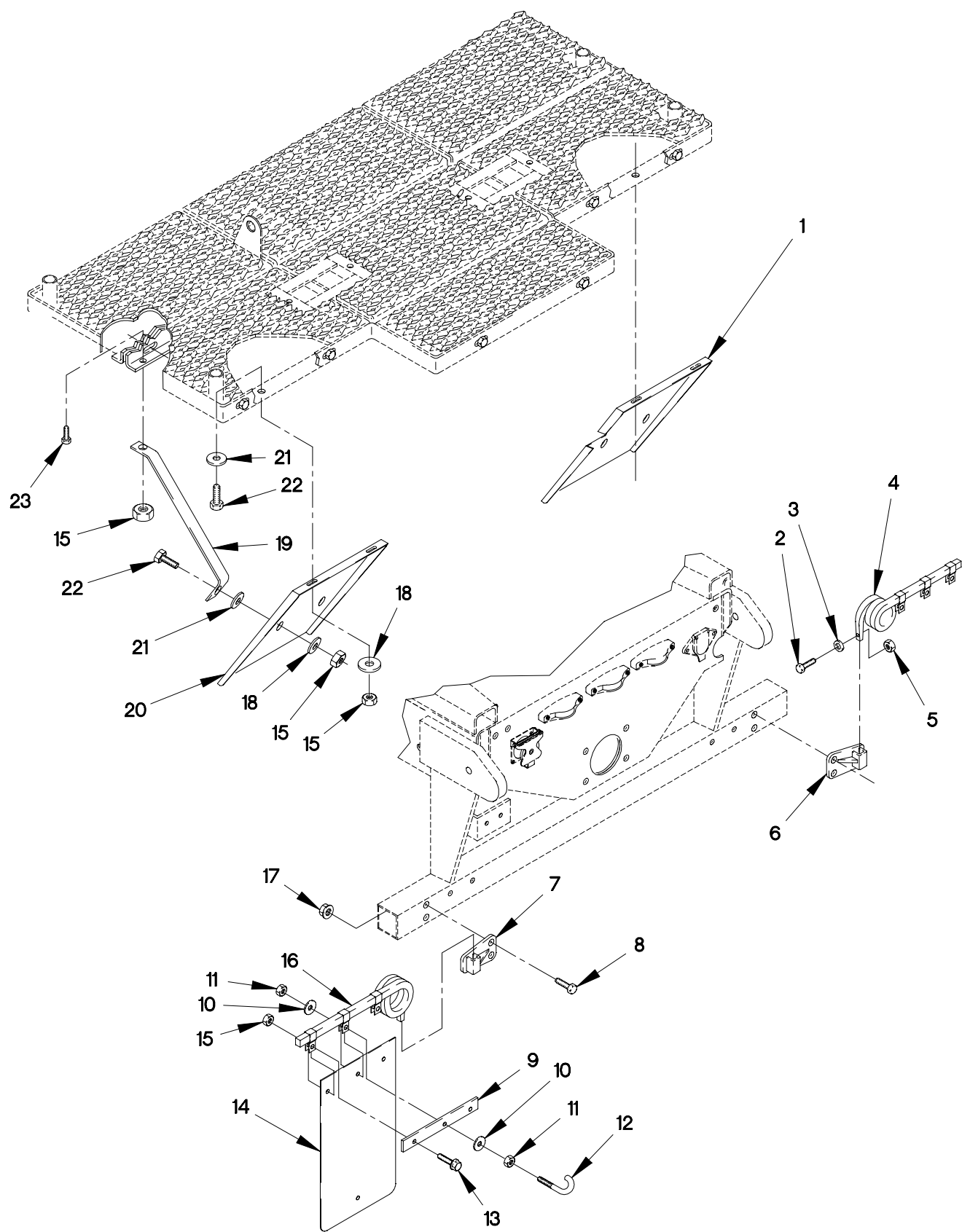
FIGURE 263. M1088 REAR FENDERS AND SPLASH GUARDS
