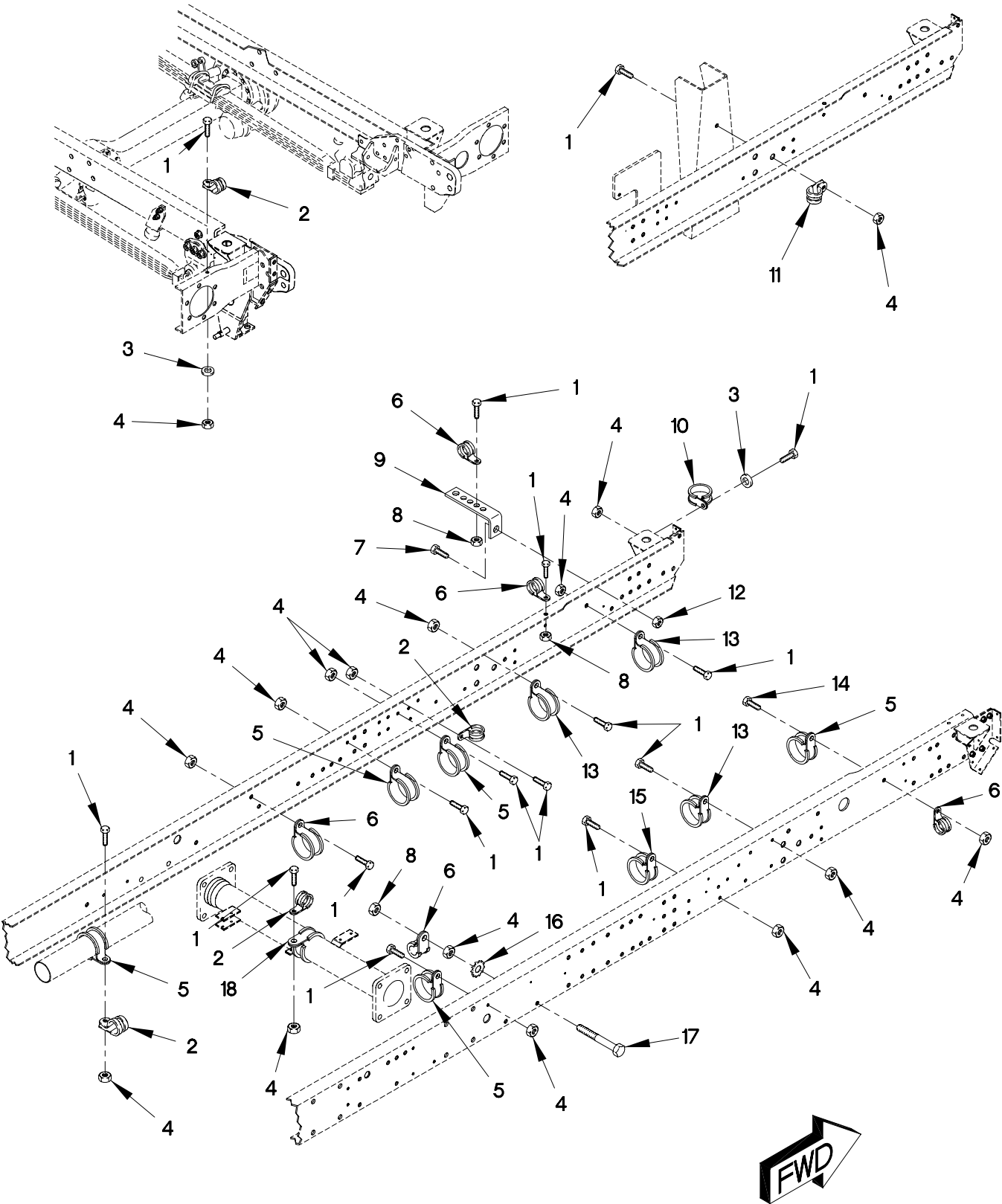
FIGURE 192. M1086 PNEUMATIC HOSE ROUTING LOOP CLAMPS AND BRACKETS (SHEET 1 OF 3)
