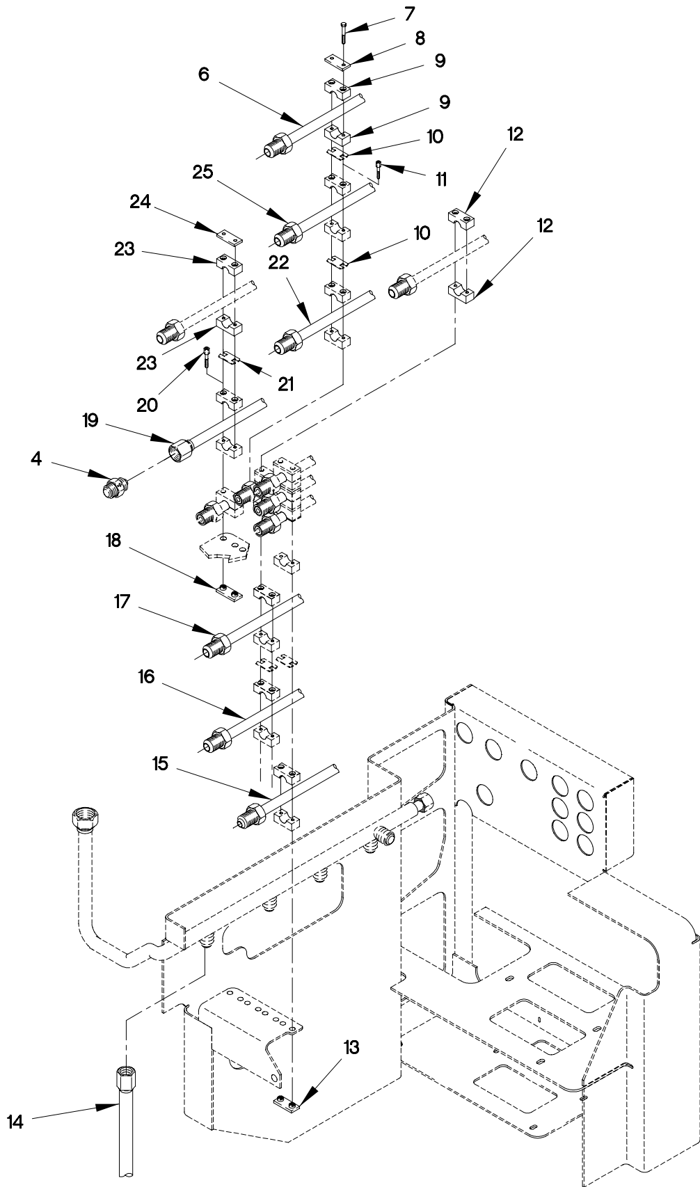
FIGURE 371. M1089 LOWER CONTROL VALVE TUBES, HOSES AND CLAMPS (SHEET 2 OF 2)
